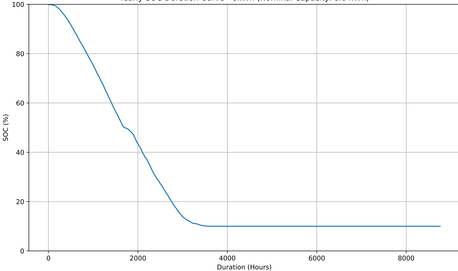
Yearly SOC Duration Curve - 8kWh (Nominal Capacity: 8.0 kWh)
