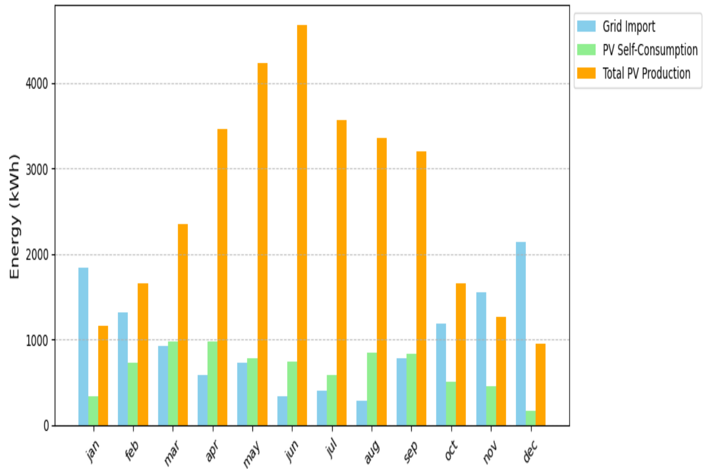
Grid and PV Interaction
