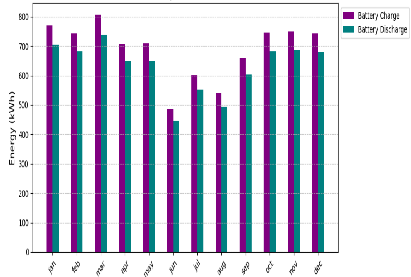
Battery Performance
