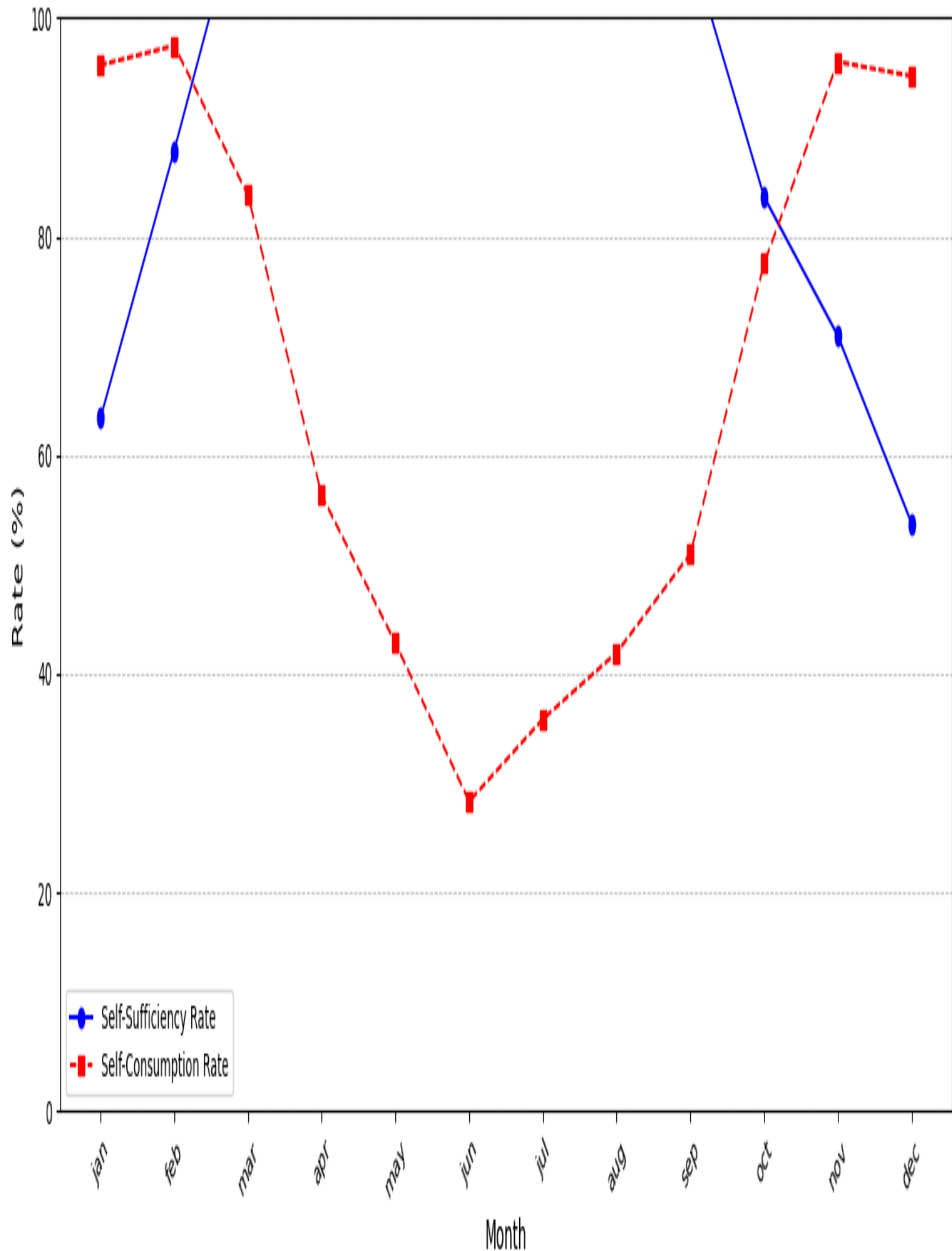
Scenario: 50kWh - Performance Rates
