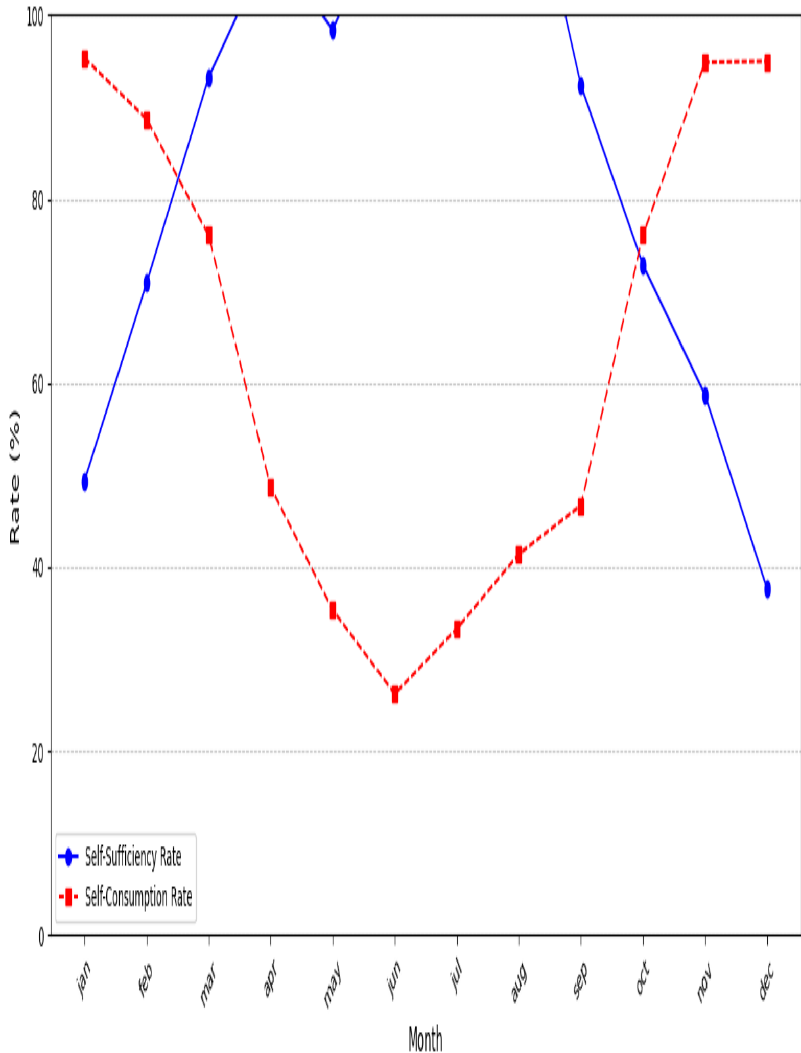
Scenario: 26kWh - Performance Rates
