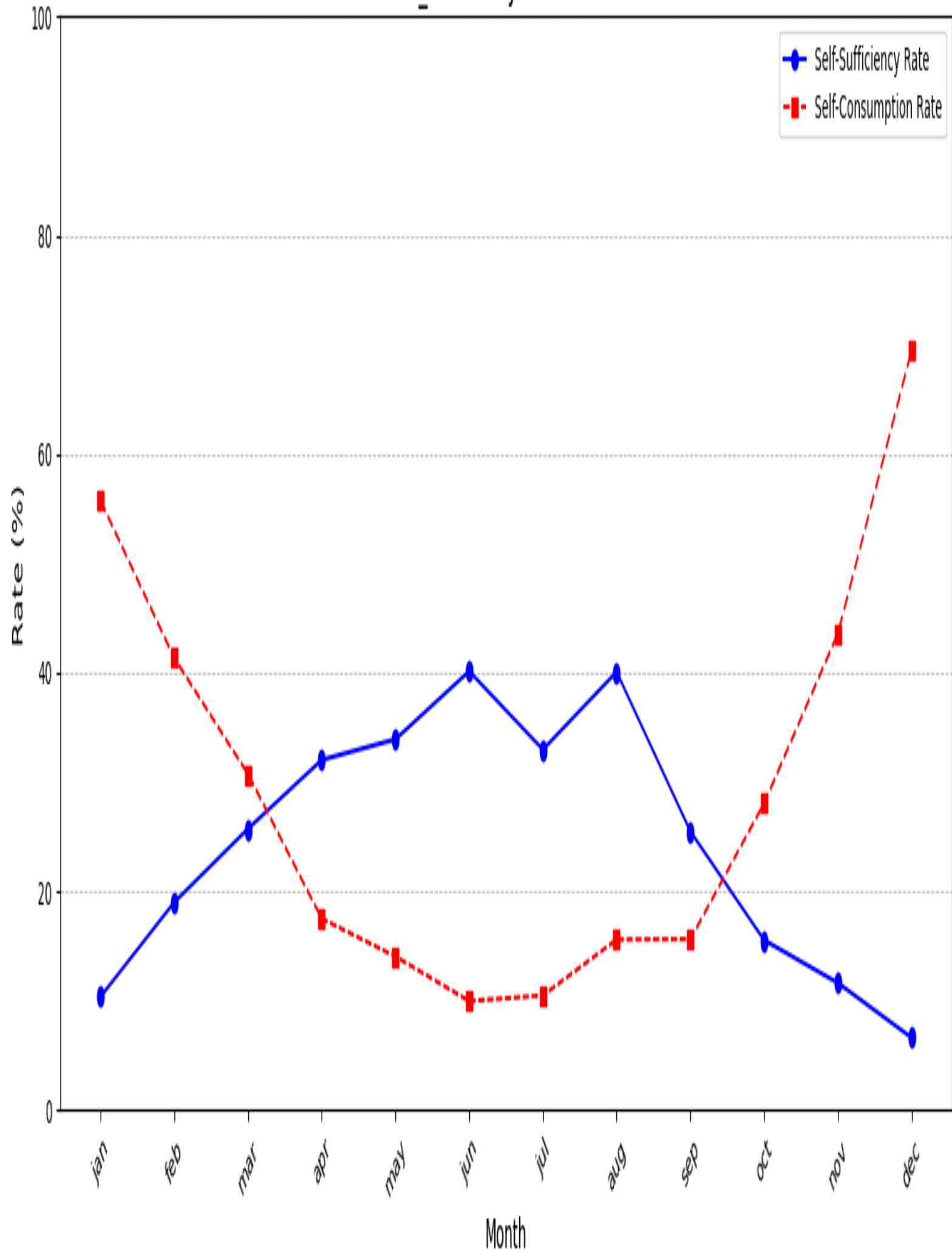
Scenario: PV_NoBattery - Performance Rates
