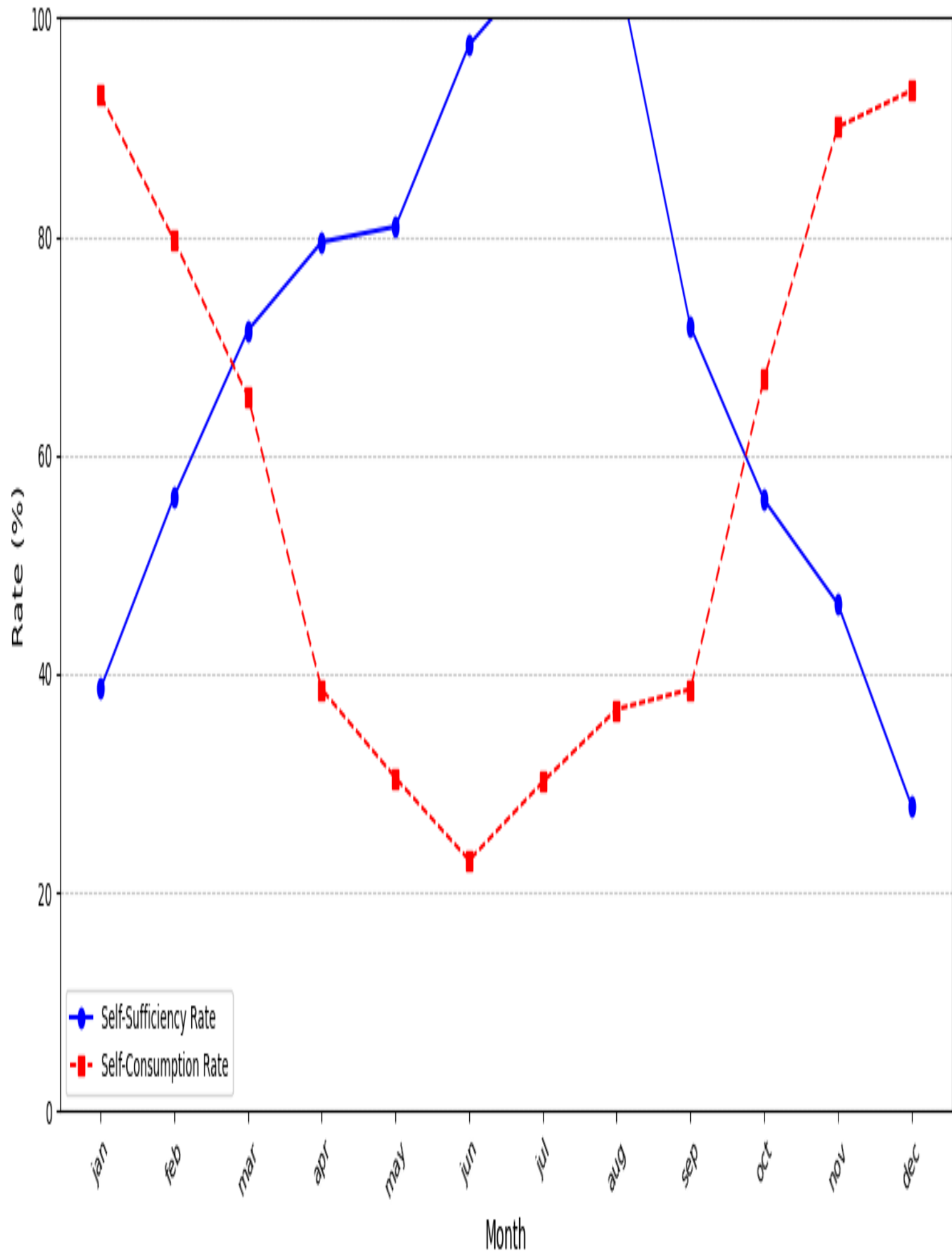
Scenario: 15kWh - Performance Rates
