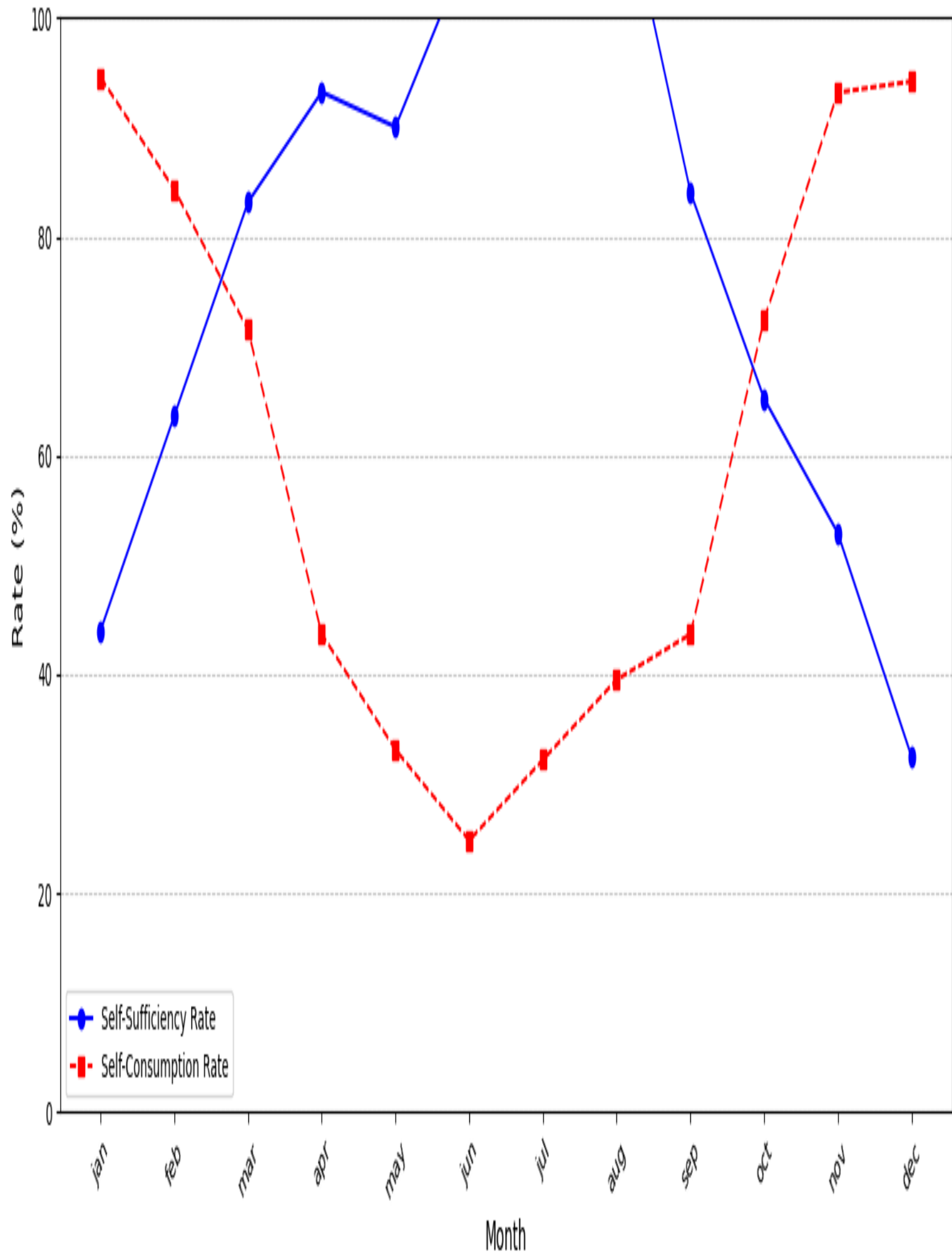
Scenario: 20kWh - Performance Rates
