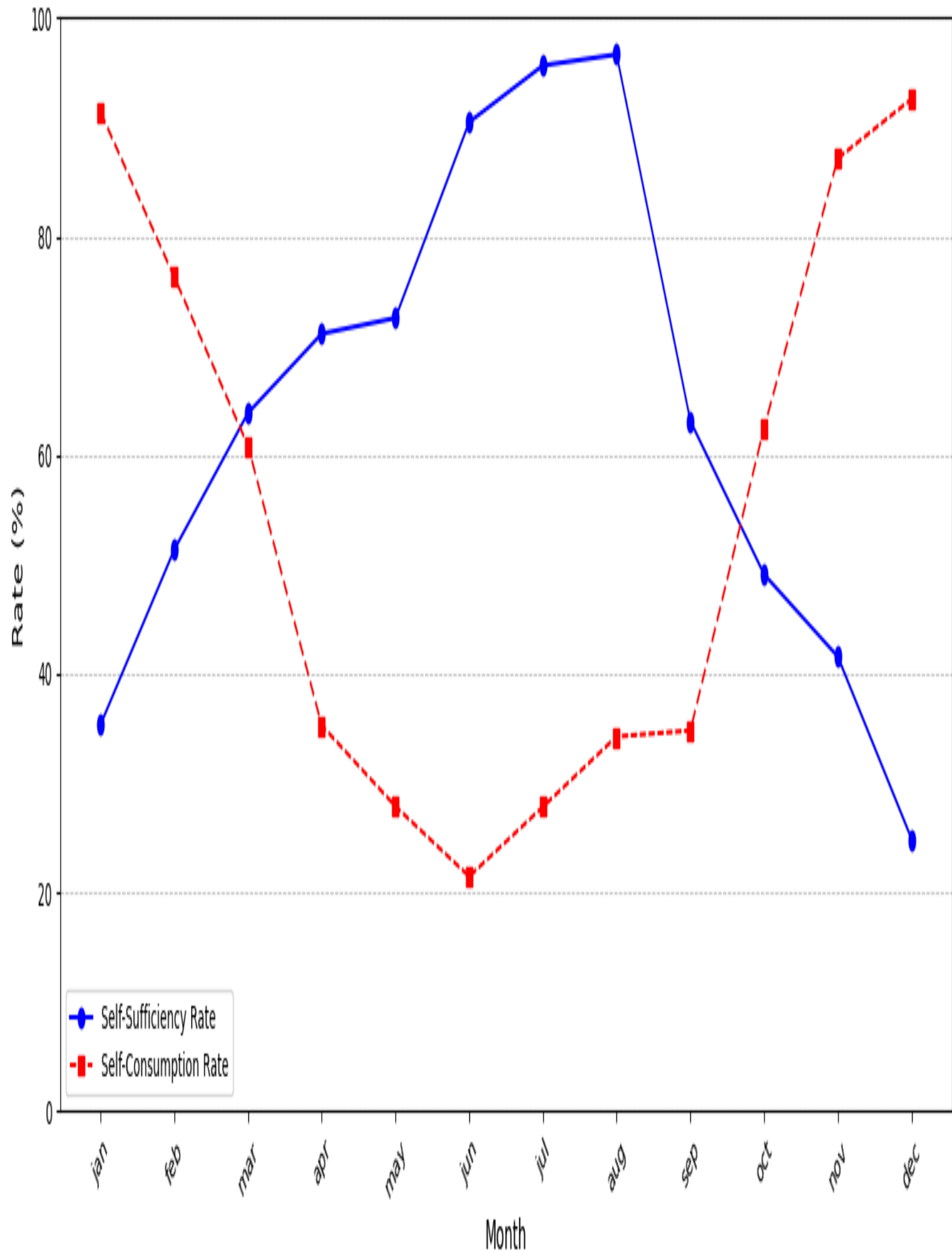
Scenario: 12kWh - Performance Rates
