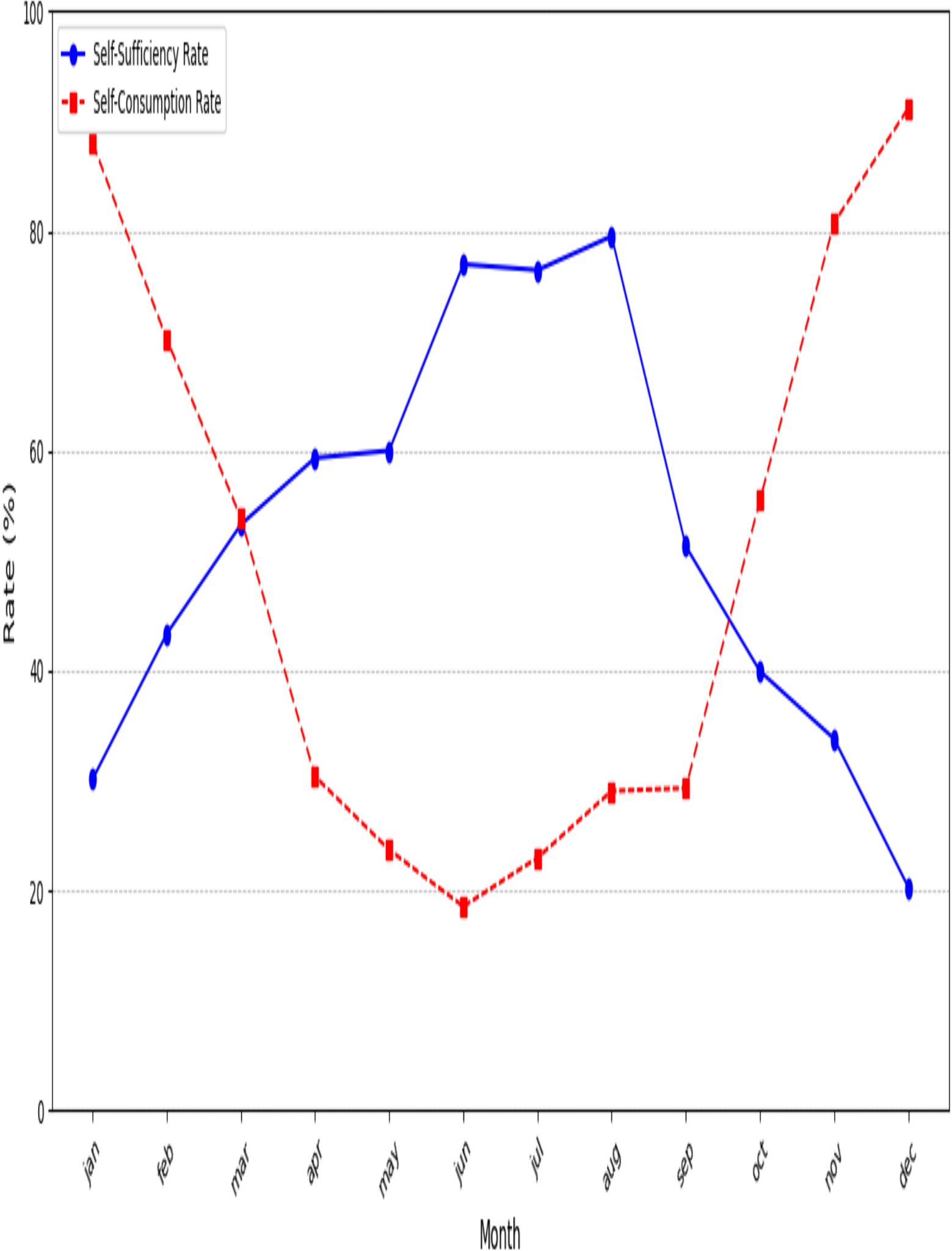
Scenario: 8kWh - Performance Rates
