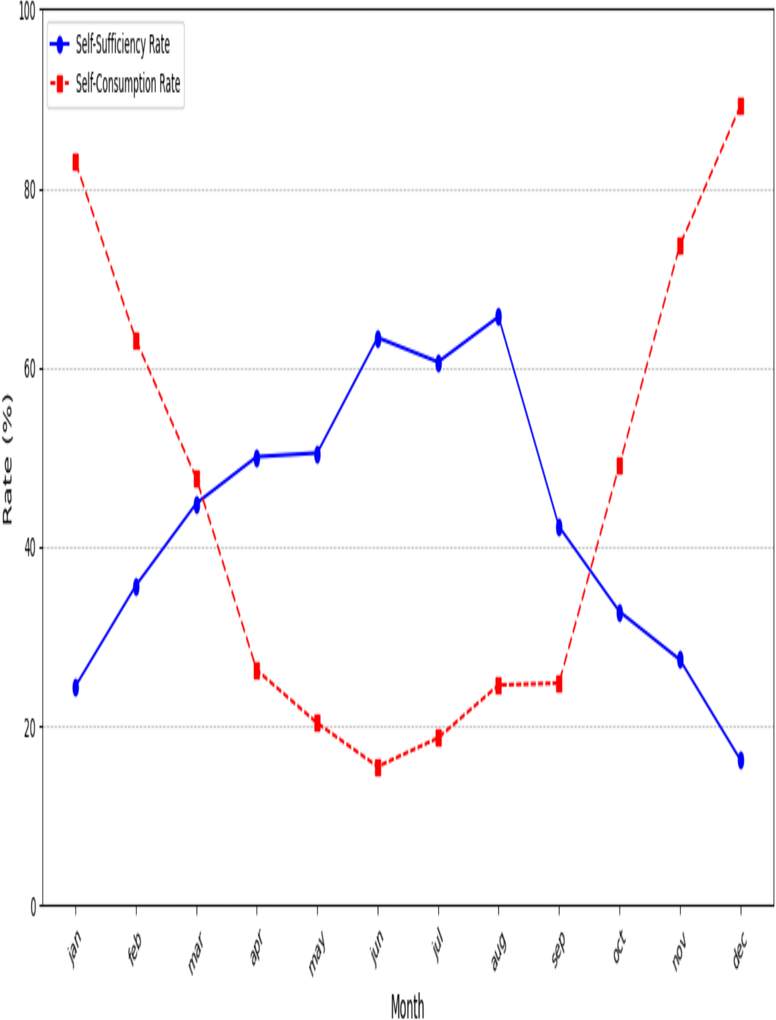
Scenario: 5kWh - Performance Rates
