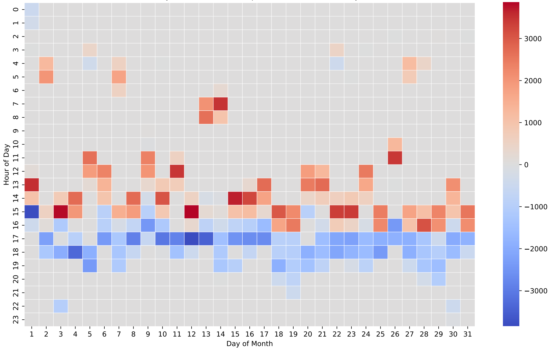
Battery Net Power Heatmap (Wh/Hour) - 5kWh - May
