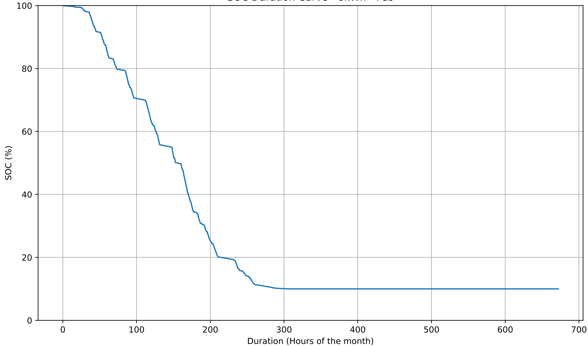
SOC Duration Curve - 8kWh - Feb
