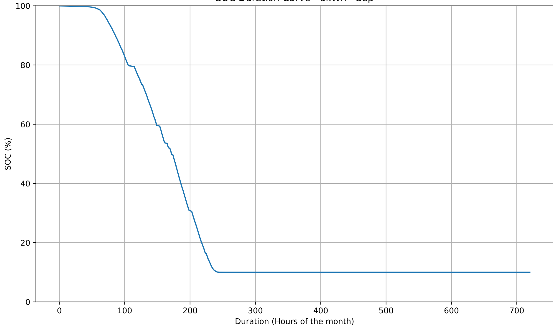
SOC Duration Curve - 8kWh - Sep
