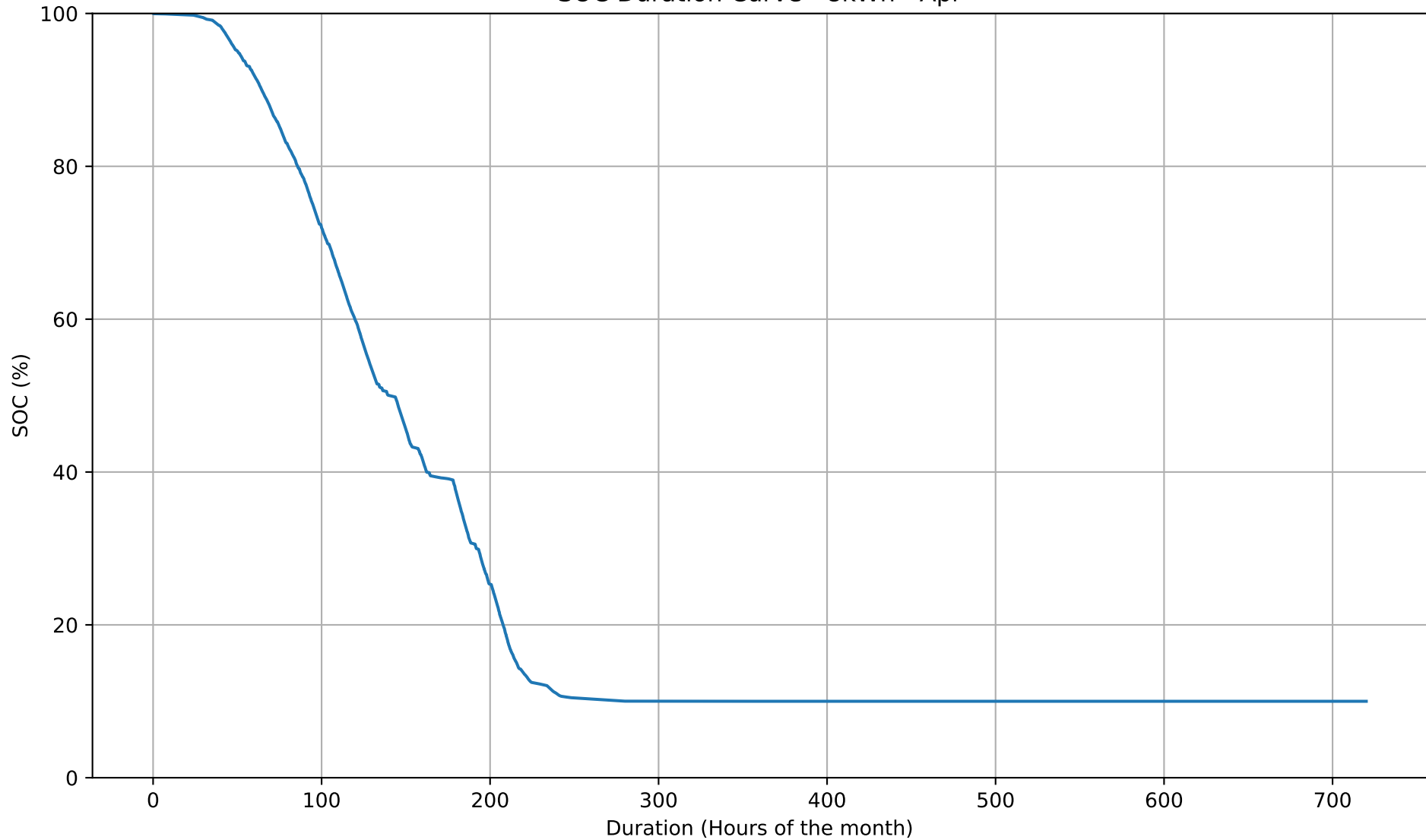
SOC Duration Curve - 8kWh - Apr
