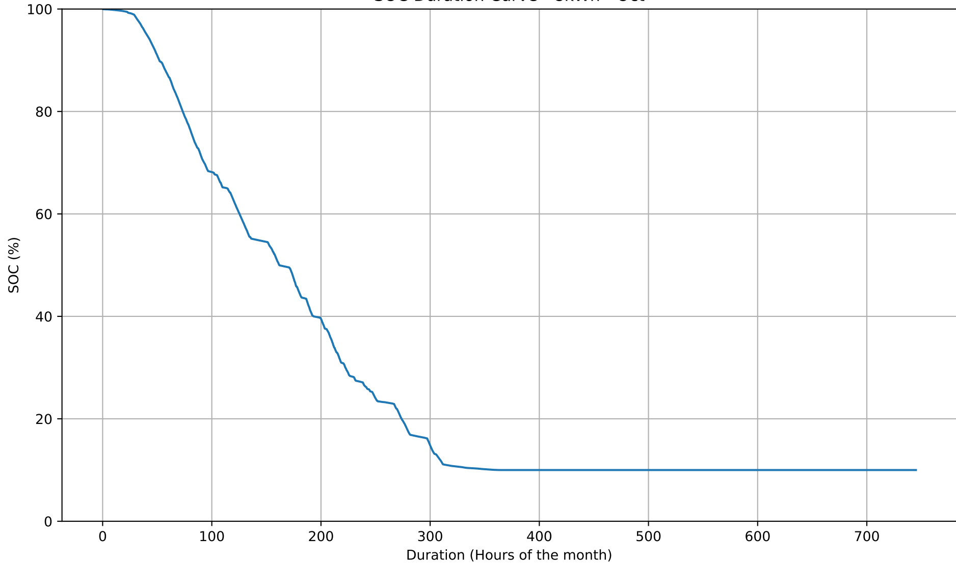
SOC Duration Curve - 8kWh - Oct
