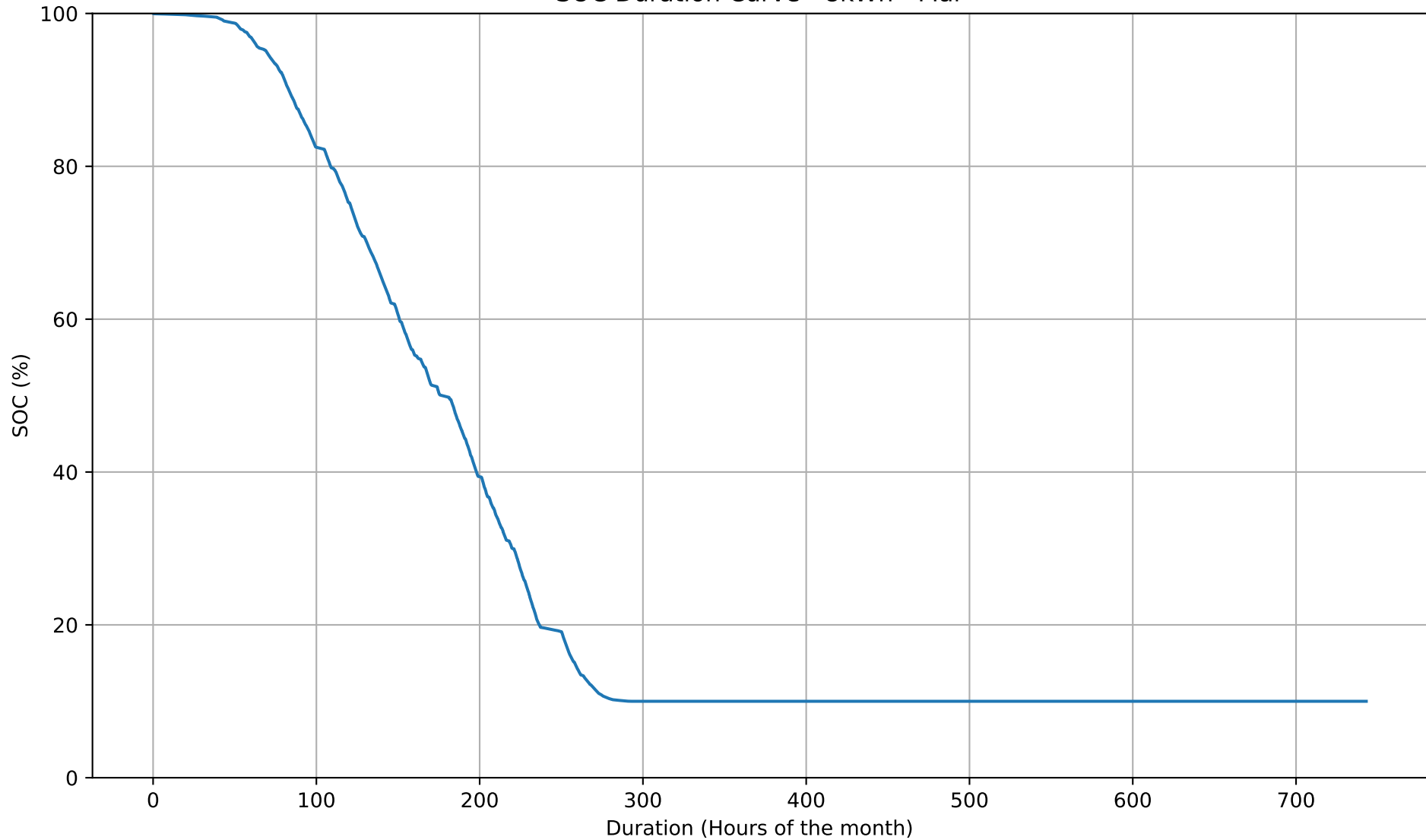
SOC Duration Curve - 8kWh - Mar
