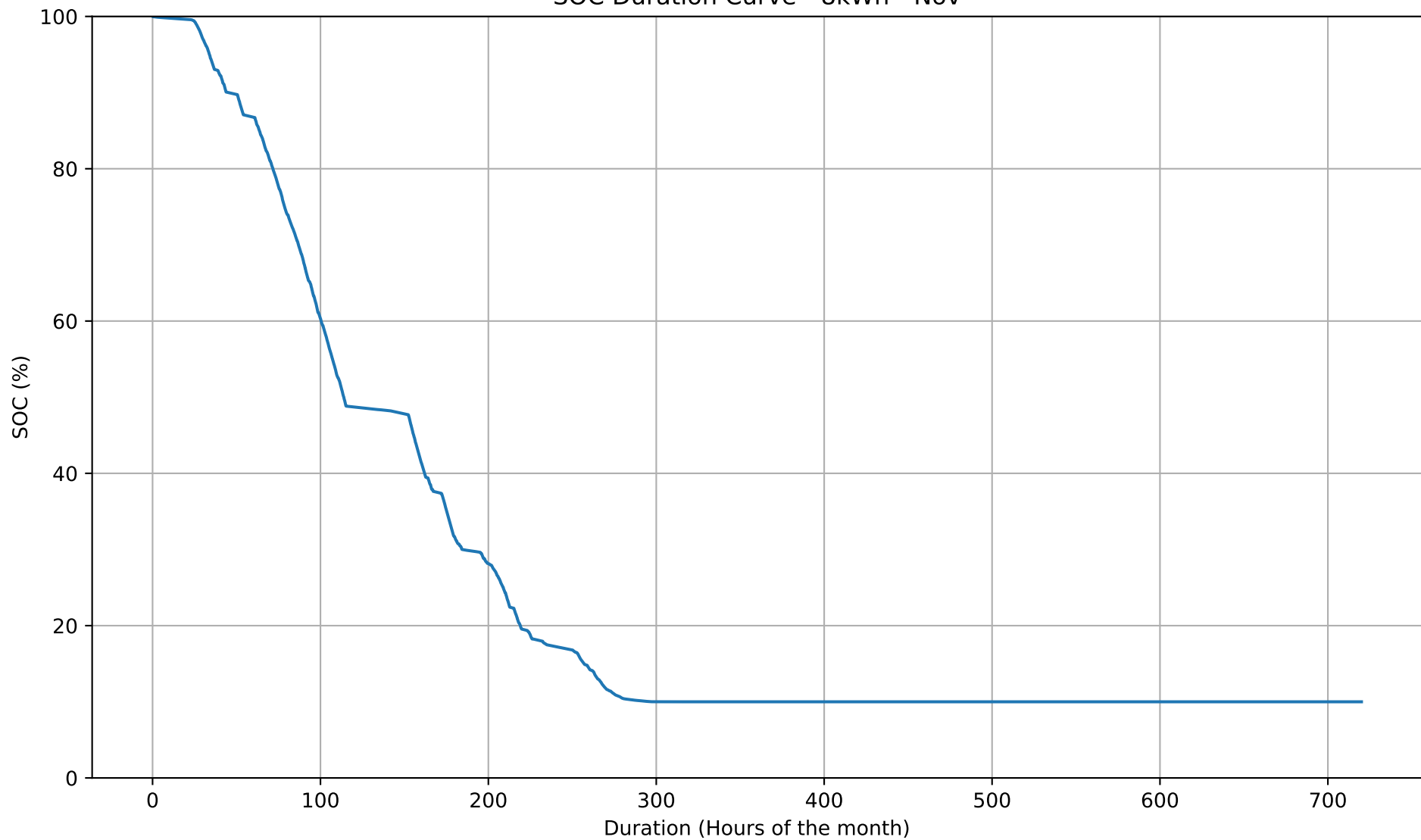
SOC Duration Curve - 8kWh - Nov
