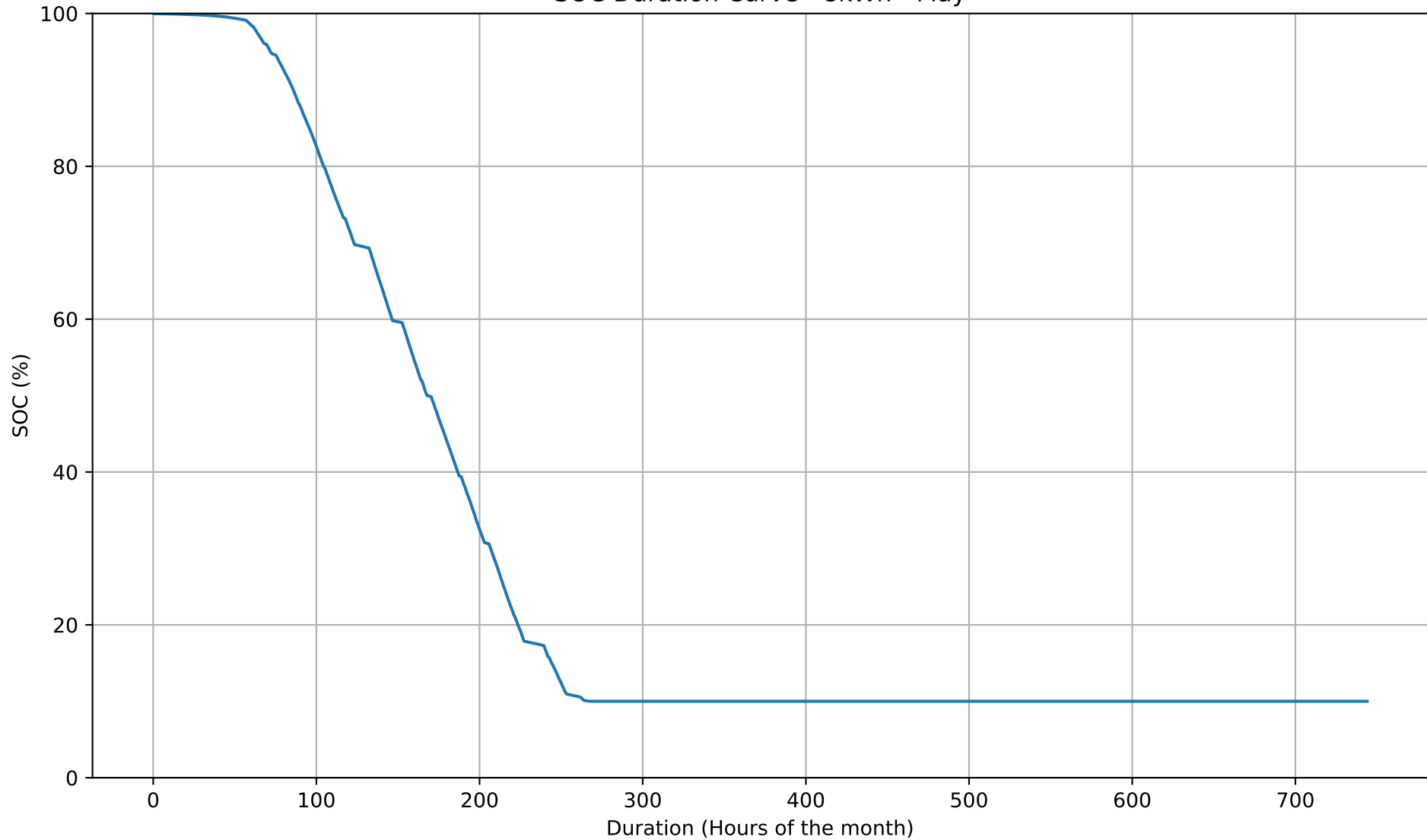
SOC Duration Curve - 8kWh - May
