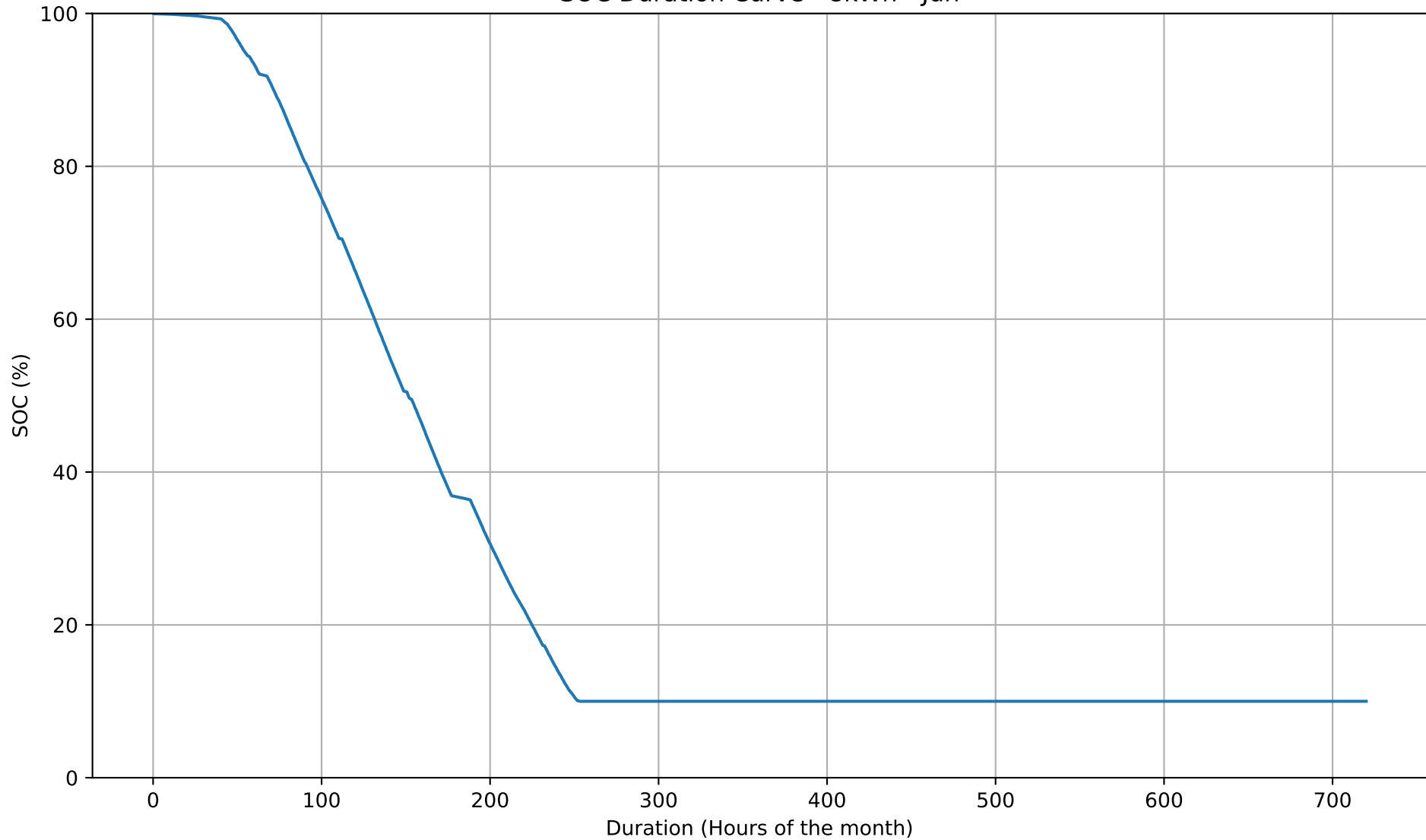
SOC Duration Curve - 8kWh - Jun
