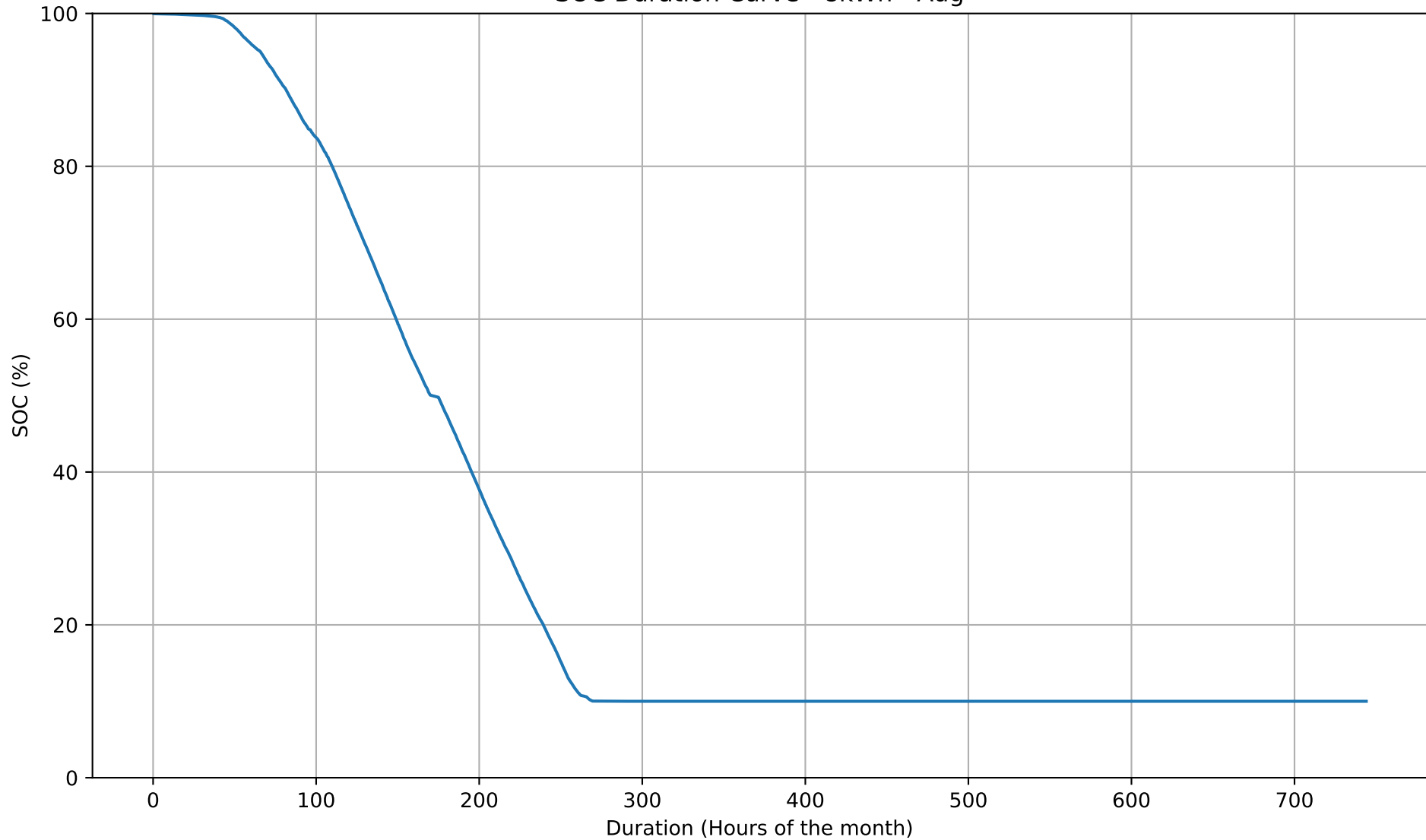
SOC Duration Curve - 8kWh - Aug
