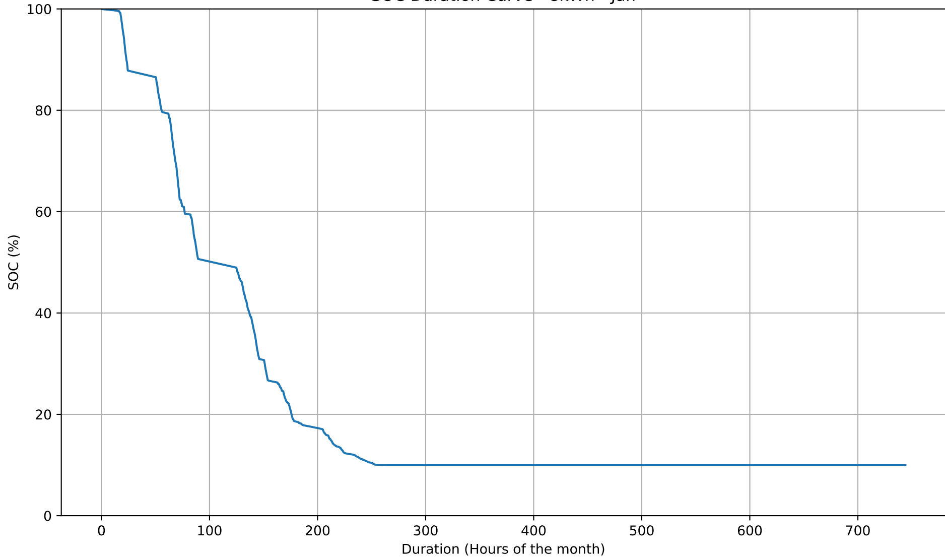
SOC Duration Curve - 8kWh - Jan
