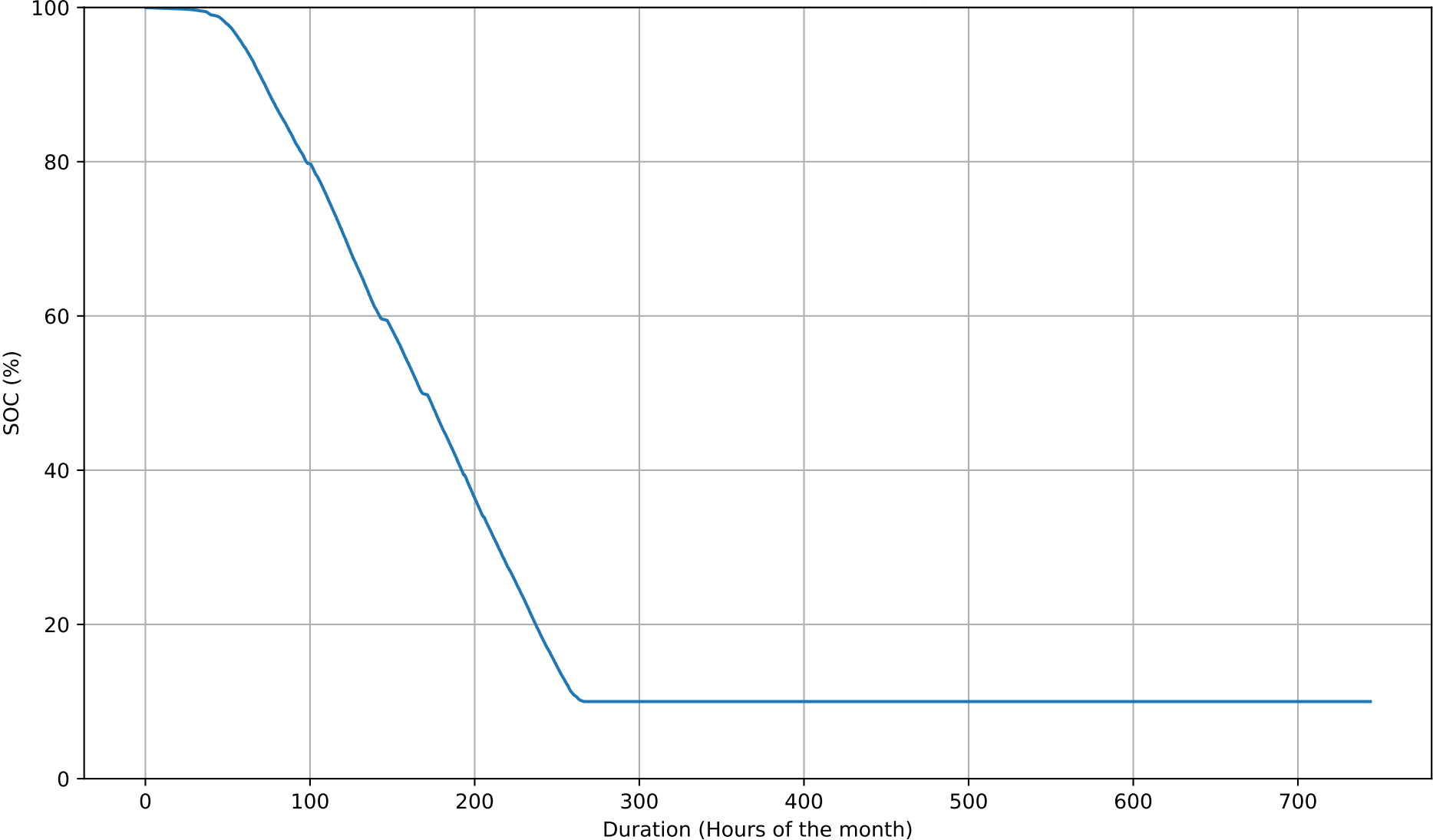
SOC Duration Curve - 8kWh - Jul
