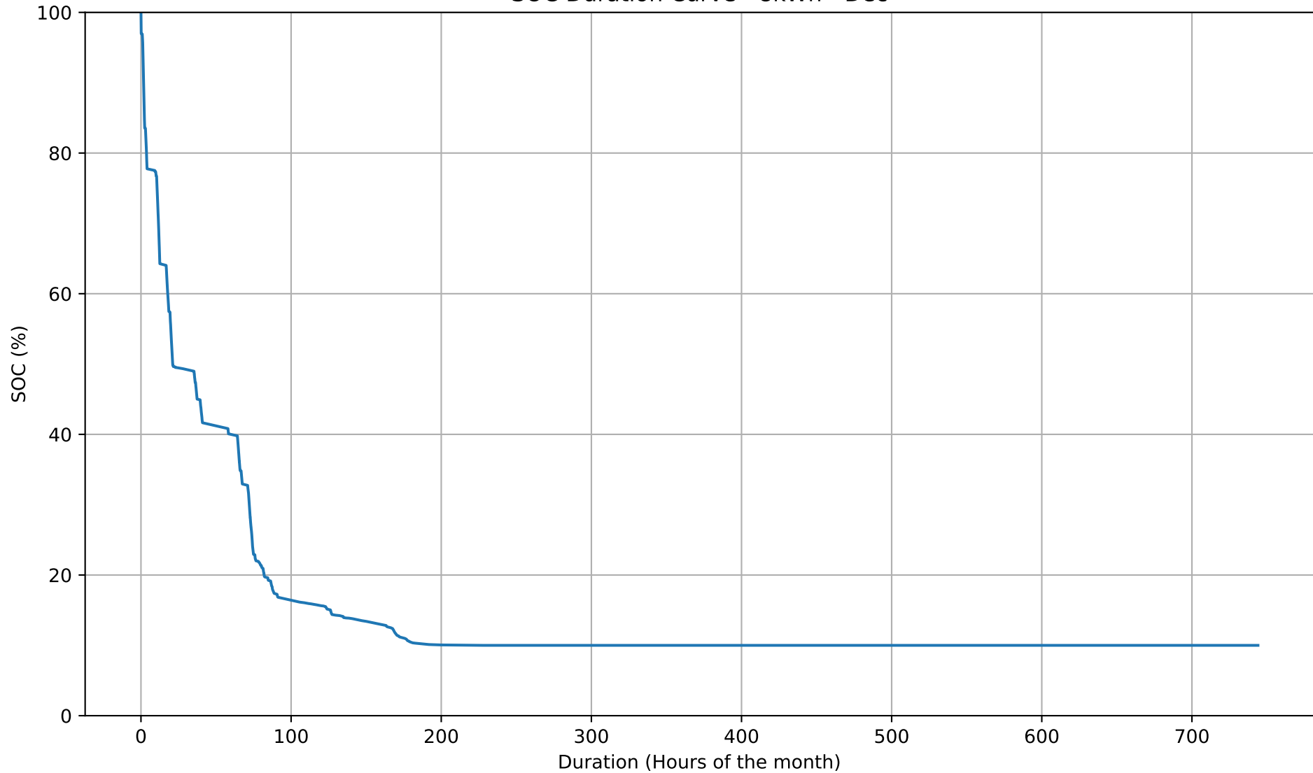
SOC Duration Curve - 8kWh - Dec
