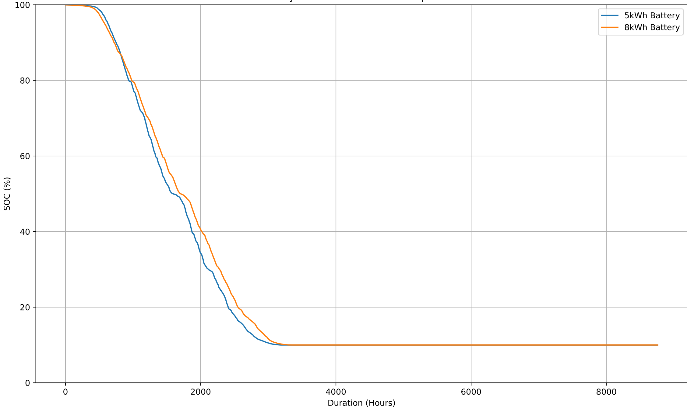
Yearly SOC Duration Curve Comparison
