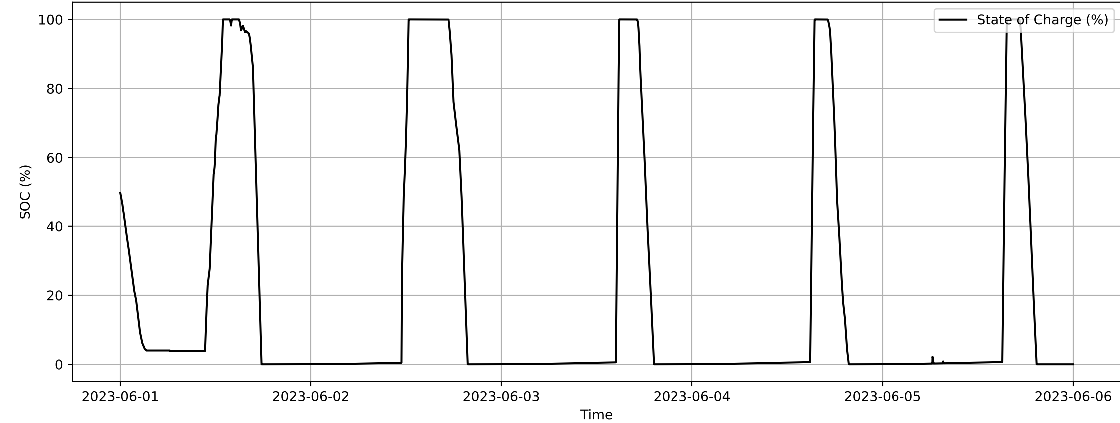
Battery State of Charge
