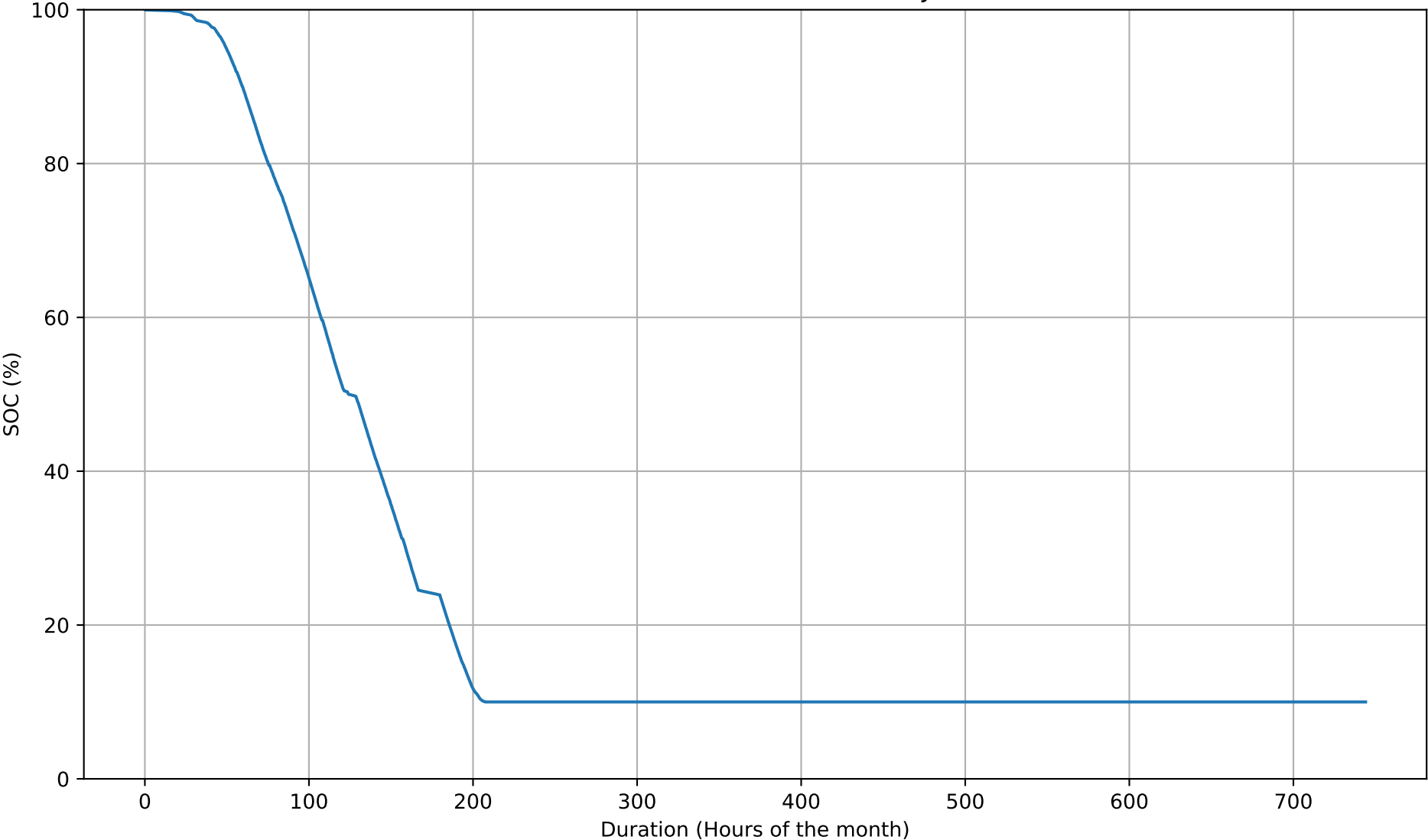
SOC Duration Curve - 5kWh - Jul
