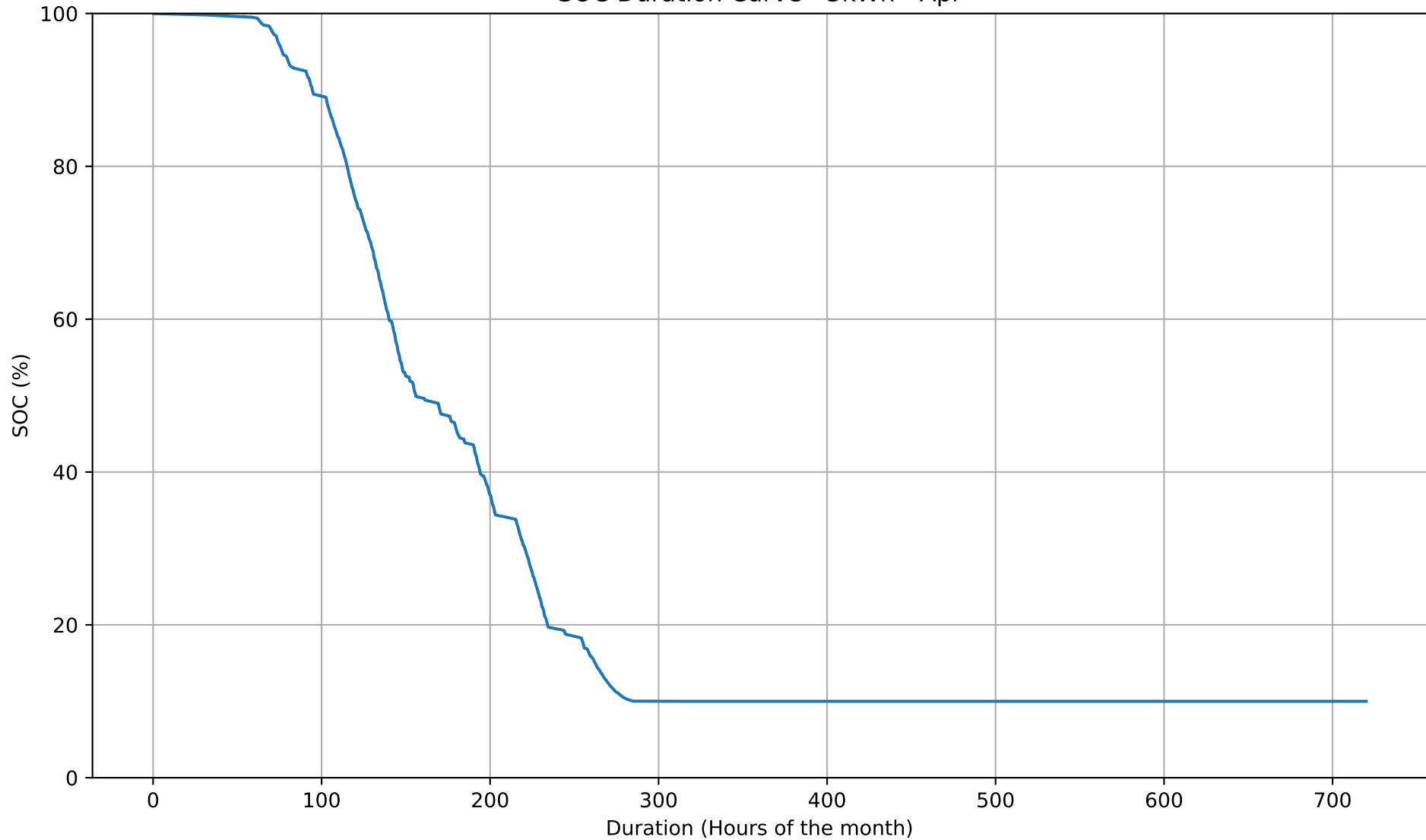
SOC Duration Curve - 5kWh - Apr
