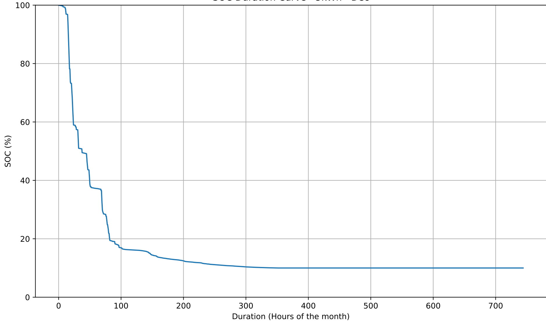
SOC Duration Curve - 5kWh - Dec
