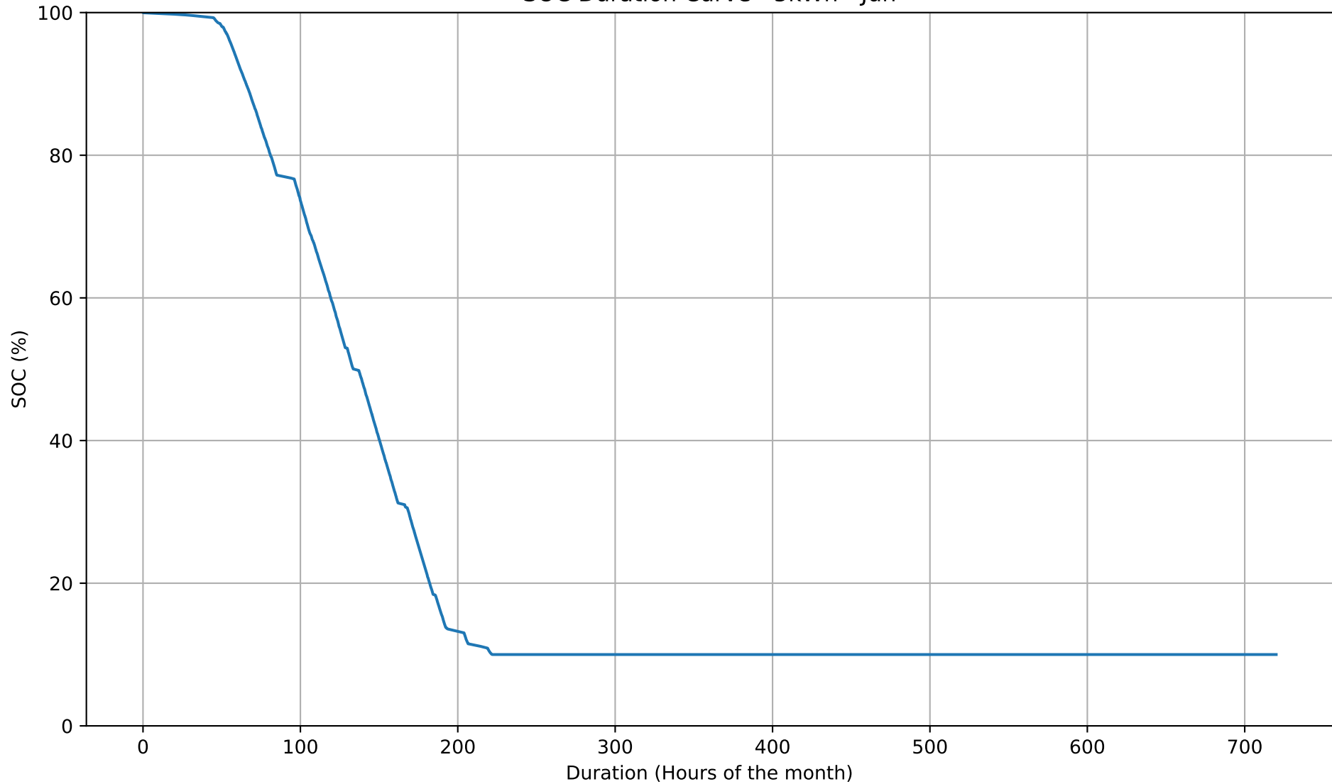
SOC Duration Curve - 5kWh - Jun
