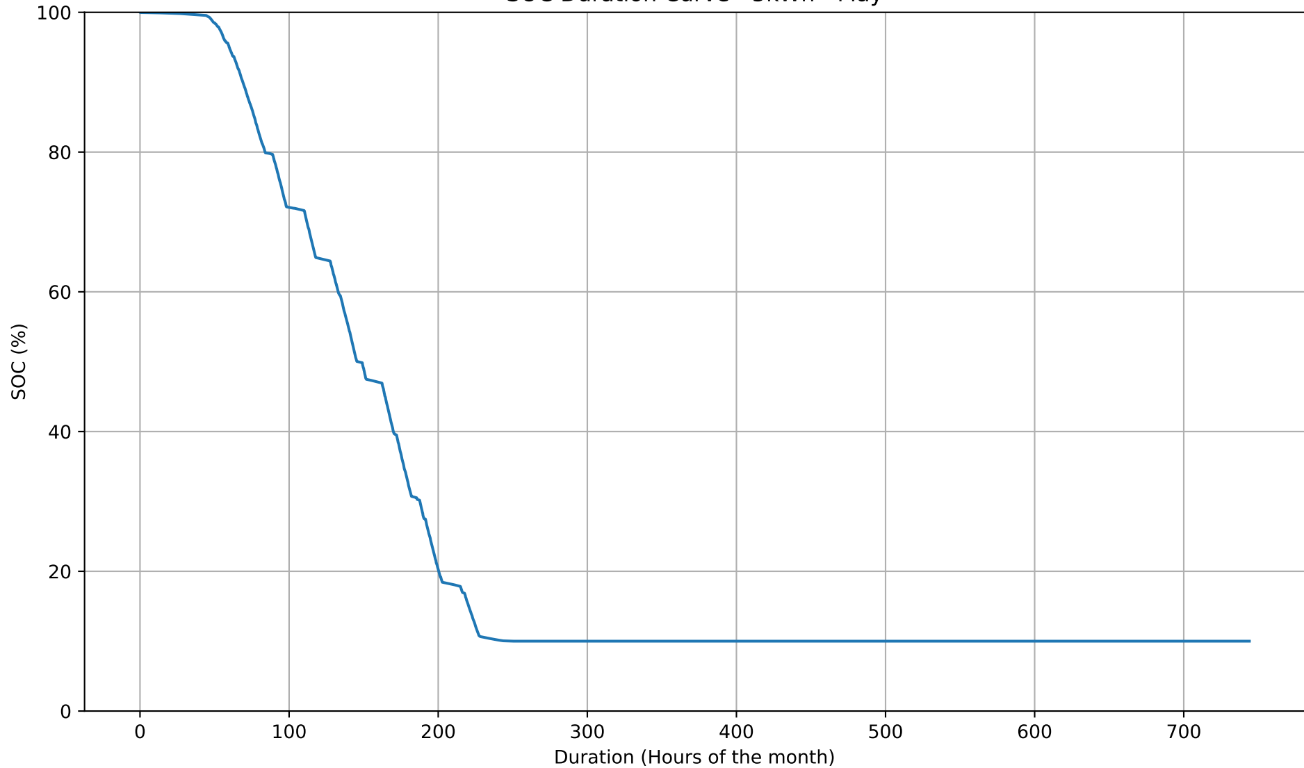
SOC Duration Curve - 5kWh - May
