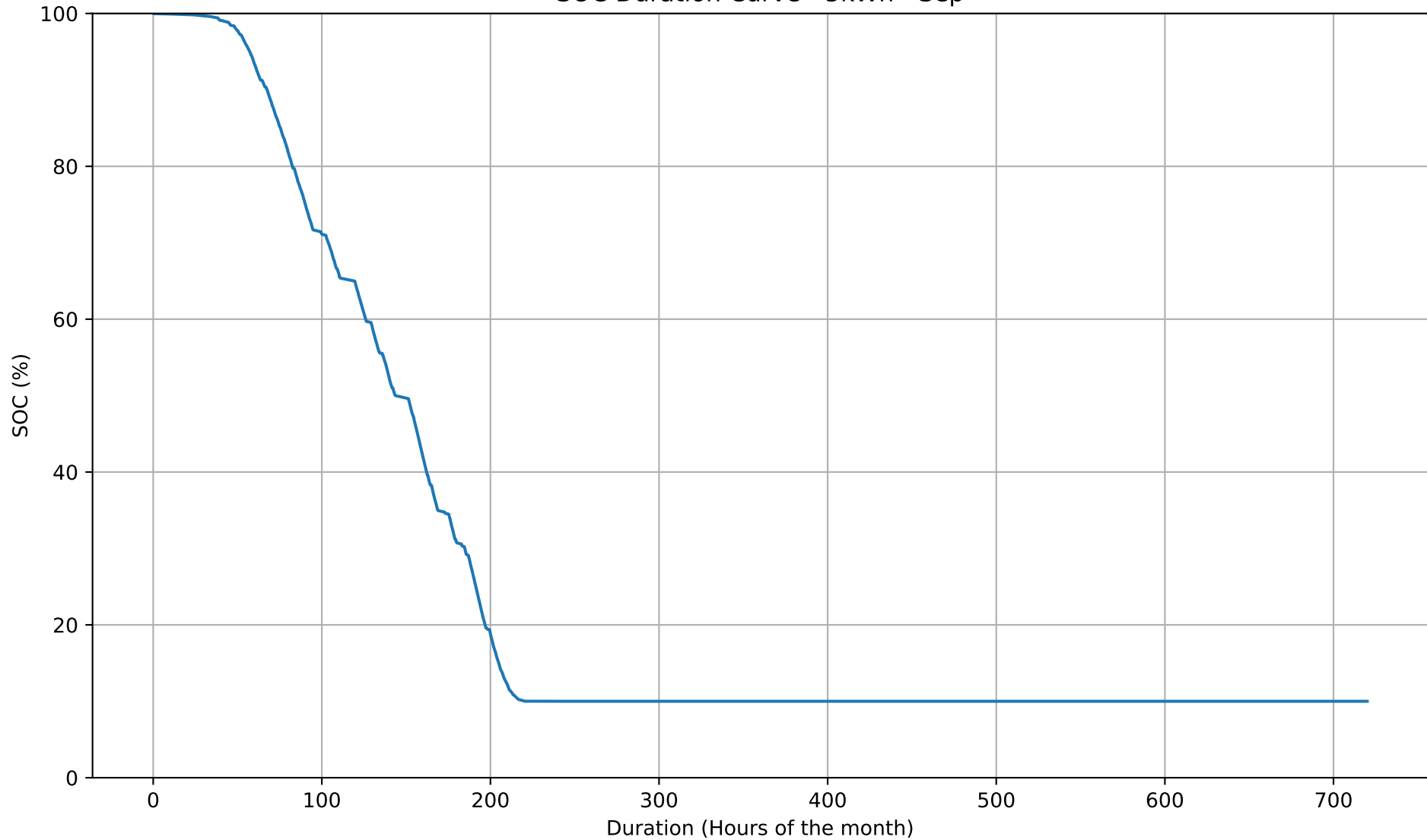
SOC Duration Curve - 5kWh - Sep
