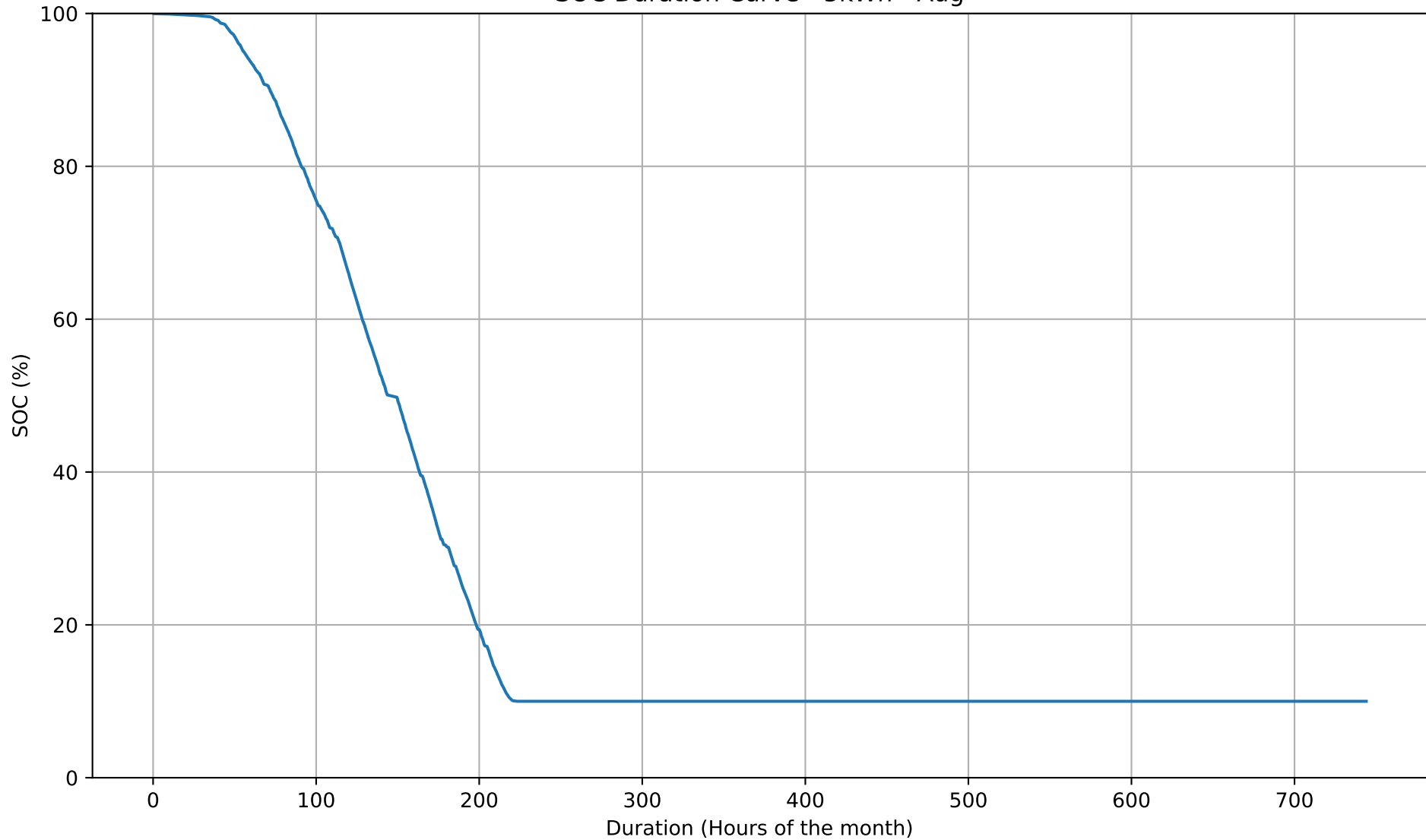
SOC Duration Curve - 5kWh - Aug
