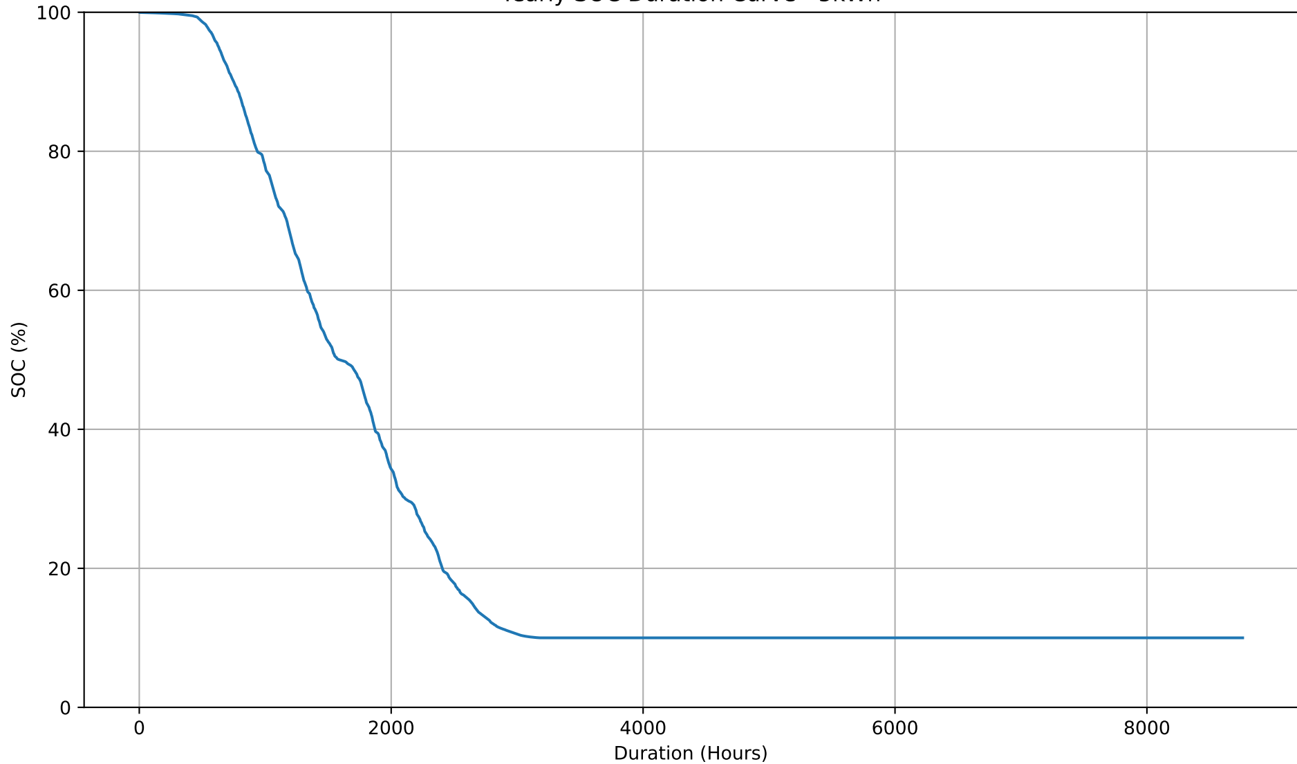
Yearly SOC Duration Curve - 5kWh
