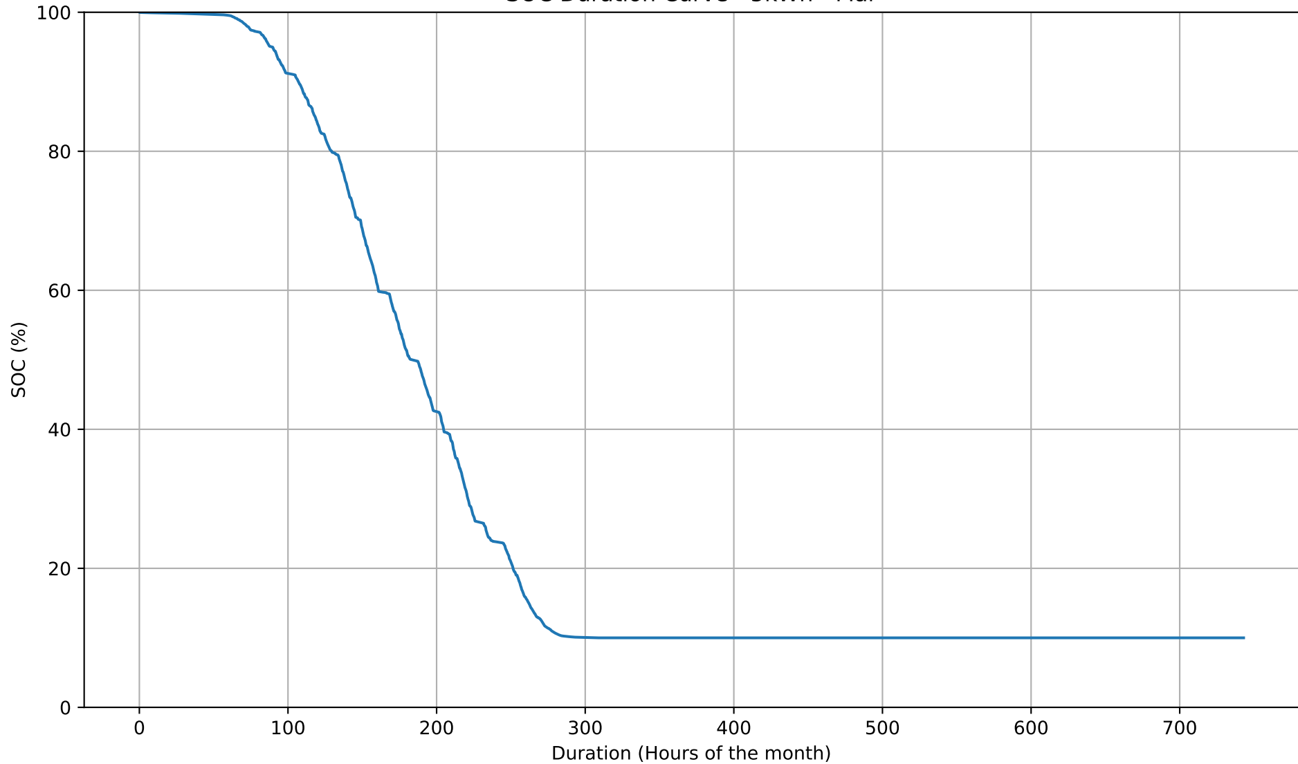
SOC Duration Curve - 5kWh - Mar
