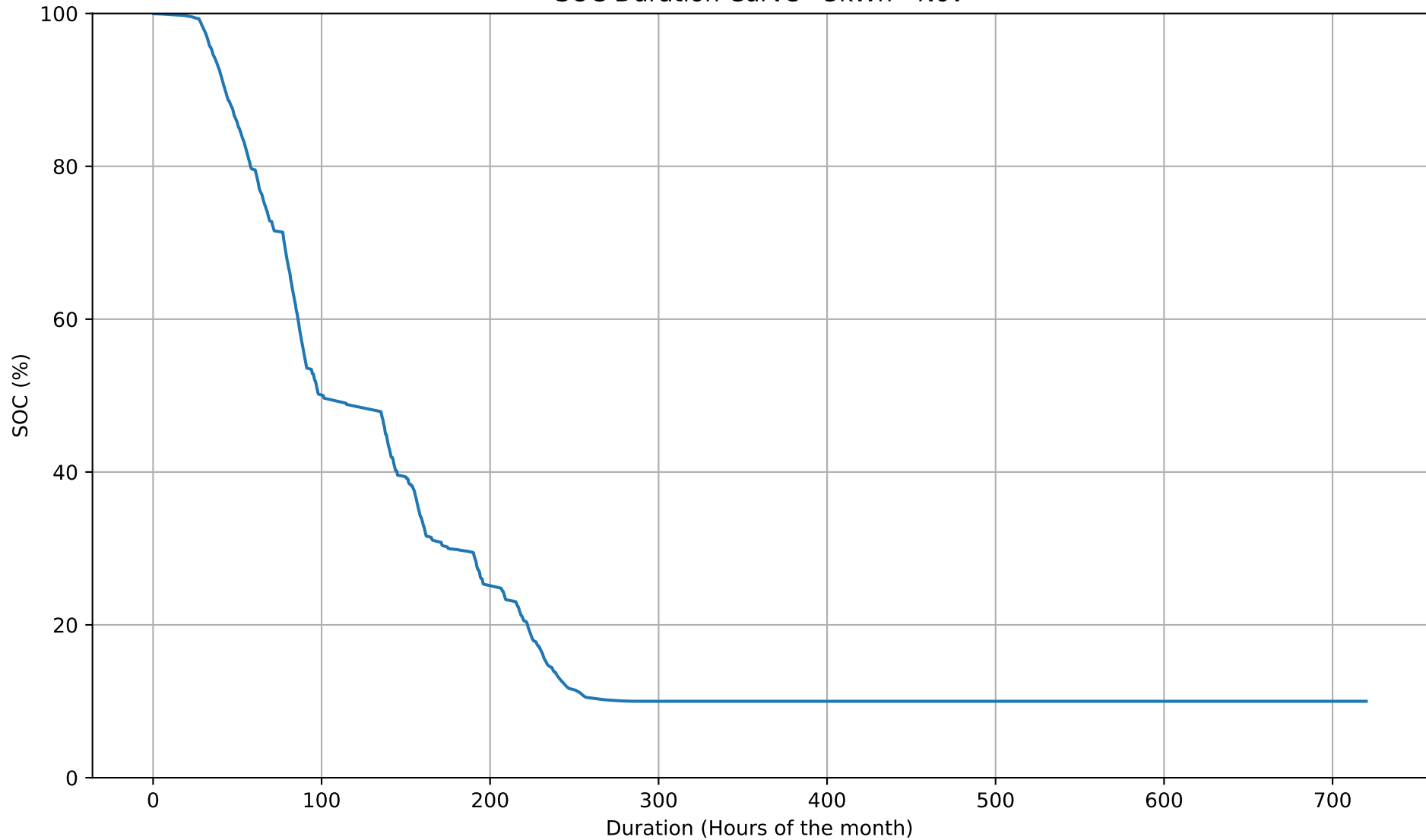
SOC Duration Curve - 5kWh - Nov
