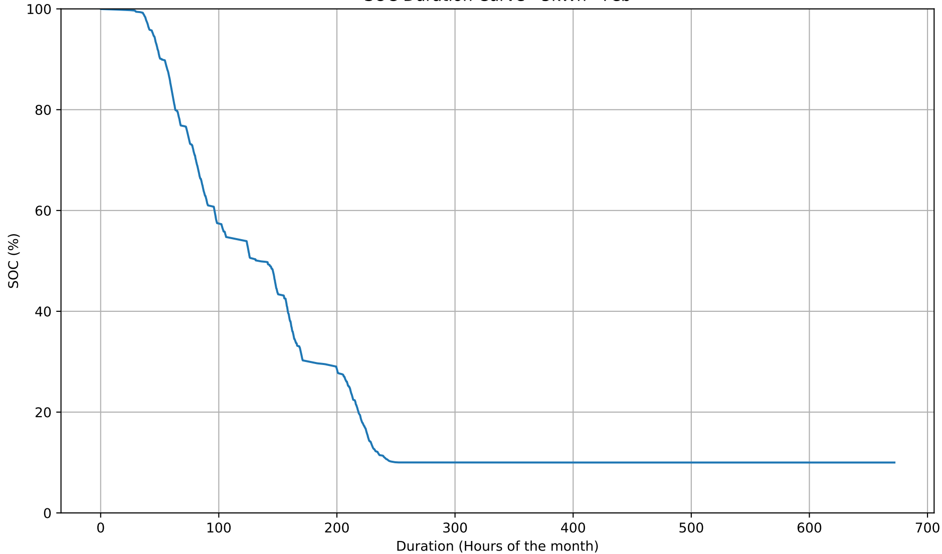
SOC Duration Curve - 5kWh - Feb
