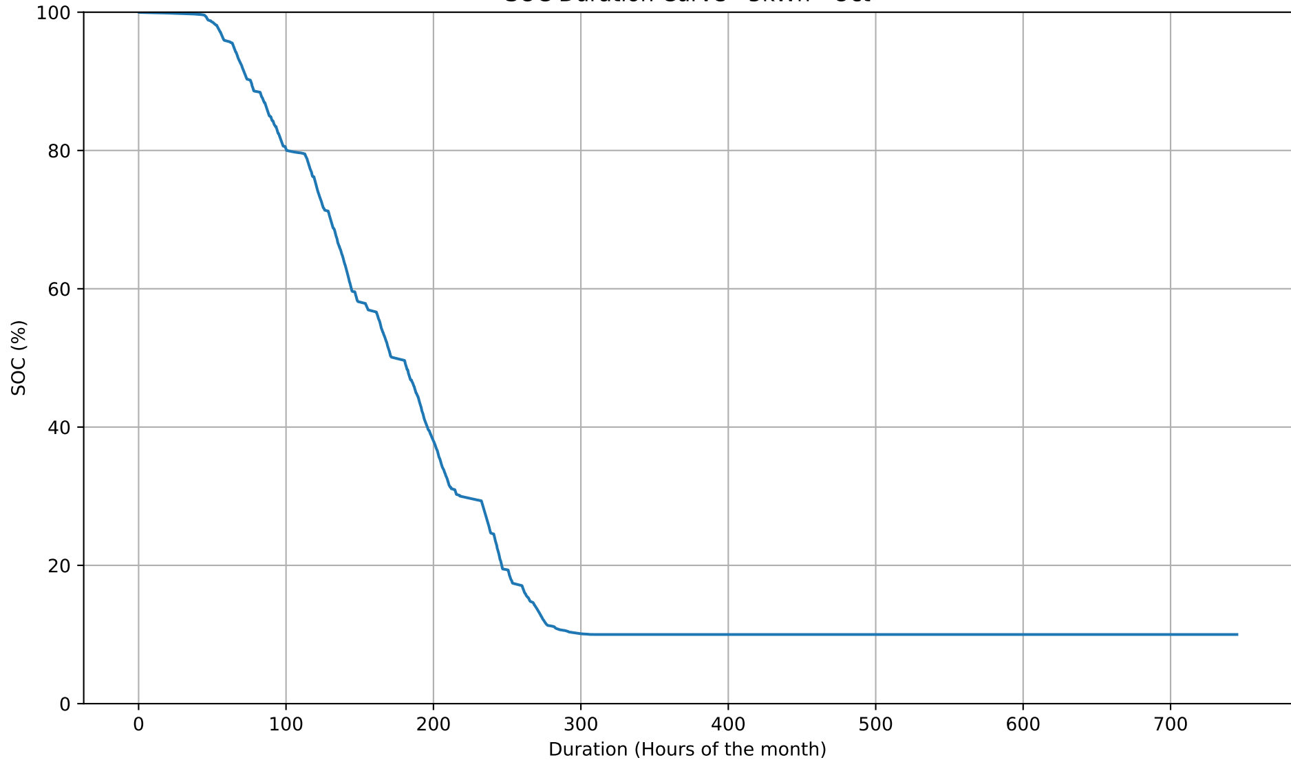
SOC Duration Curve - 5kWh - Oct
