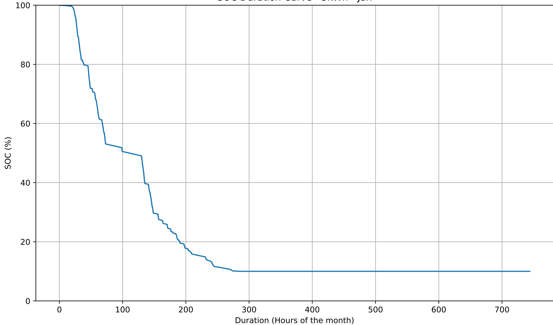
SOC Duration Curve - 5kWh - Jan
