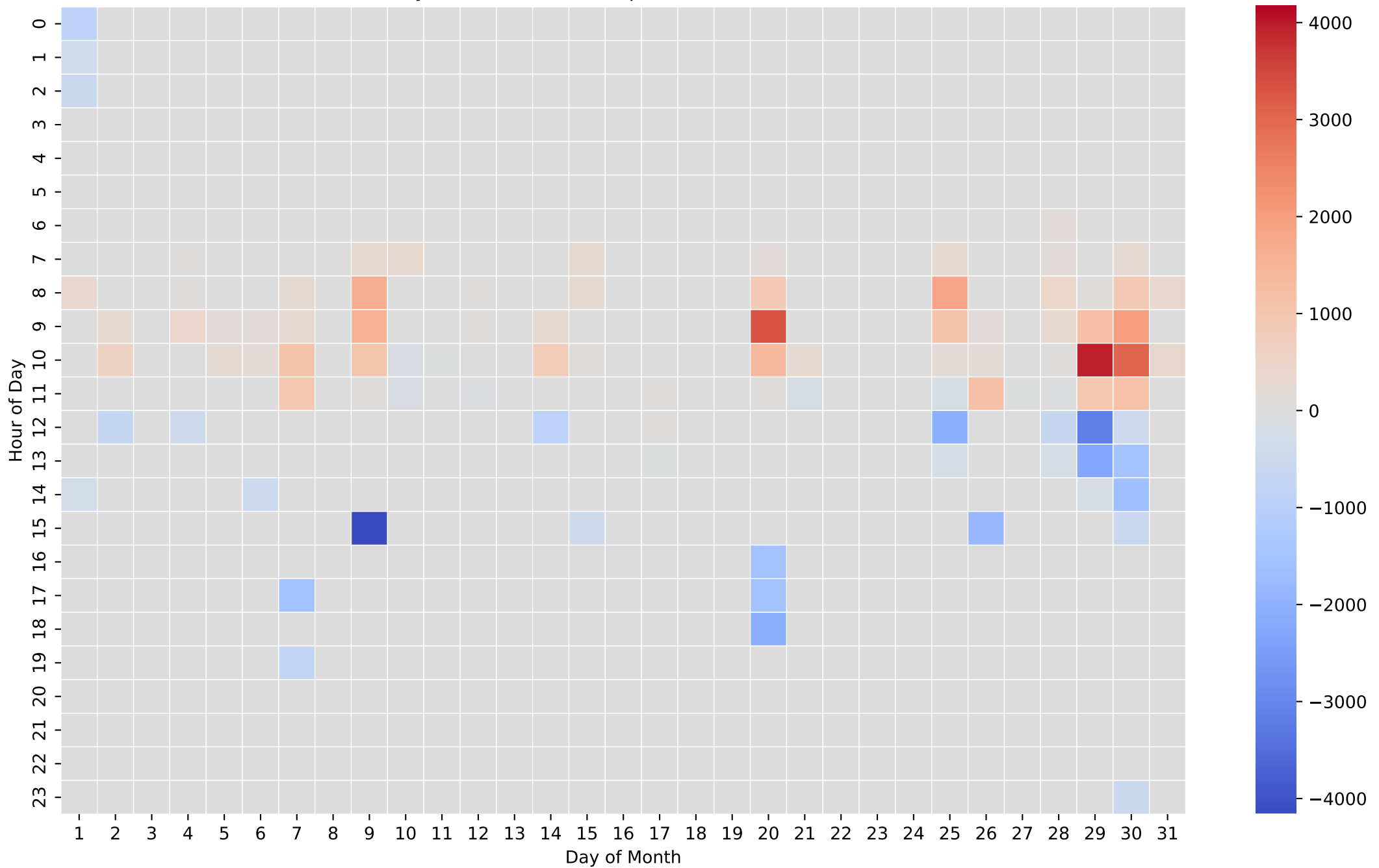
Battery Net Power Heatmap (Wh/Hour) - 8kWh - Dec
