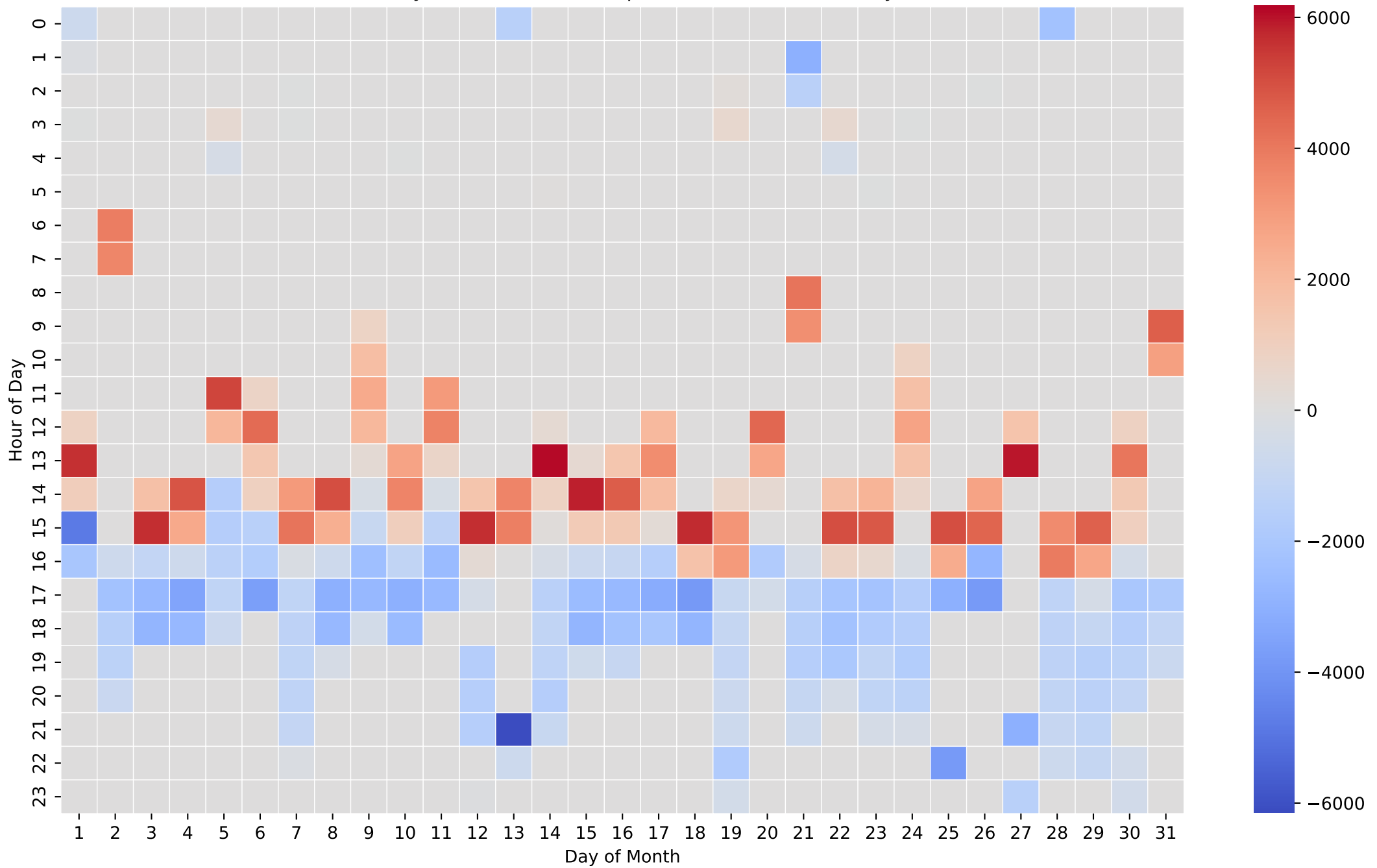
Battery Net Power Heatmap (Wh/Hour) - 8kWh - May
