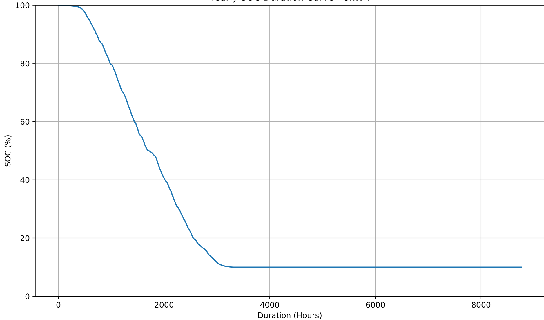
Yearly SOC Duration Curve - 8kWh
