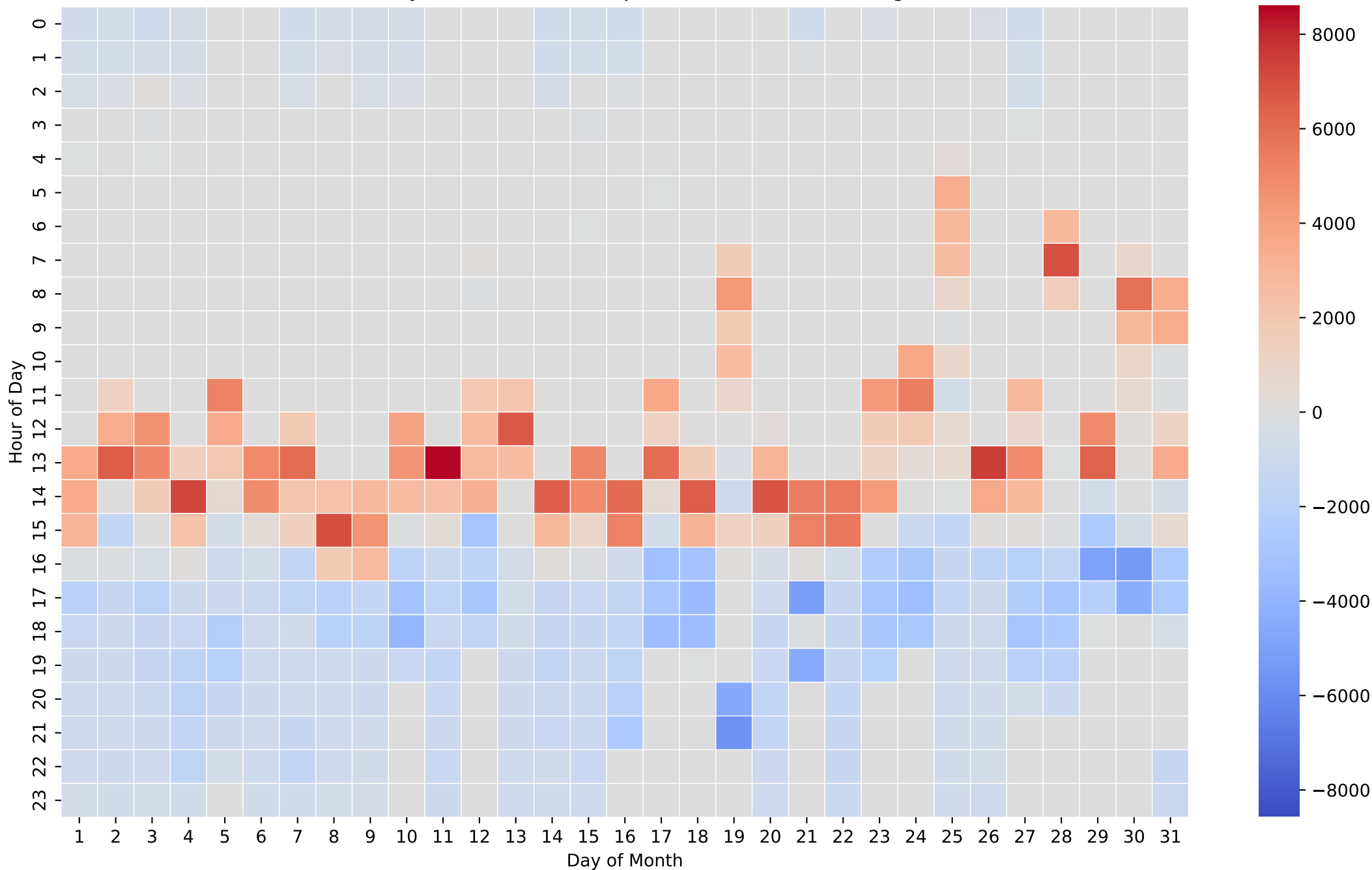
Battery Net Power Heatmap (Wh/Hour) - 12kWh - Aug
