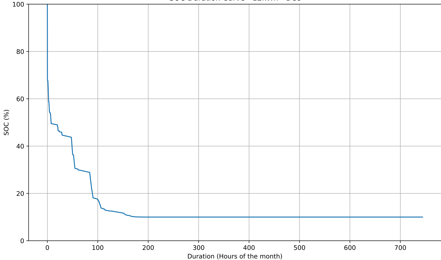
SOC Duration Curve - 12kWh - Dec
