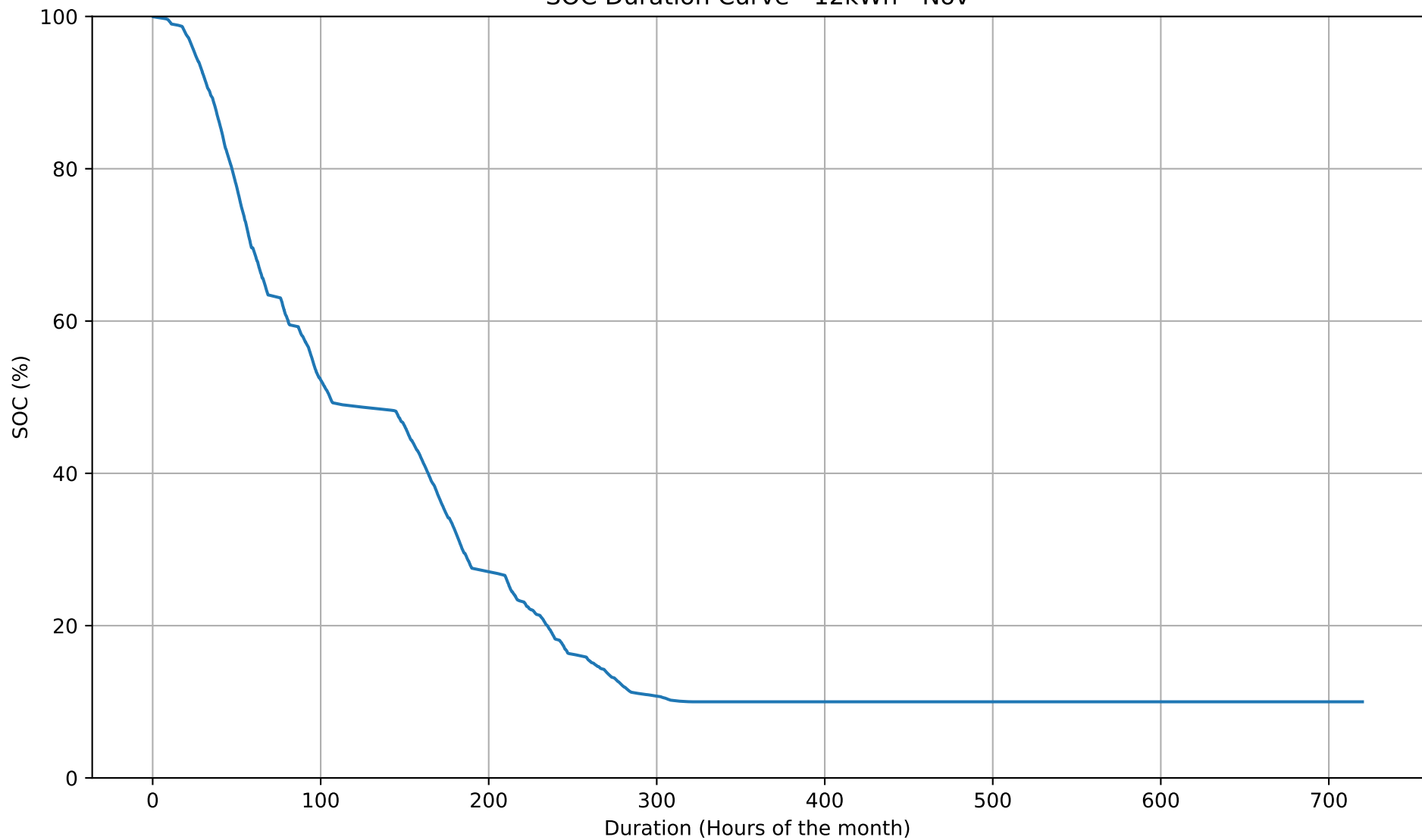
SOC Duration Curve - 12kWh - Nov
