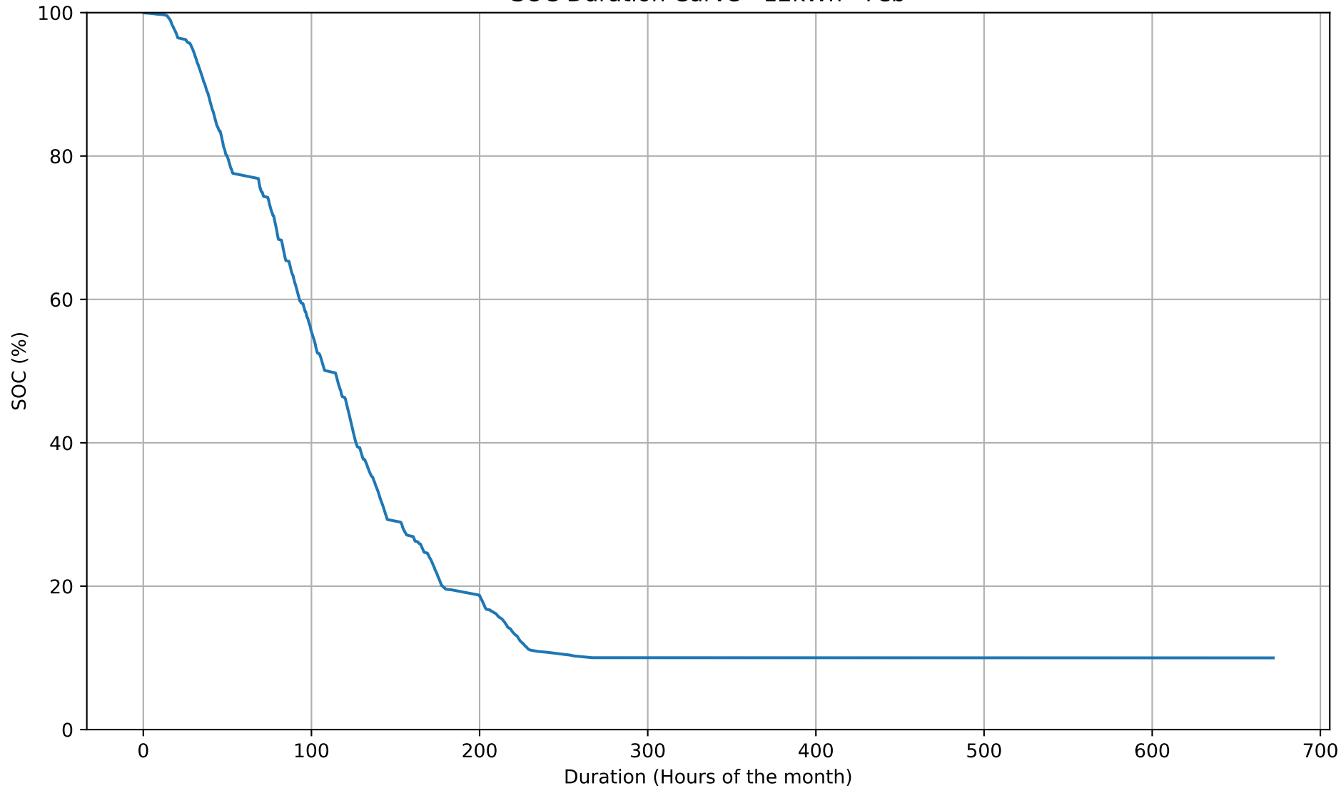
SOC Duration Curve - 12kWh - Feb
