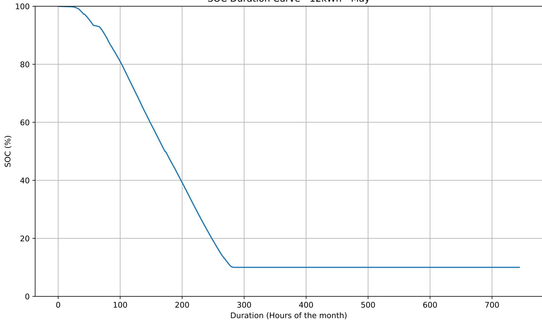
SOC Duration Curve - 12kWh - May
