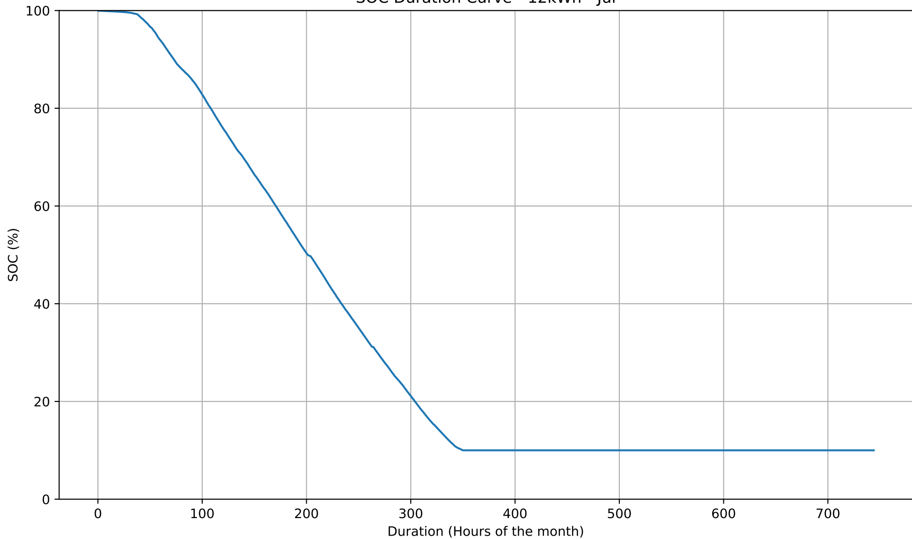
SOC Duration Curve - 12kWh - Jul
