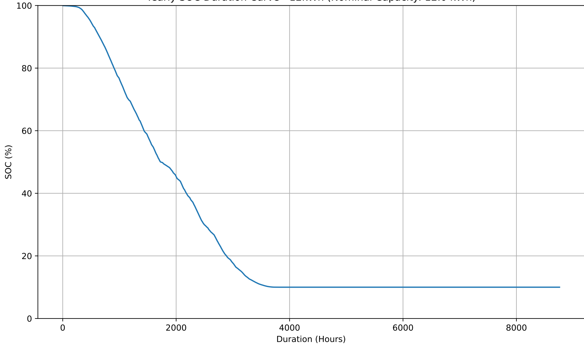
Yearly SOC Duration Curve - 12kWh (Nominal Capacity: 12.0 kWh)
