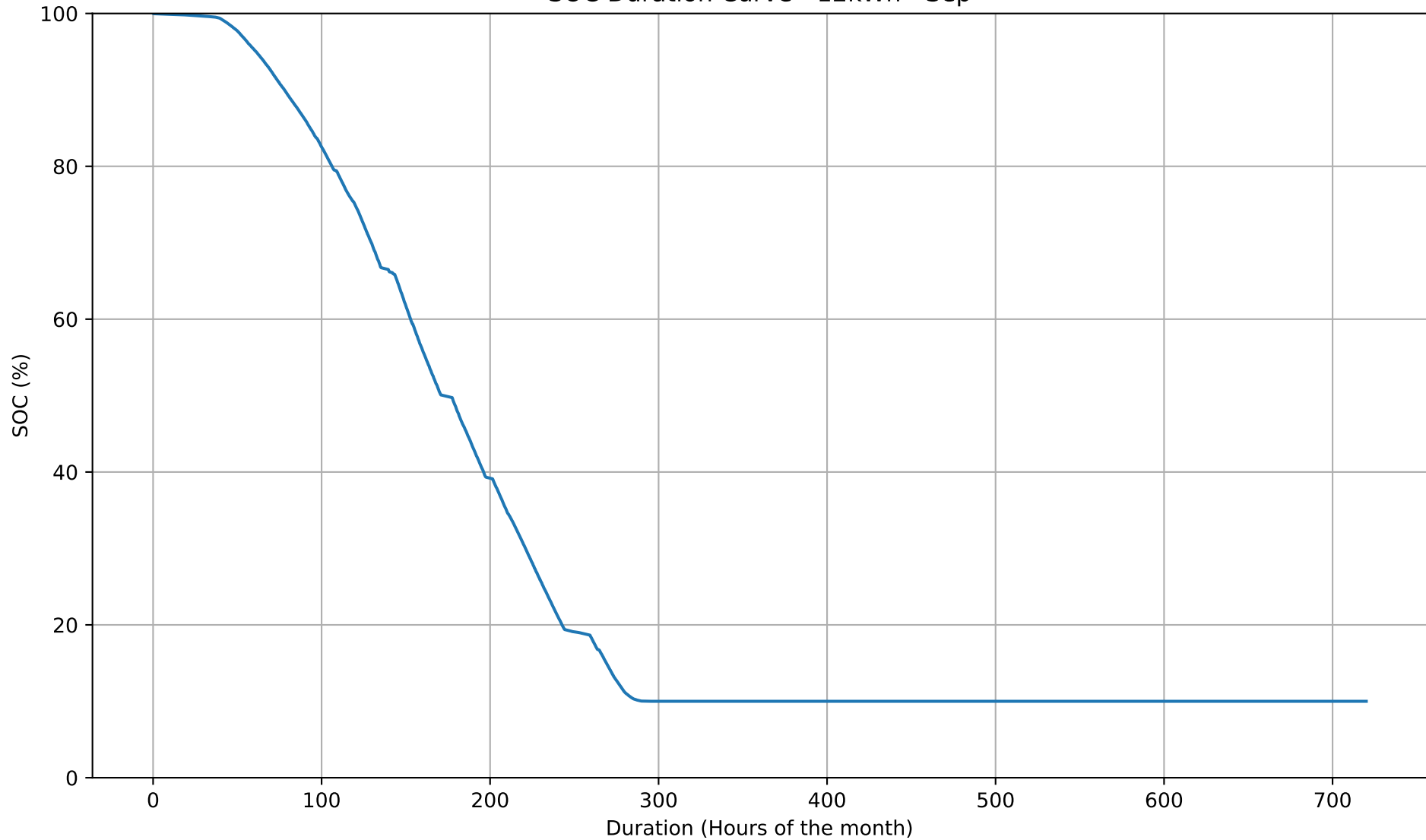
SOC Duration Curve - 12kWh - Sep
