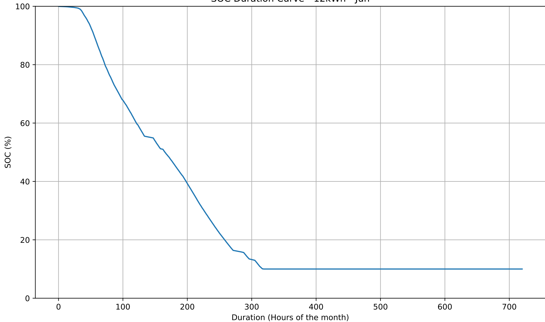
SOC Duration Curve - 12kWh - Jun
