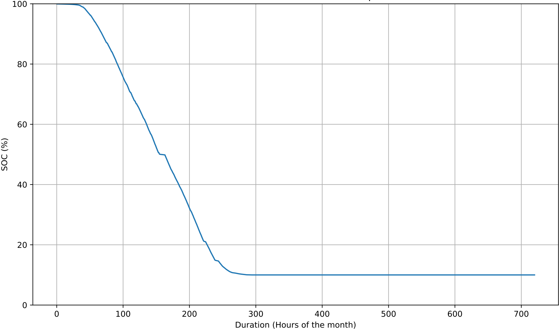
SOC Duration Curve - 12kWh - Apr
