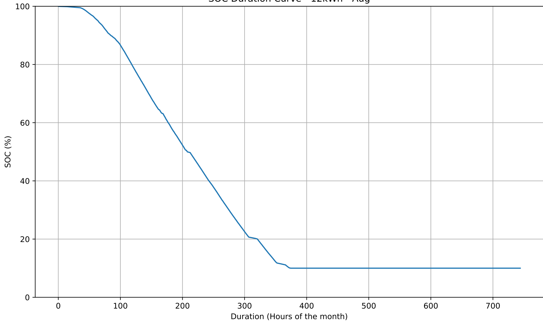
SOC Duration Curve - 12kWh - Aug
