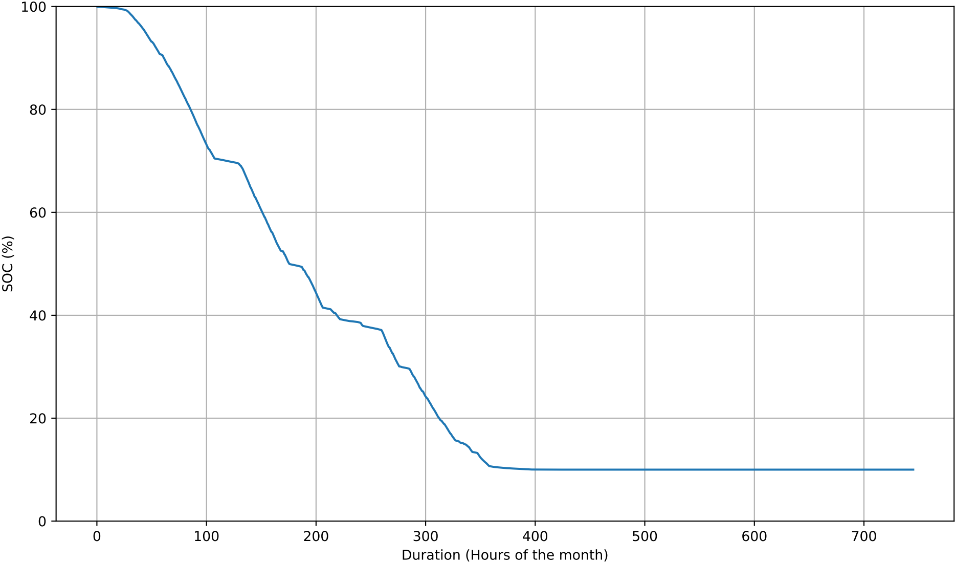
SOC Duration Curve - 12kWh - Oct
