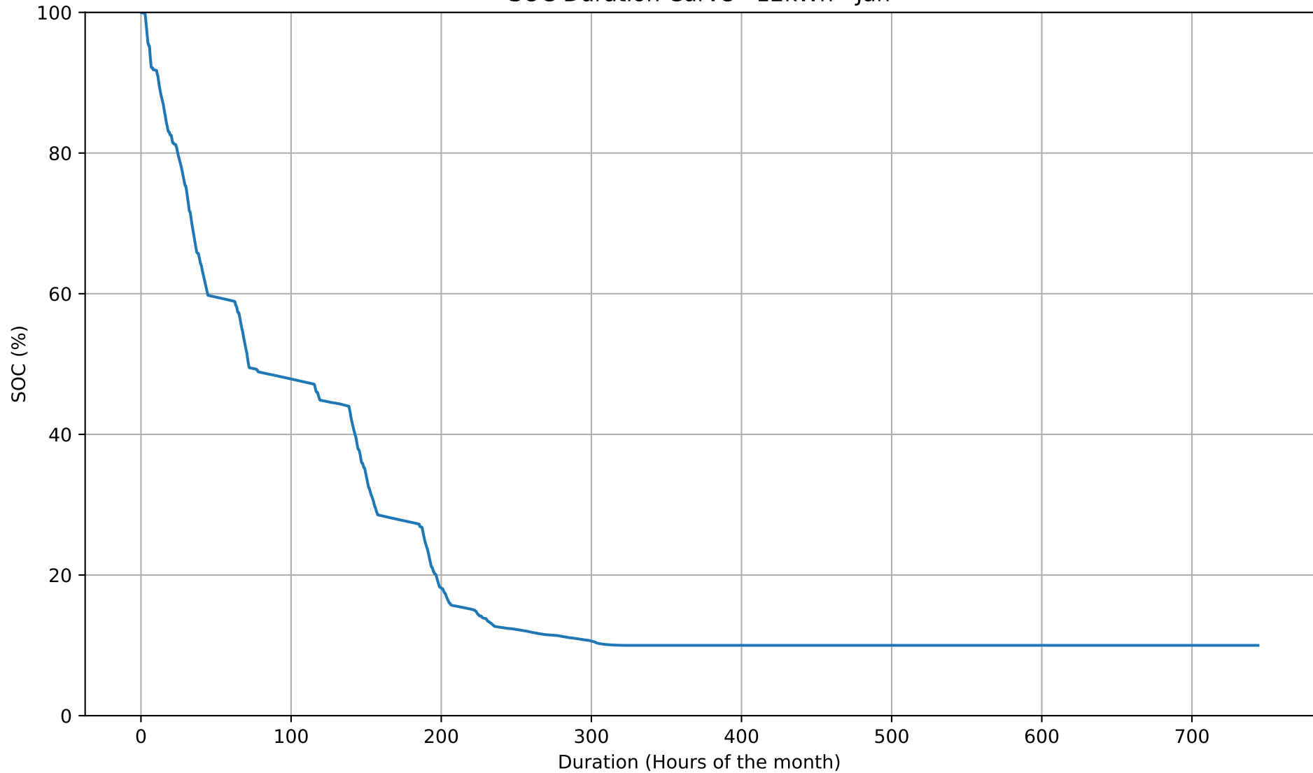
SOC Duration Curve - 12kWh - Jan
