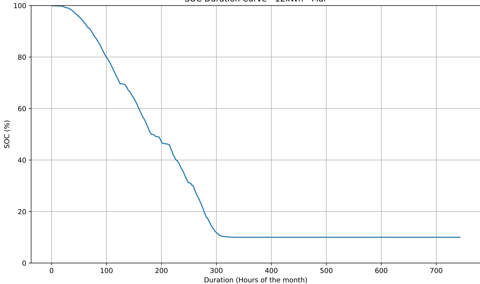
SOC Duration Curve - 12kWh - Mar
