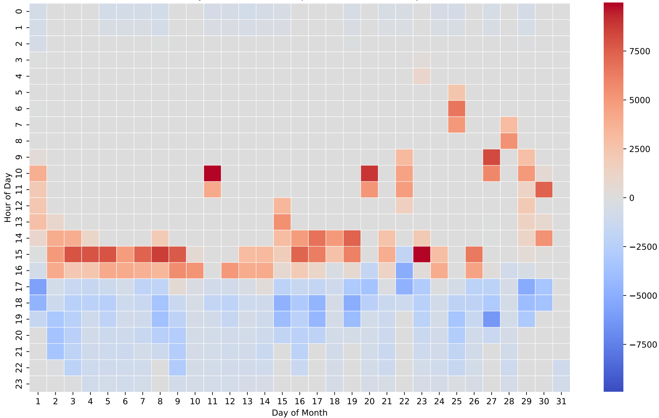
Battery Net Power Heatmap (Wh/Hour) - 15kWh - Jun
