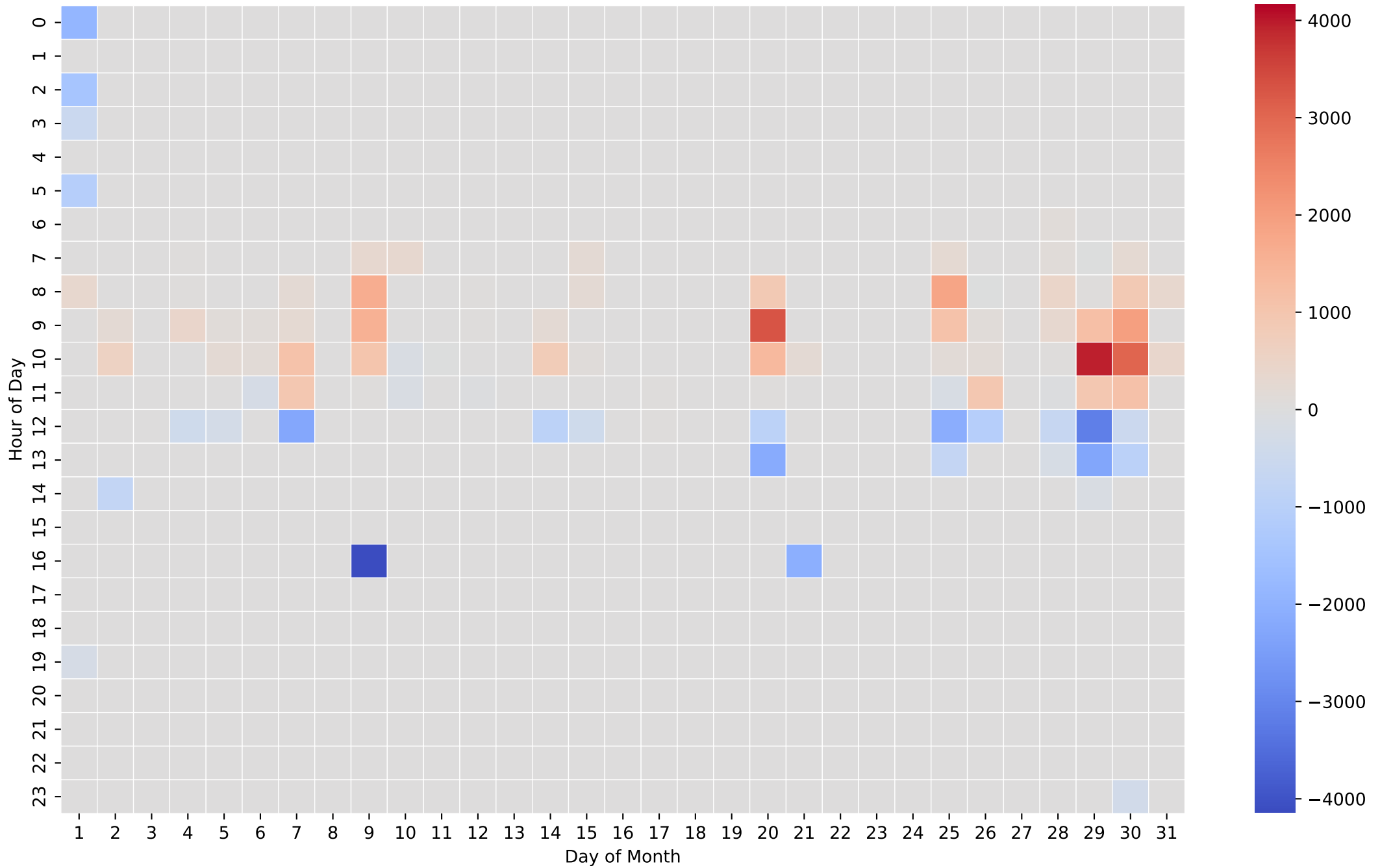
Battery Net Power Heatmap (Wh/Hour) - 15kWh - Dec
