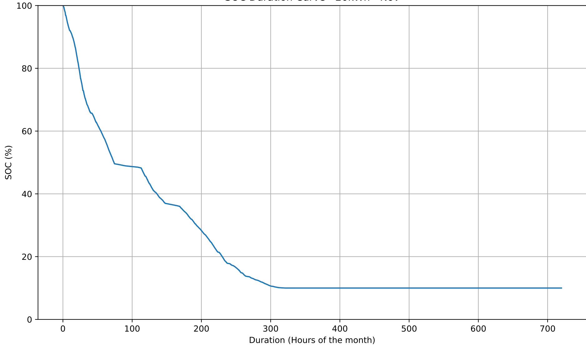
SOC Duration Curve - 20kWh - Nov
