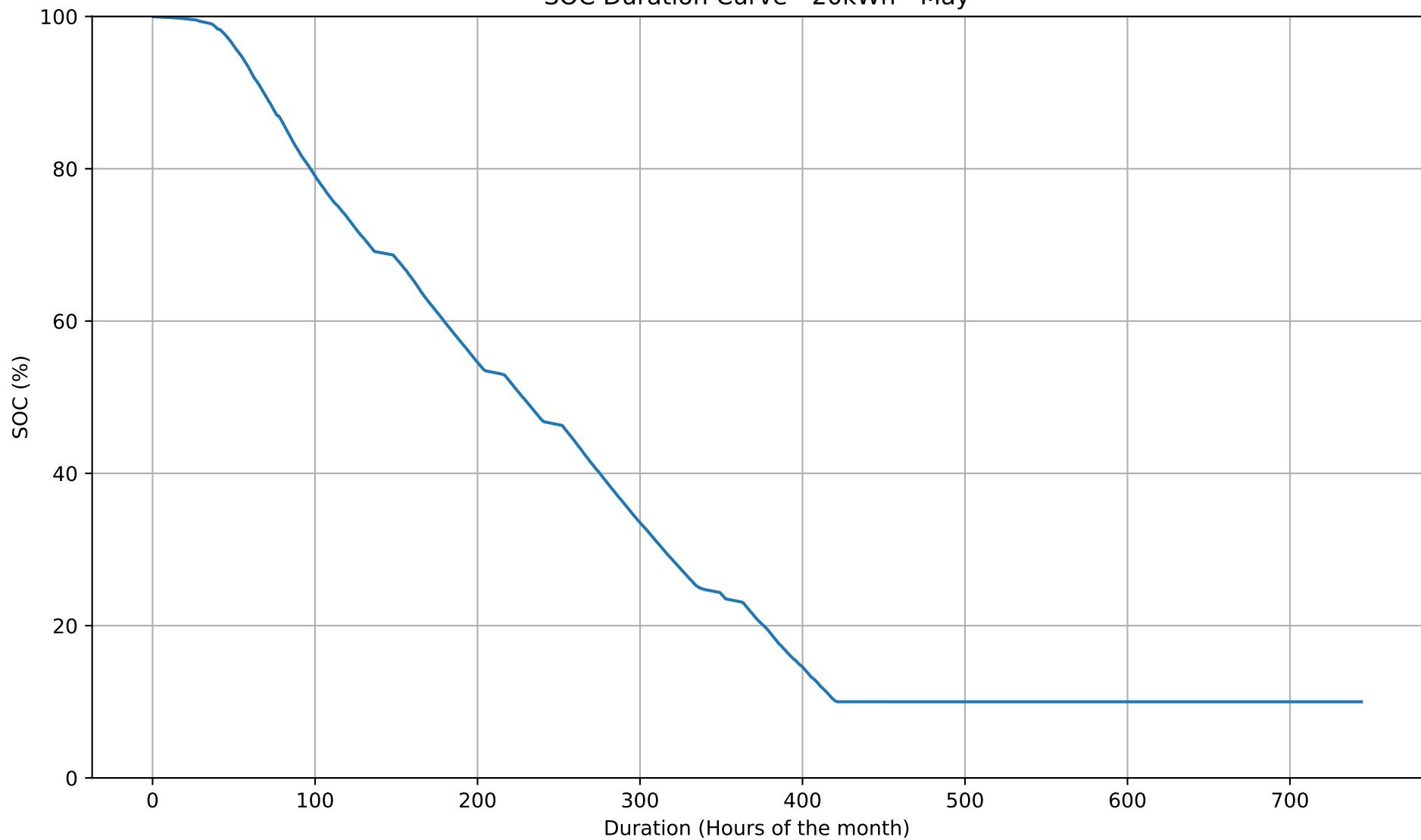
SOC Duration Curve - 20kWh - May
