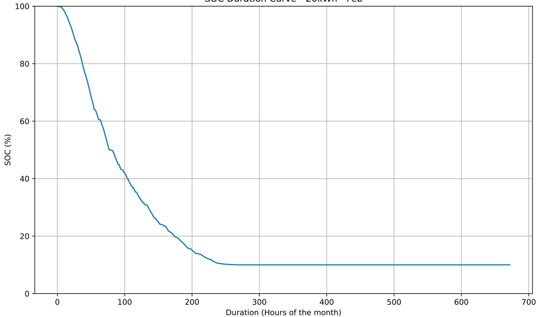
SOC Duration Curve - 20kWh - Feb
