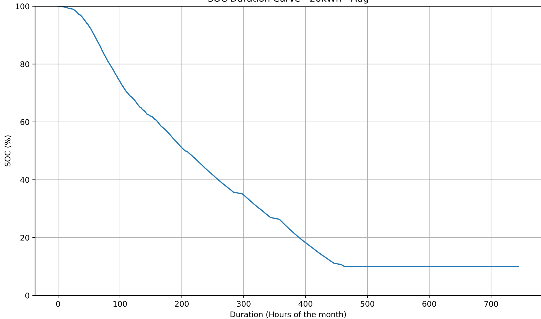
SOC Duration Curve - 20kWh - Aug
