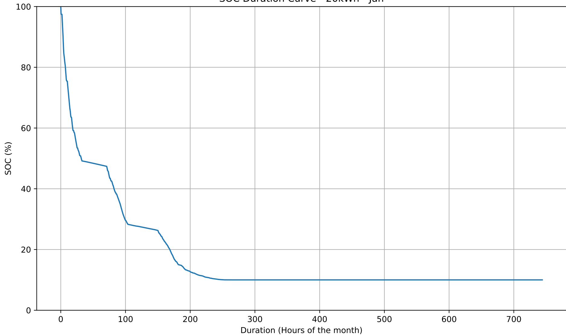
SOC Duration Curve - 20kWh - Jan
