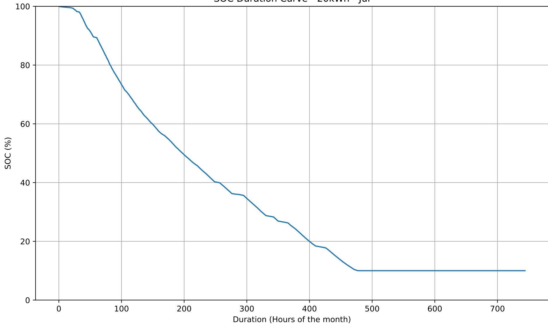
SOC Duration Curve - 20kWh - Jul
