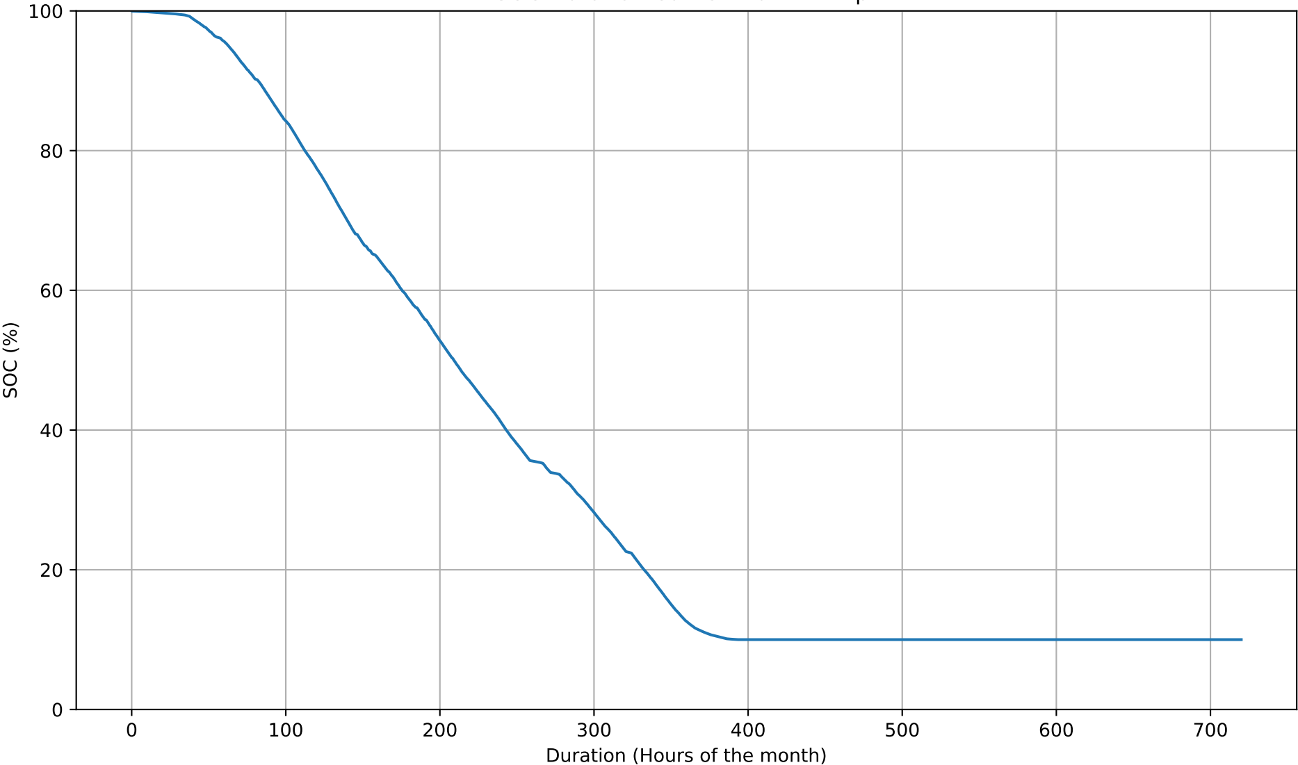
SOC Duration Curve - 20kWh - Apr
