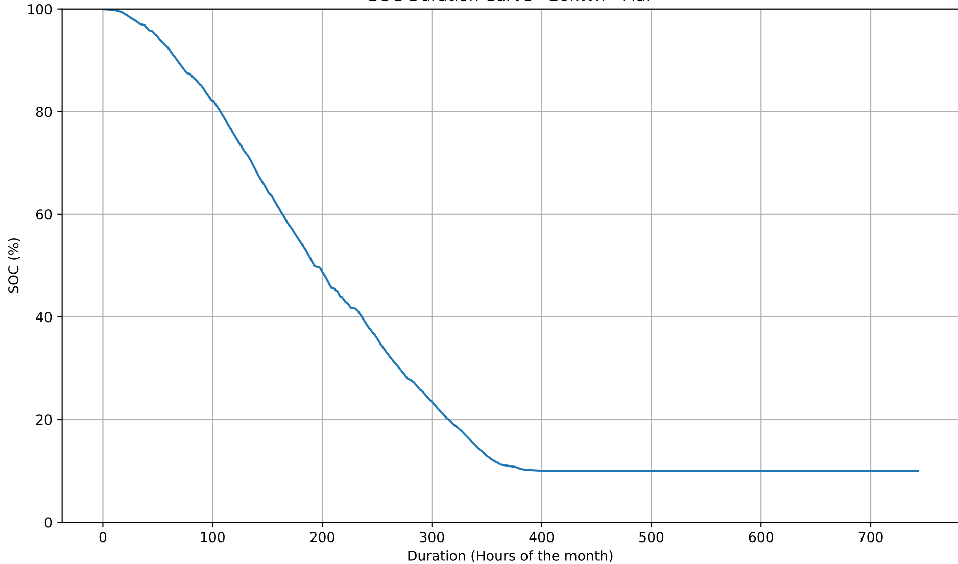
SOC Duration Curve - 20kWh - Mar
