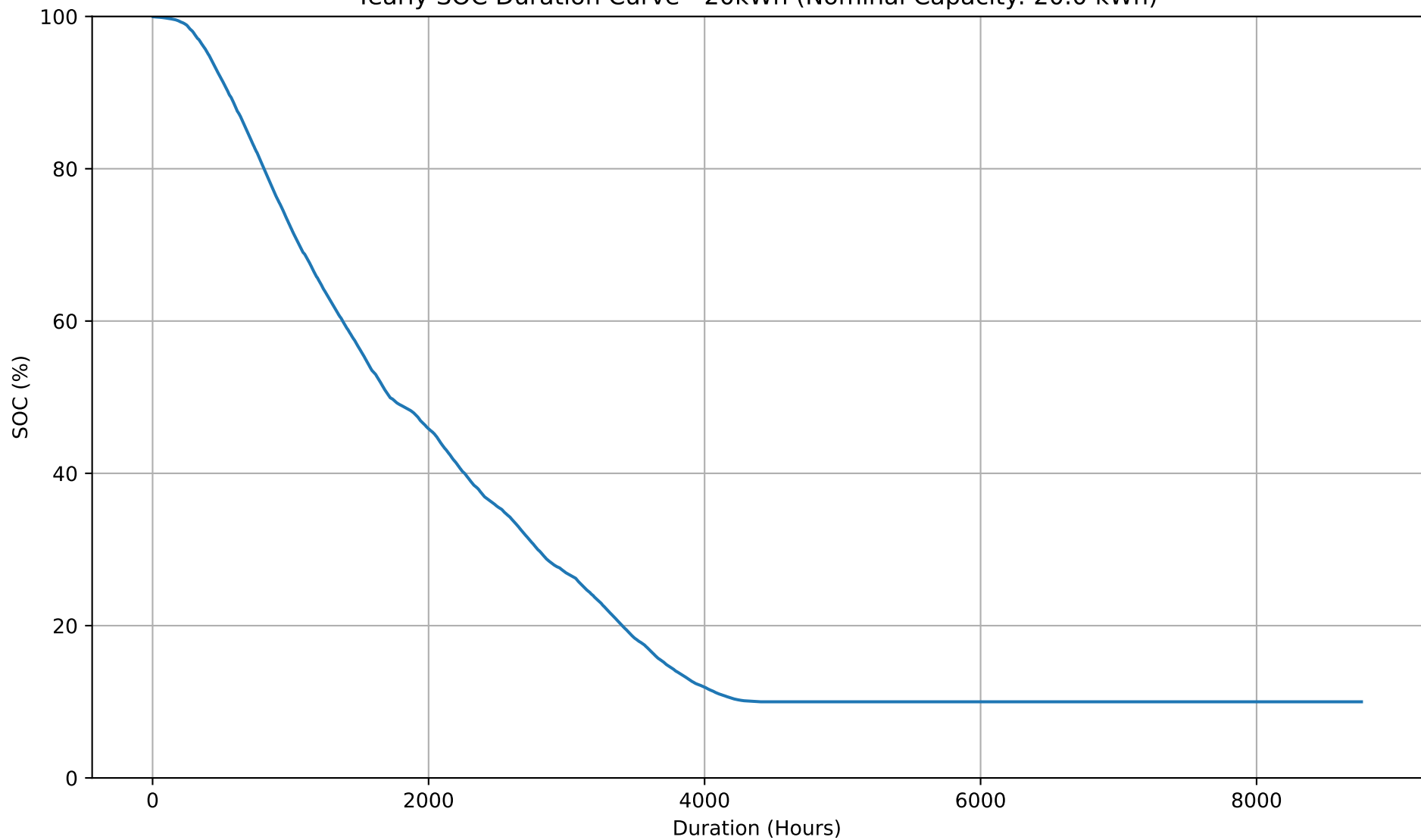
Yearly SOC Duration Curve - 20kWh (Nominal Capacity: 20.0 kWh)
