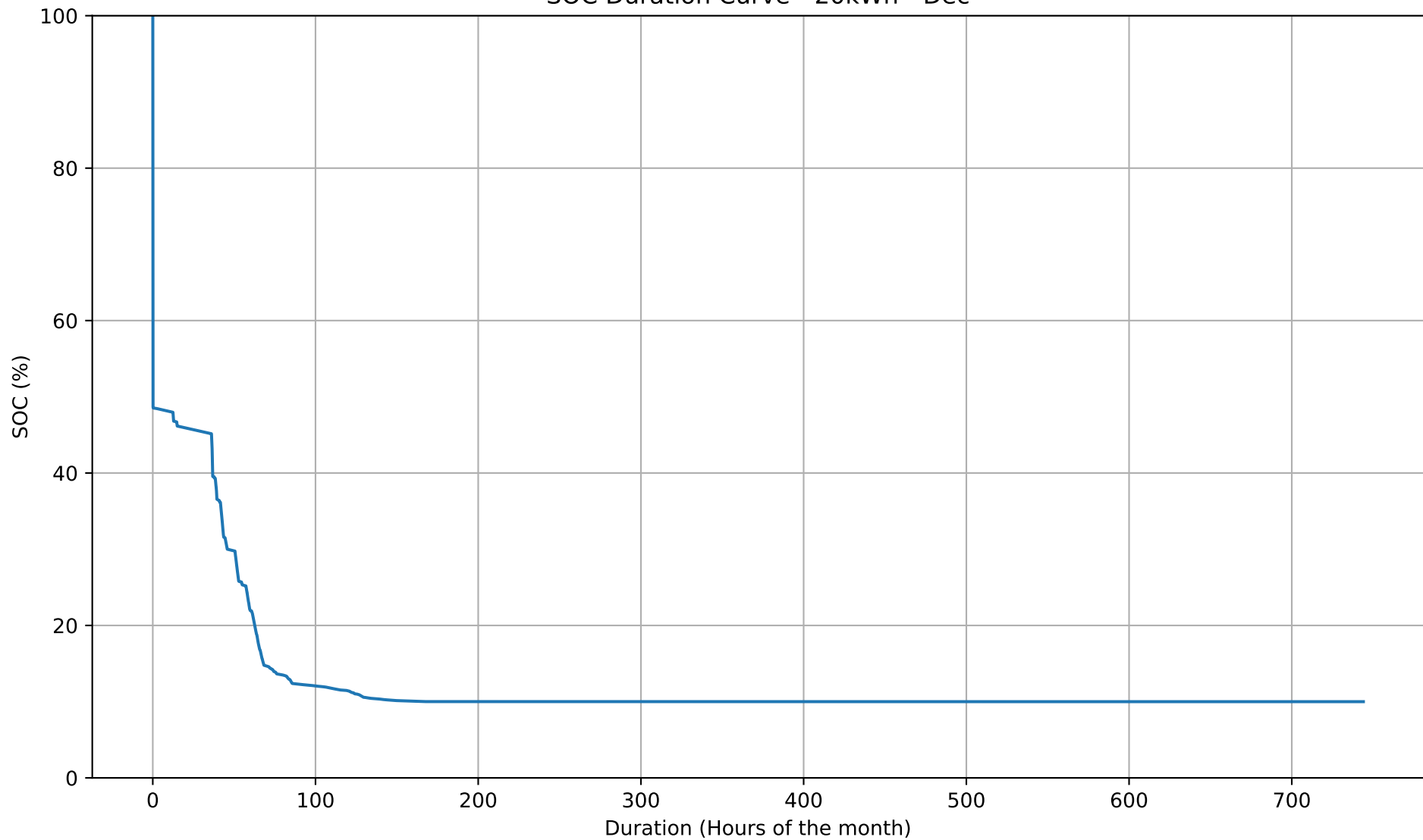
SOC Duration Curve - 20kWh - Dec
