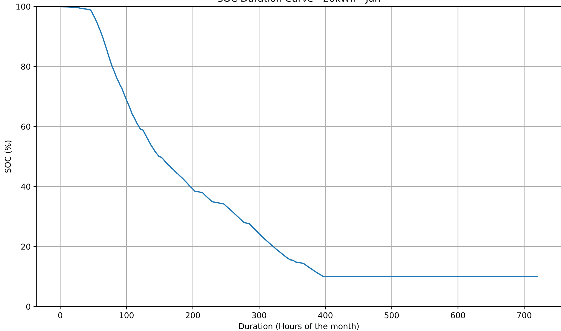
SOC Duration Curve - 20kWh - Jun
