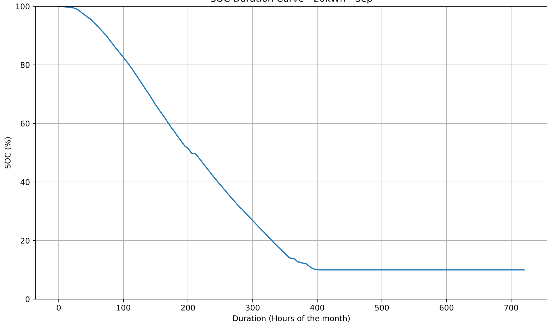
SOC Duration Curve - 20kWh - Sep
