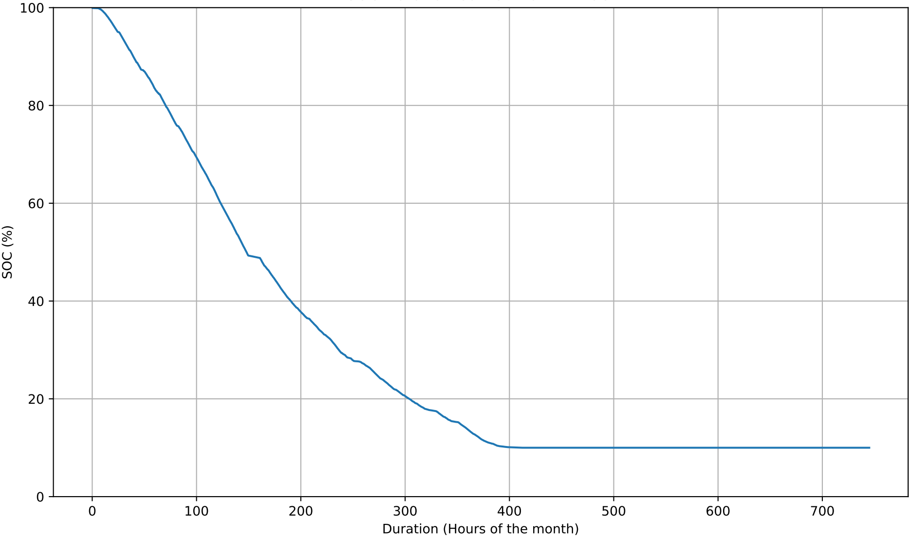
SOC Duration Curve - 20kWh - Oct
