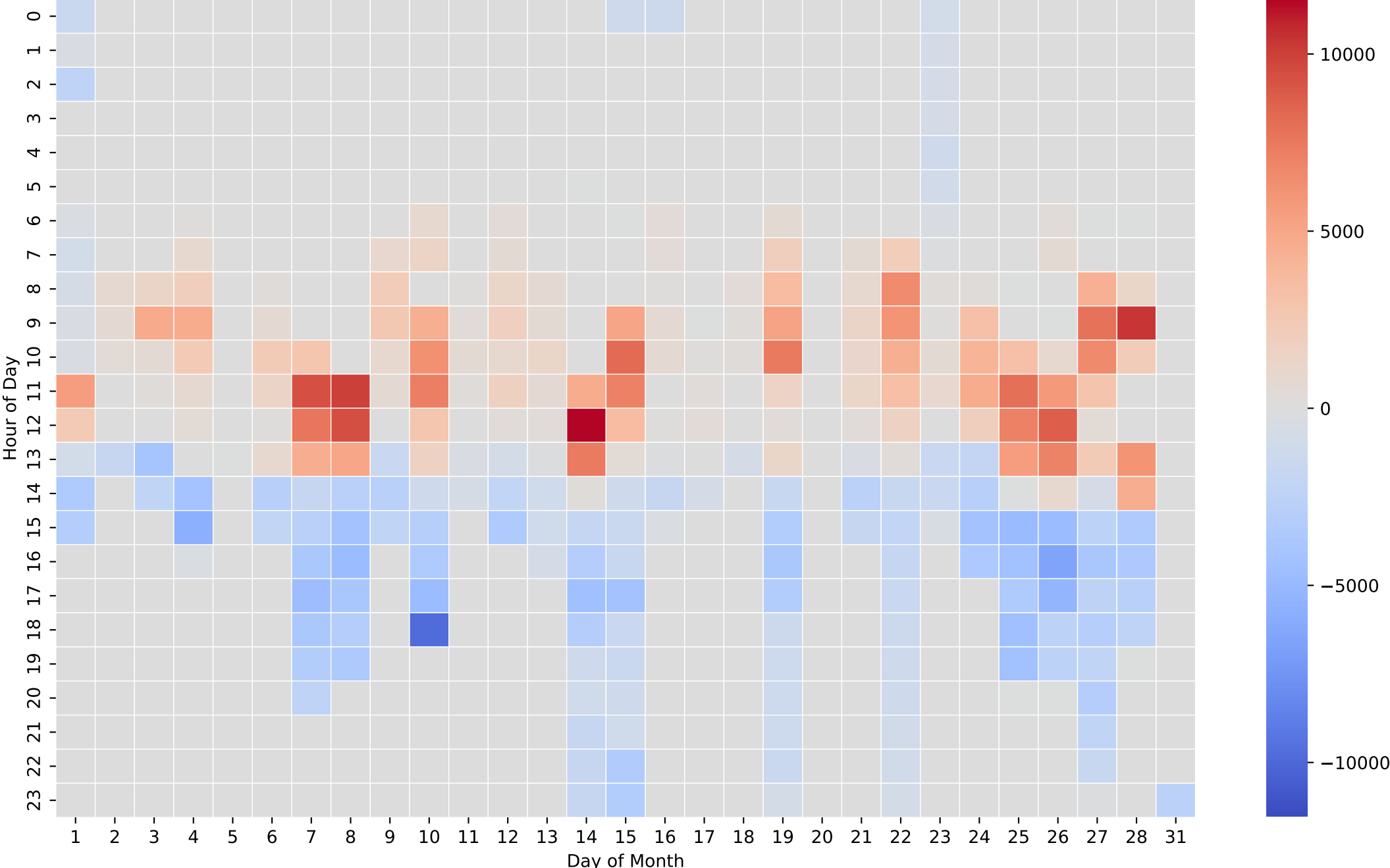
Battery Net Power Heatmap (Wh/Hour) - 26kWh - Feb
