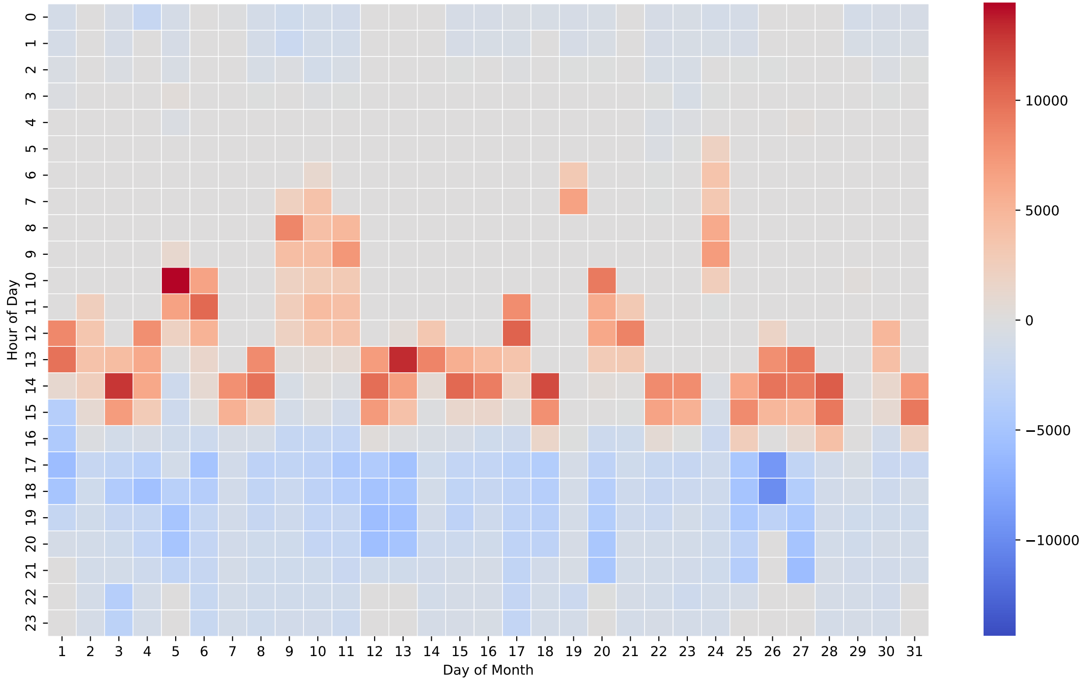
Battery Net Power Heatmap (Wh/Hour) - 26kWh - May
