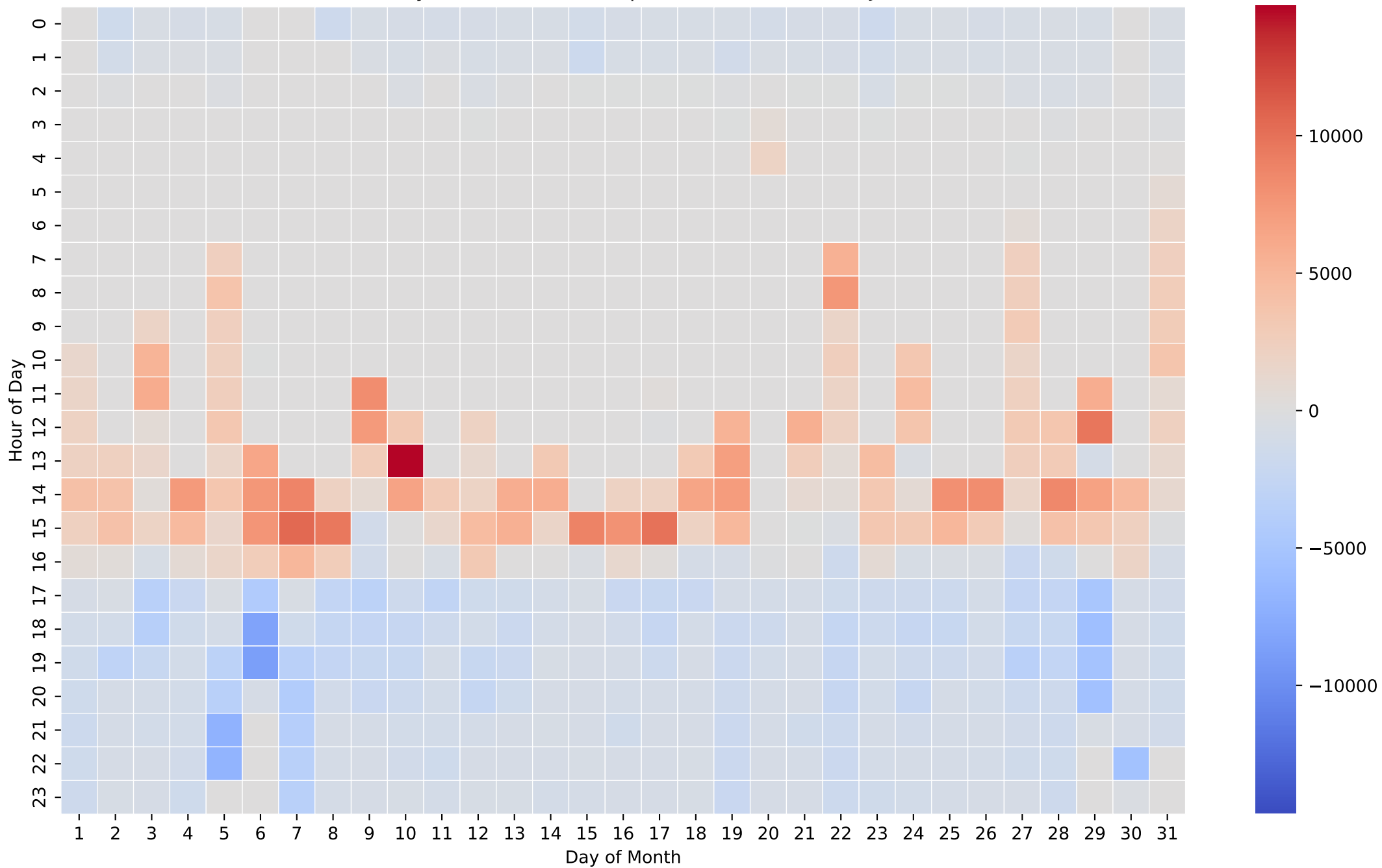
Battery Net Power Heatmap (Wh/Hour) - 26kWh - Jul
