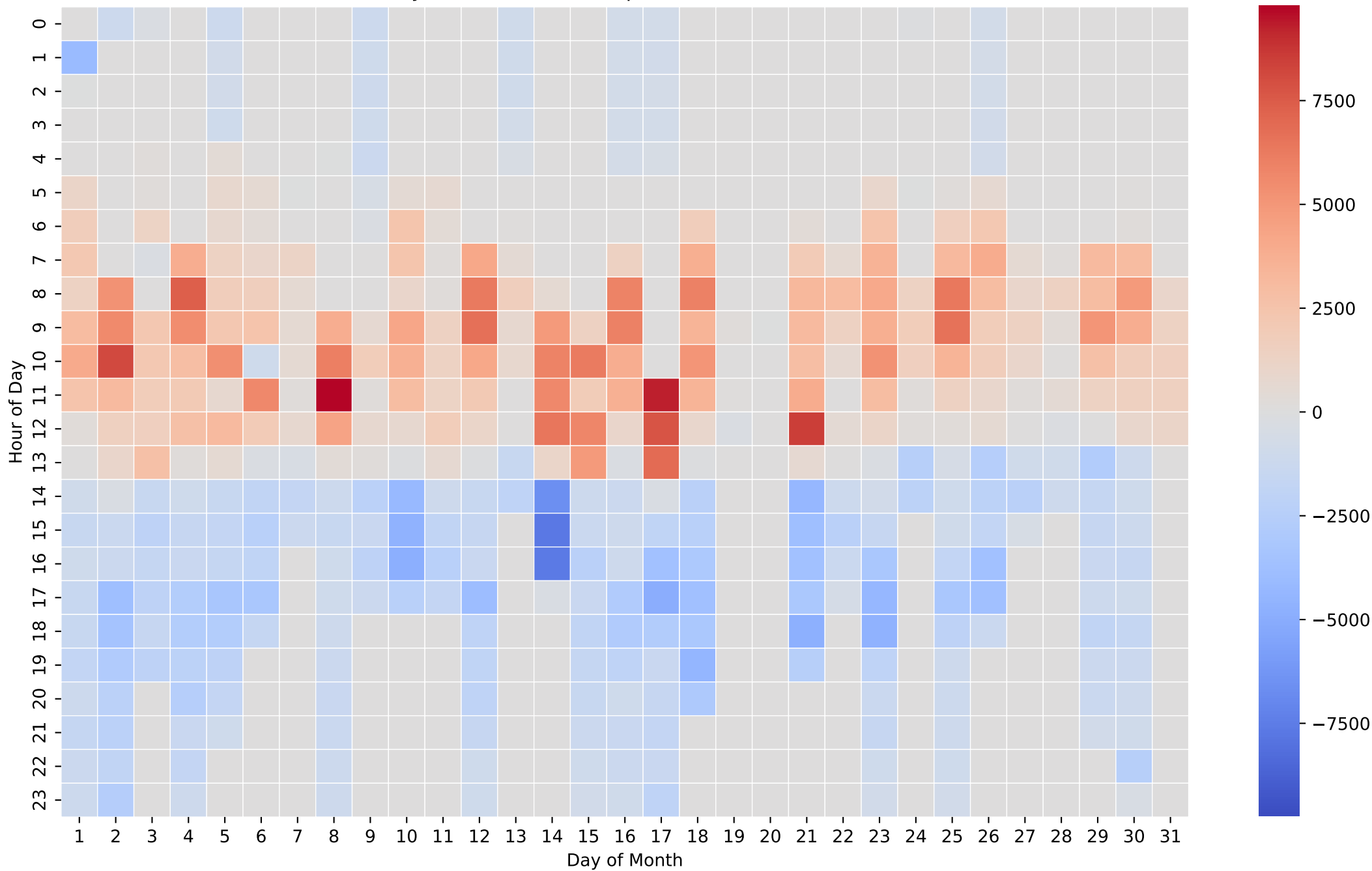
Battery Net Power Heatmap (Wh/Hour) - 26kWh - Oct
