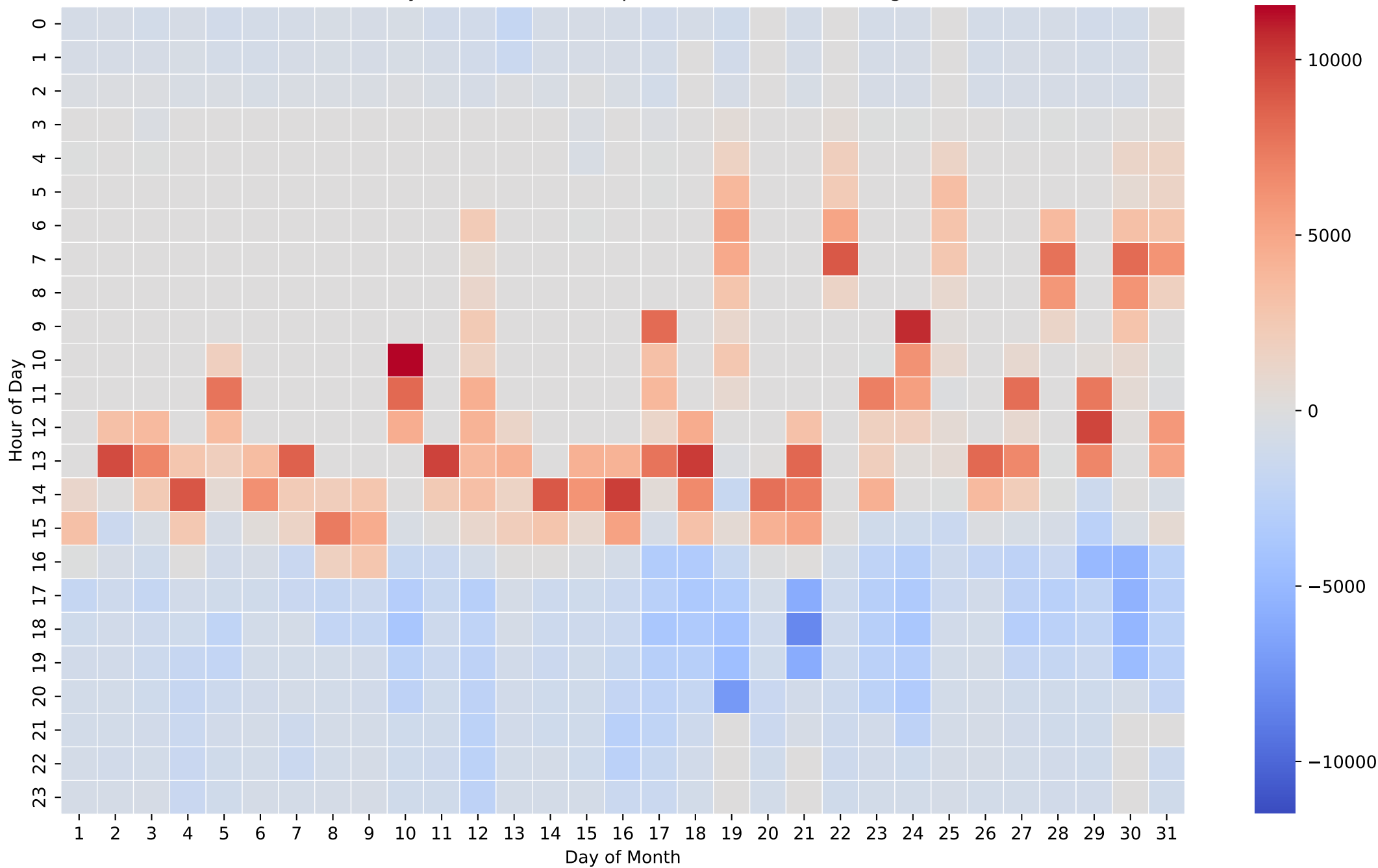
Battery Net Power Heatmap (Wh/Hour) - 26kWh - Aug
