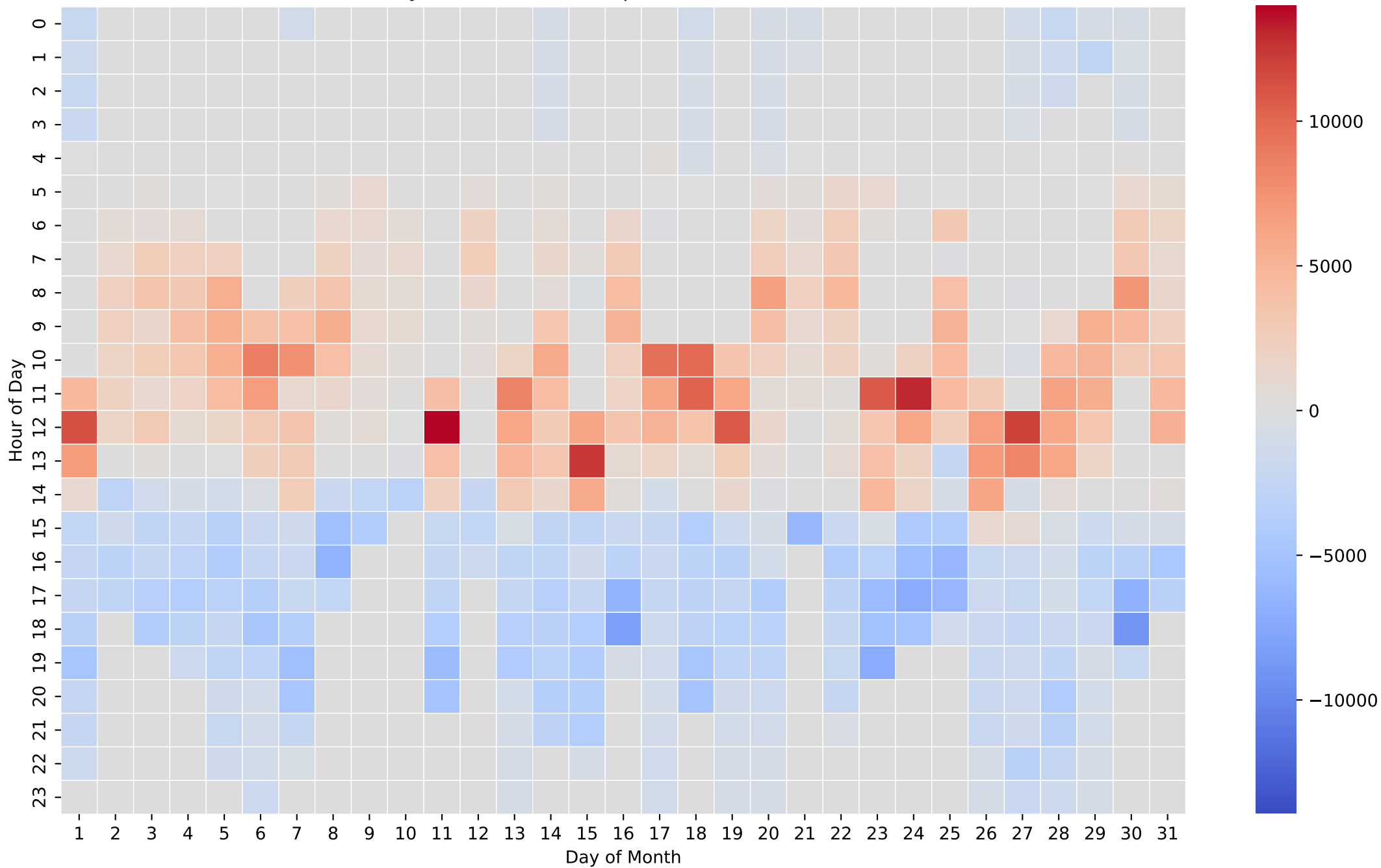
Battery Net Power Heatmap (Wh/Hour) - 26kWh - Mar
