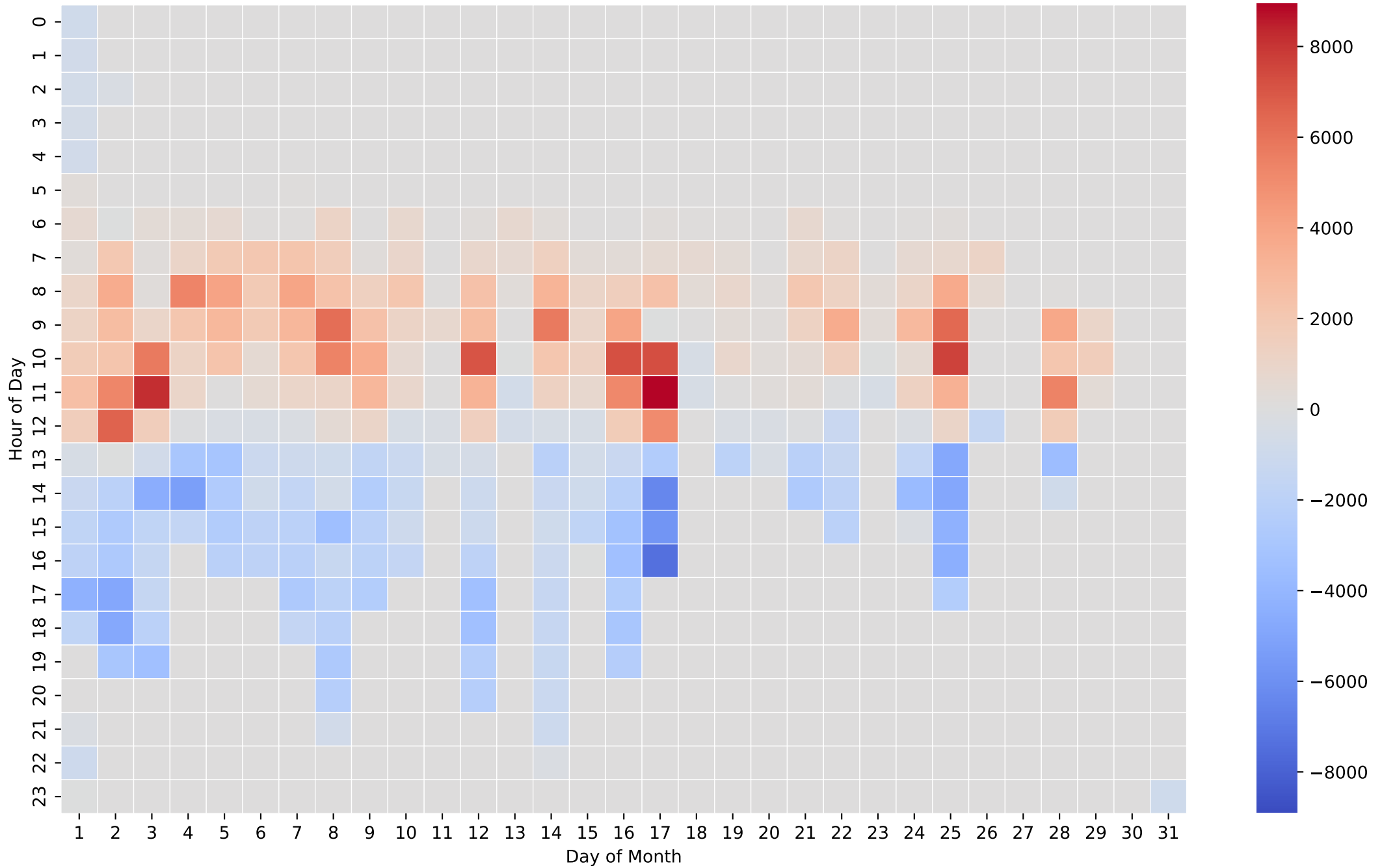
Battery Net Power Heatmap (Wh/Hour) - 26kWh - Nov
