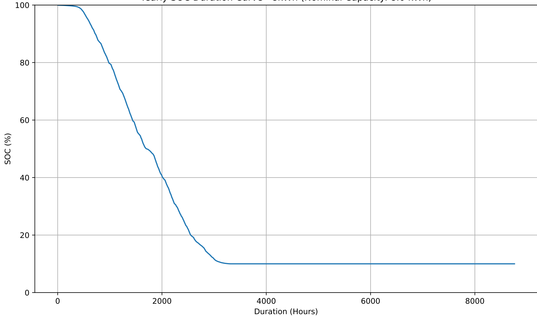
Yearly SOC Duration Curve - 8kWh (Nominal Capacity: 8.0 kWh)
