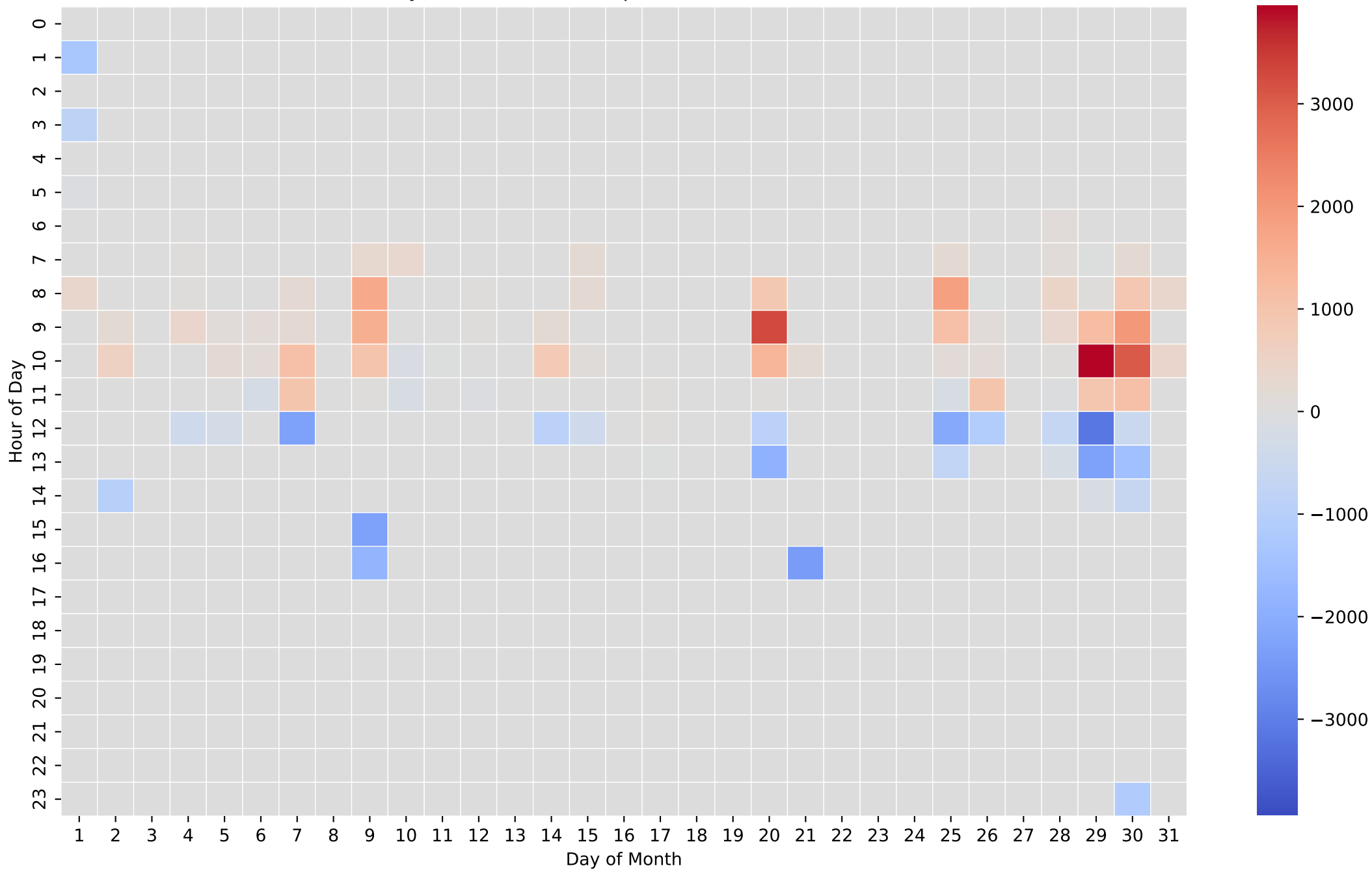
Battery Net Power Heatmap (Wh/Hour) - 12kWh - Dec
