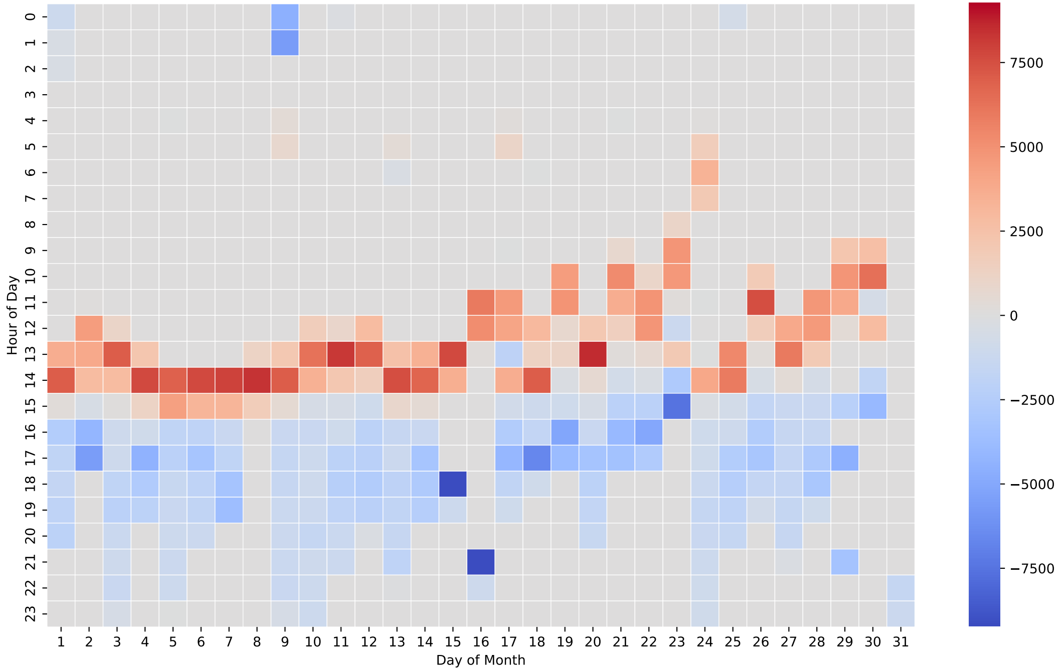
Battery Net Power Heatmap (Wh/Hour) - 12kWh - Sep
