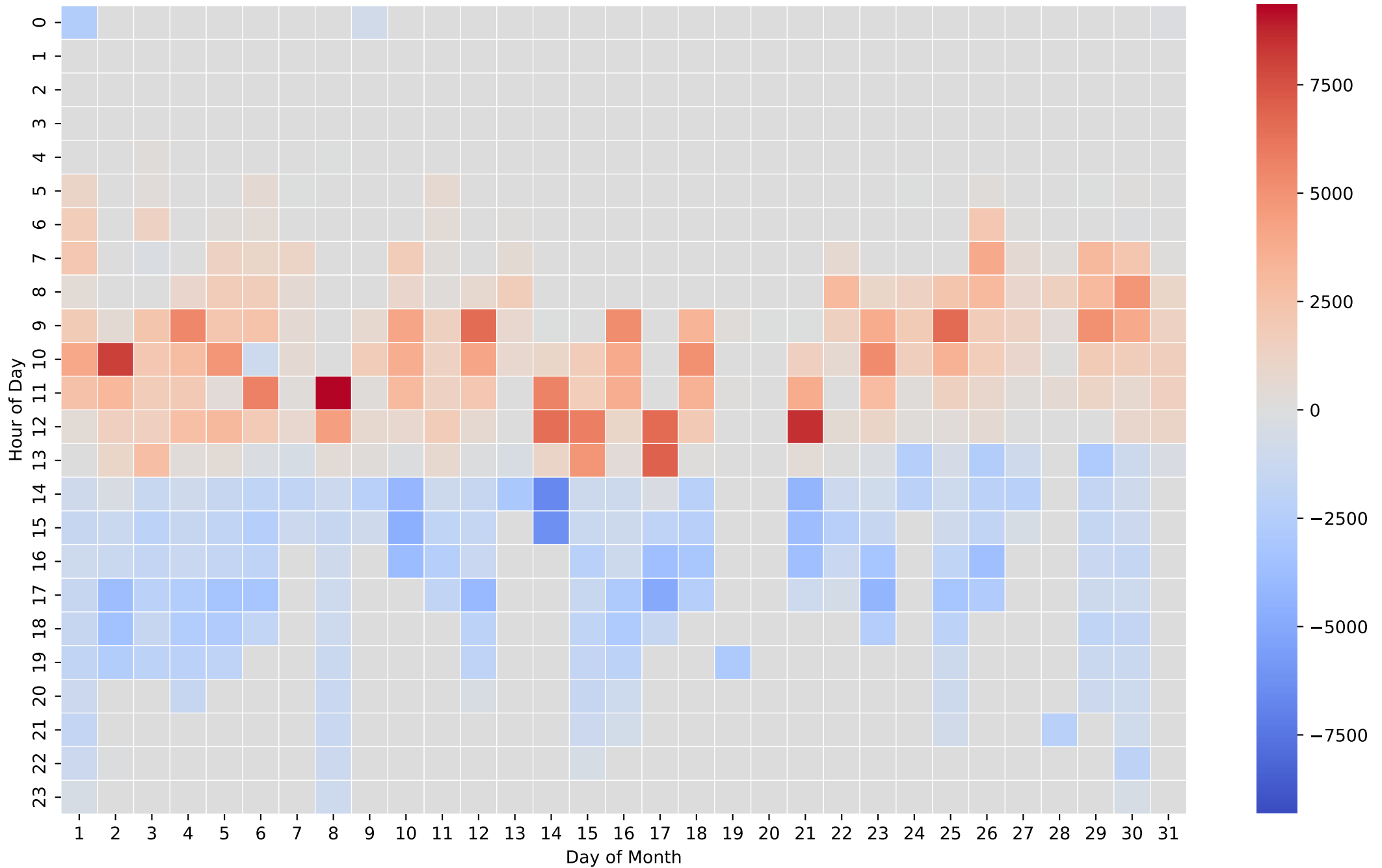
Battery Net Power Heatmap (Wh/Hour) - 15kWh - Oct
