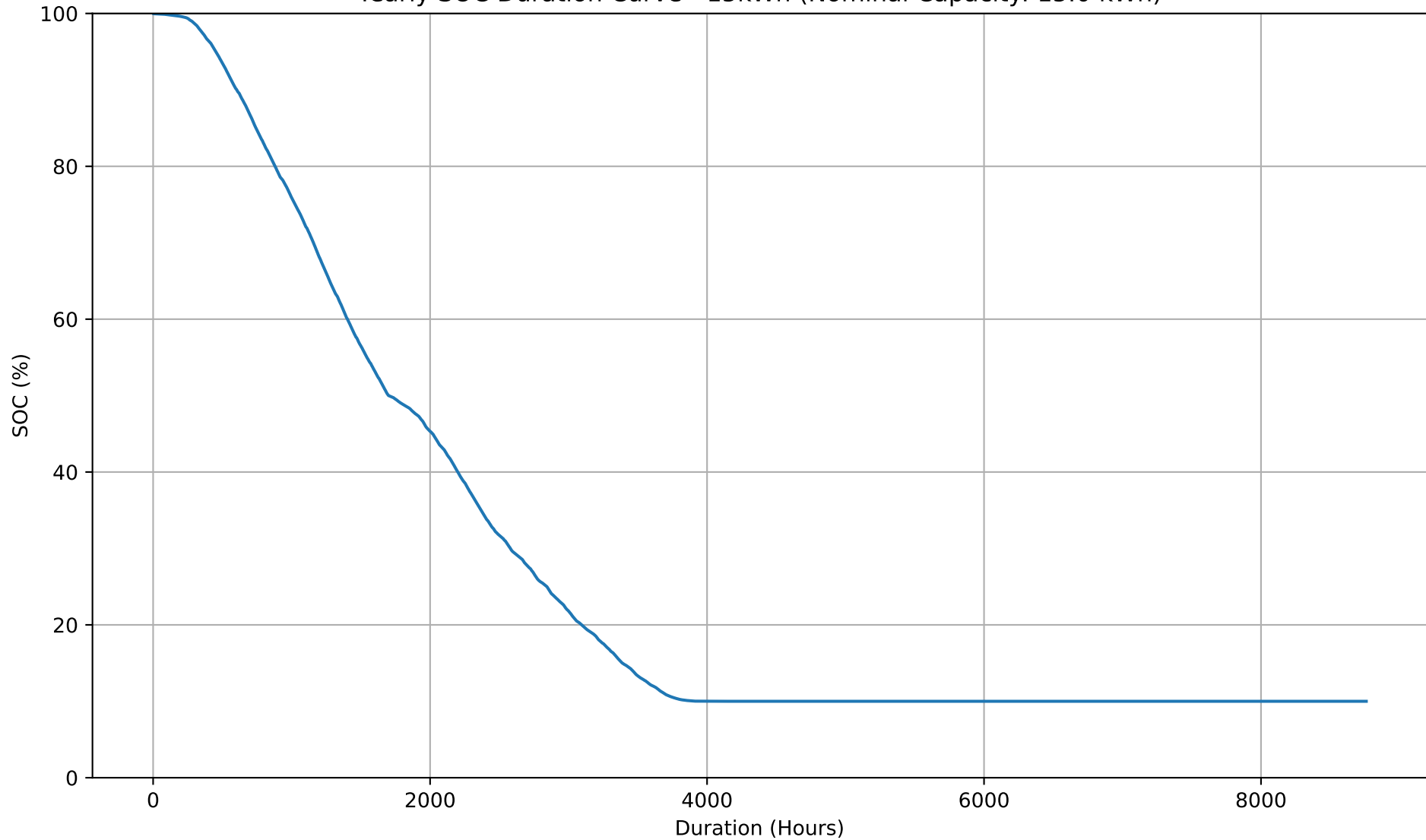
Yearly SOC Duration Curve - 15kWh (Nominal Capacity: 15.0 kWh)
