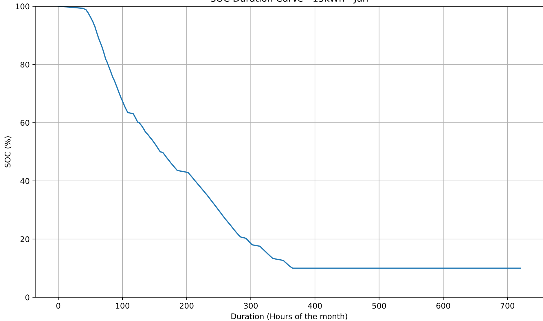
SOC Duration Curve - 15kWh - Jun
