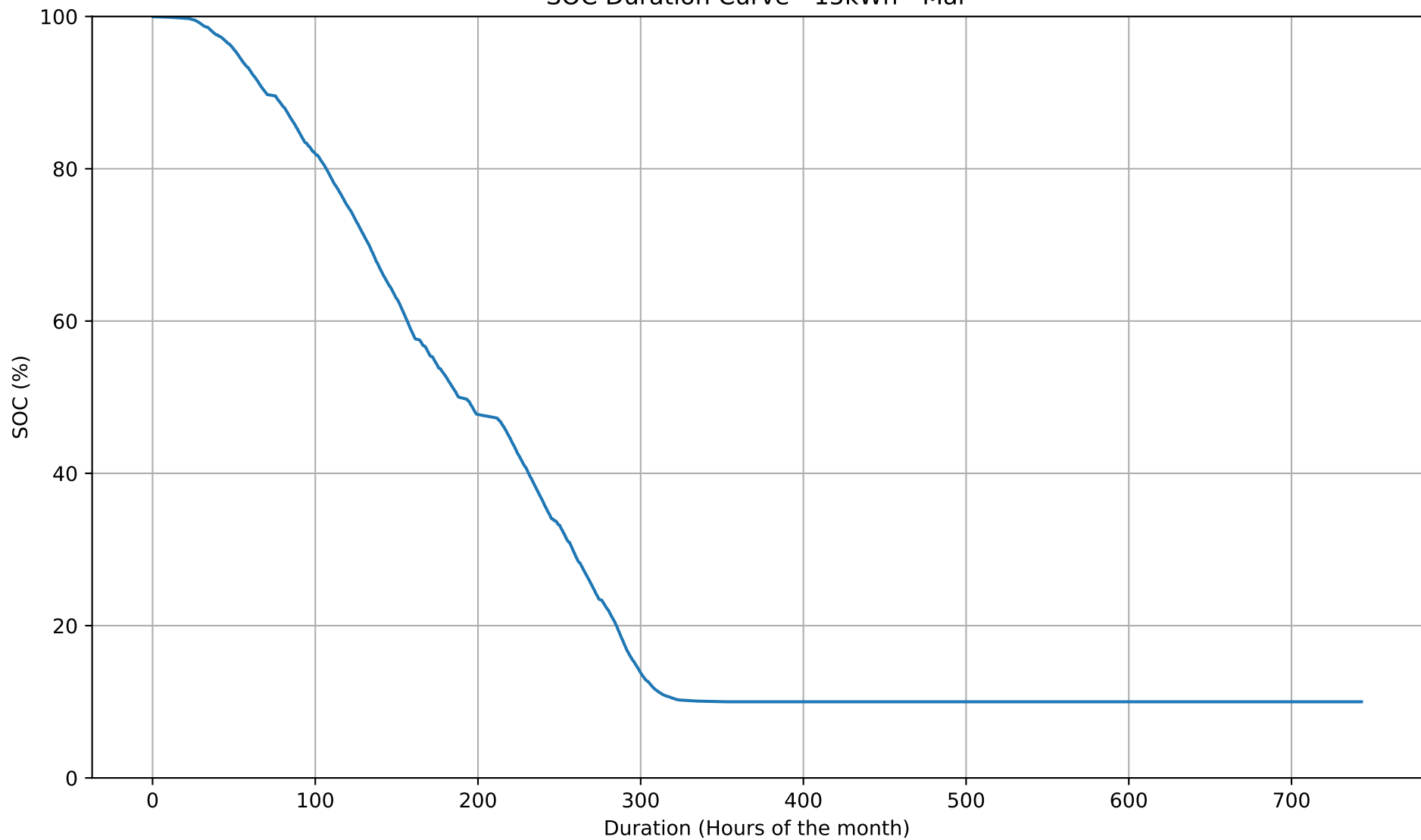
SOC Duration Curve - 15kWh - Mar
