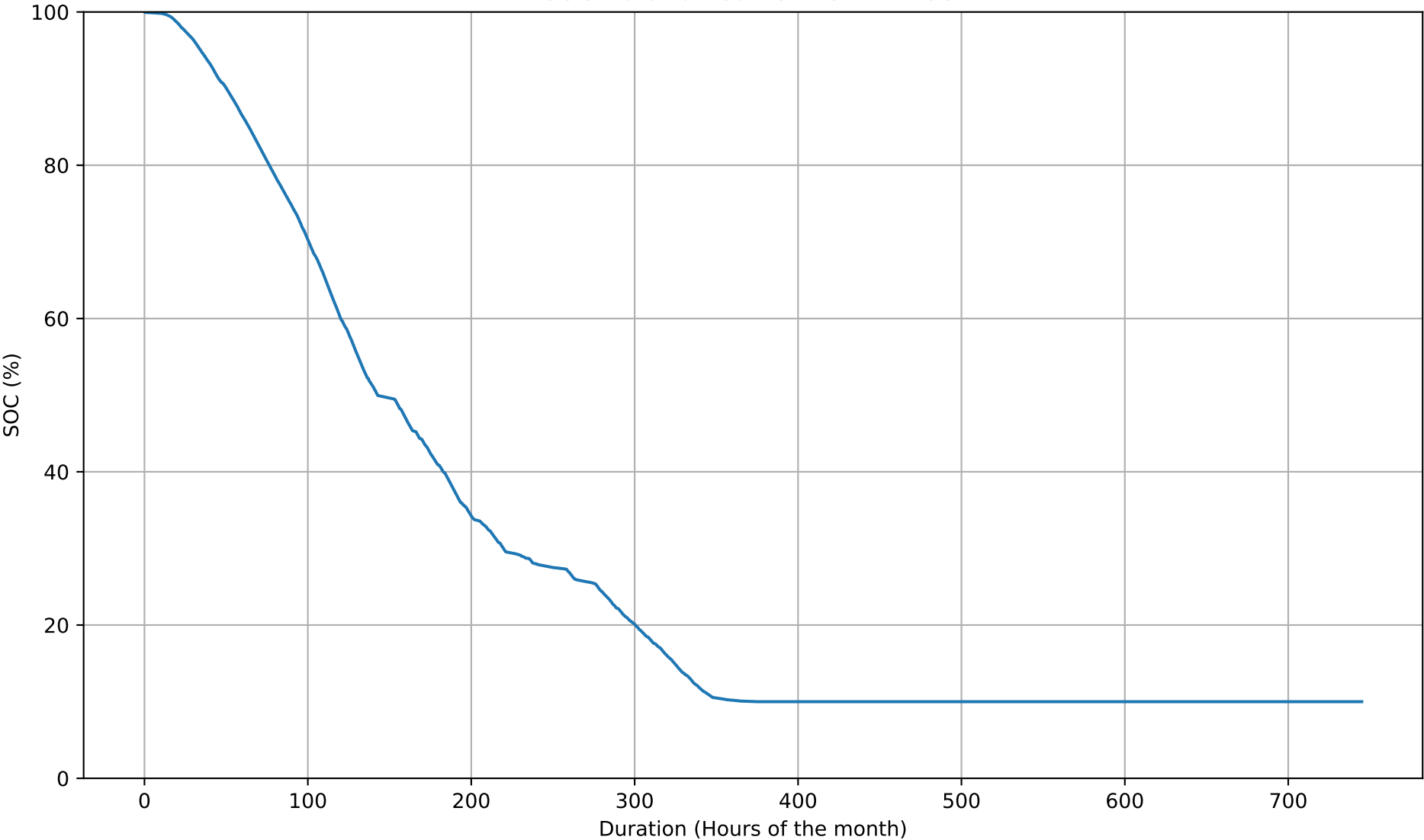
SOC Duration Curve - 15kWh - Oct
