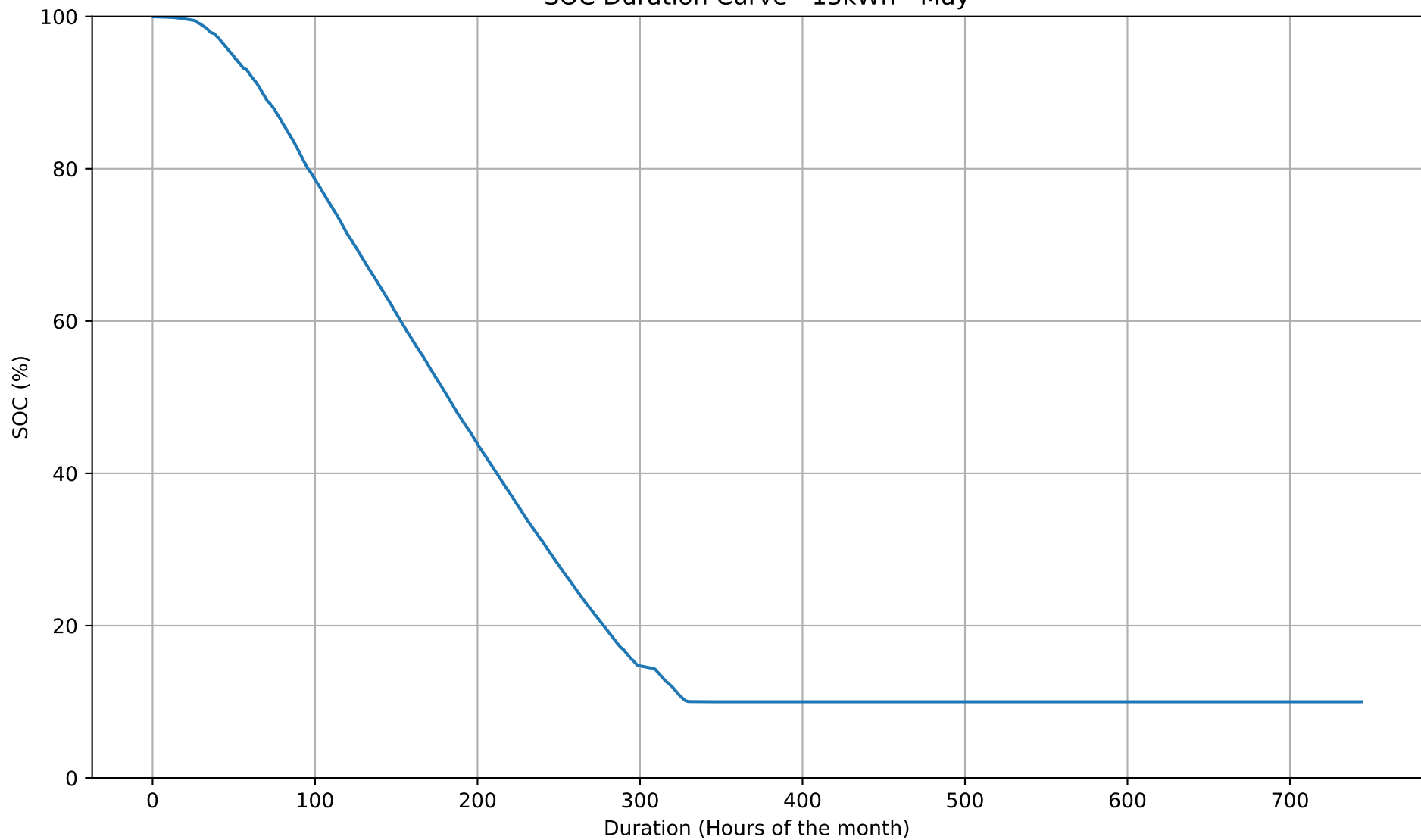
SOC Duration Curve - 15kWh - May
