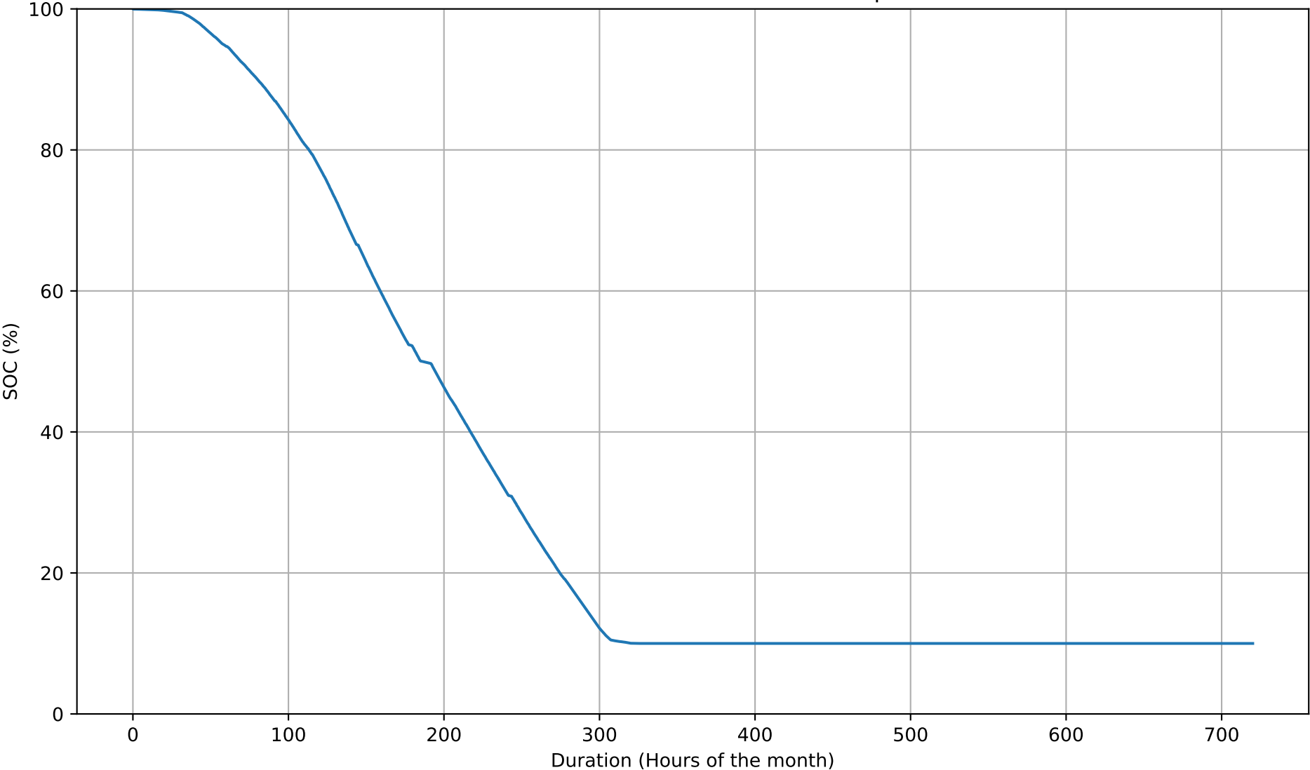
SOC Duration Curve - 15kWh - Sep
