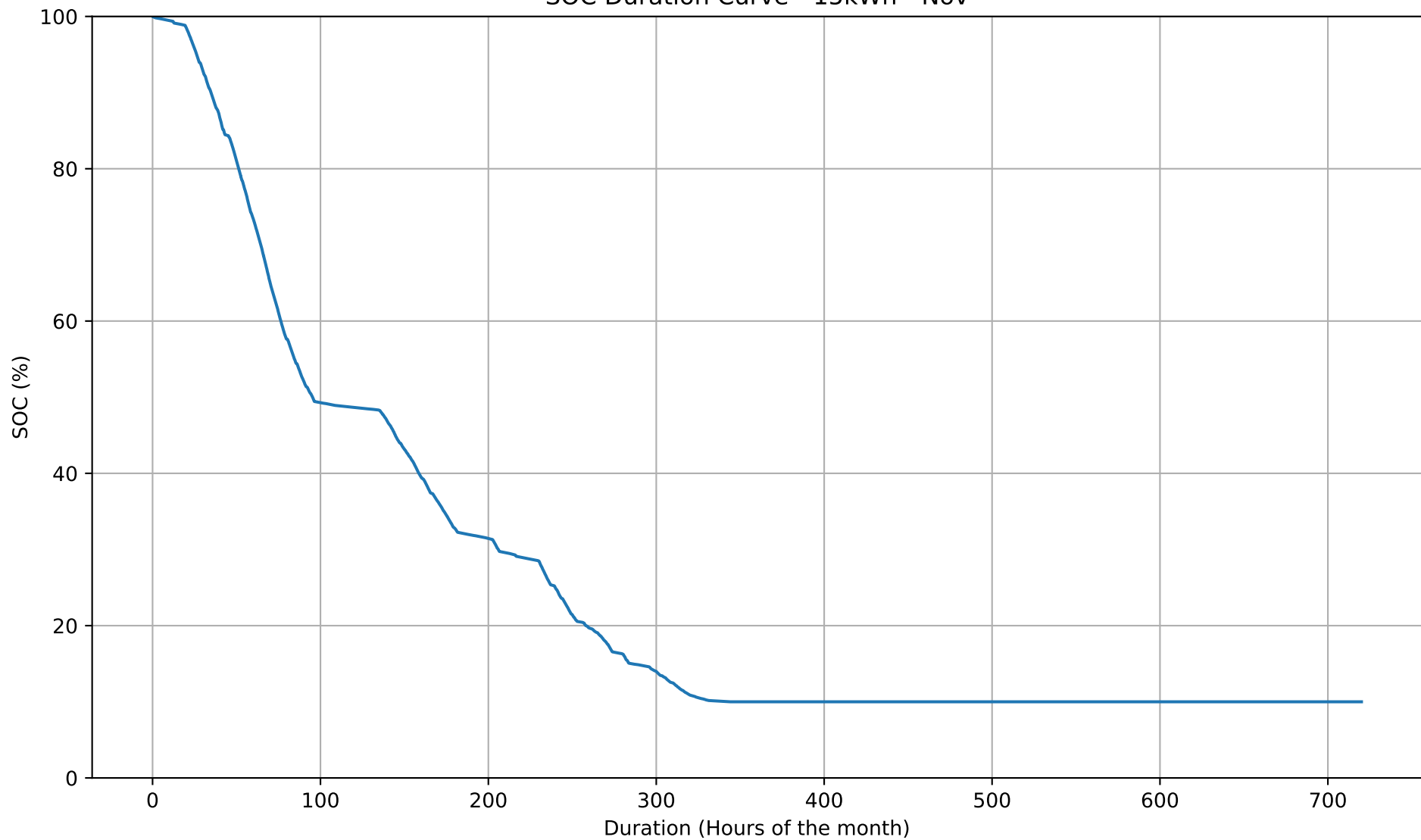
SOC Duration Curve - 15kWh - Nov
