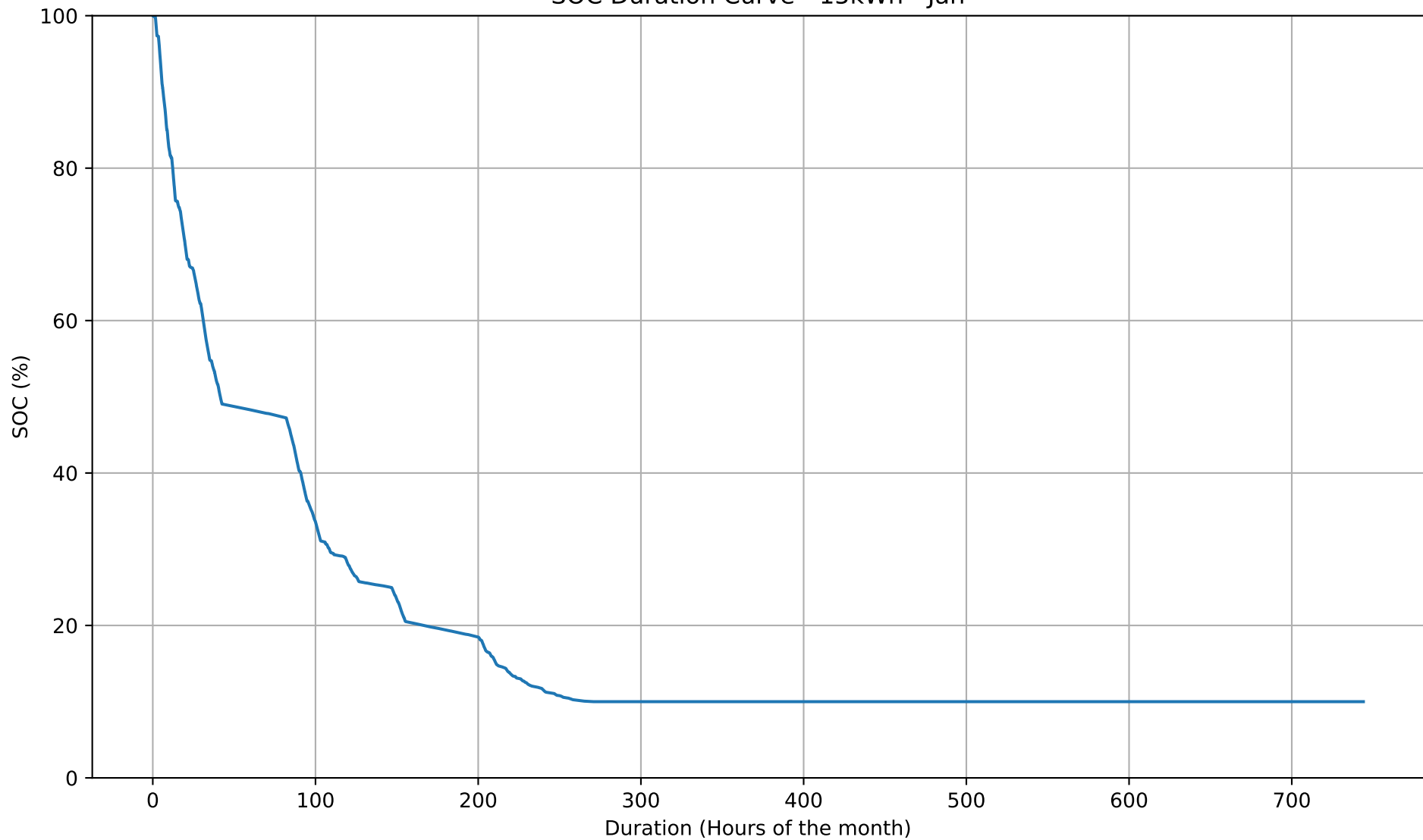
SOC Duration Curve - 15kWh - Jan
