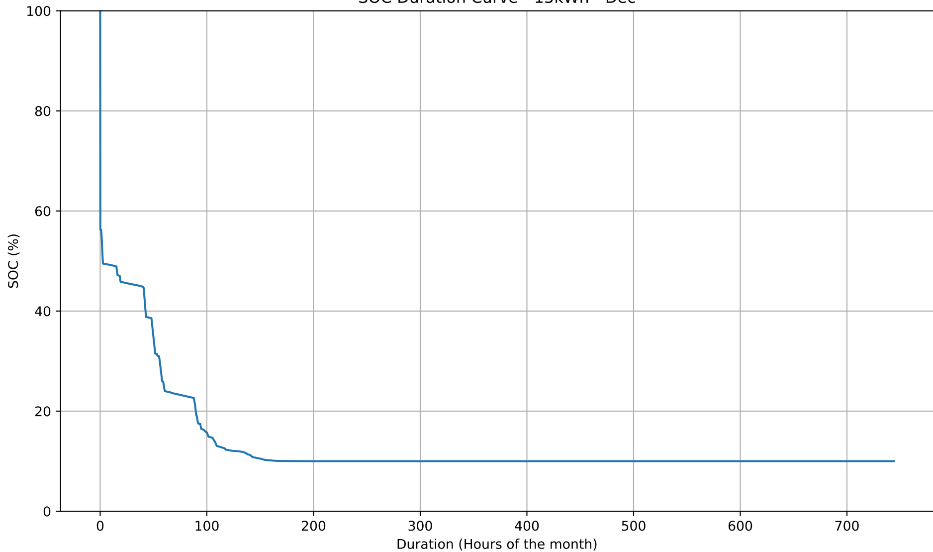
SOC Duration Curve - 15kWh - Dec
