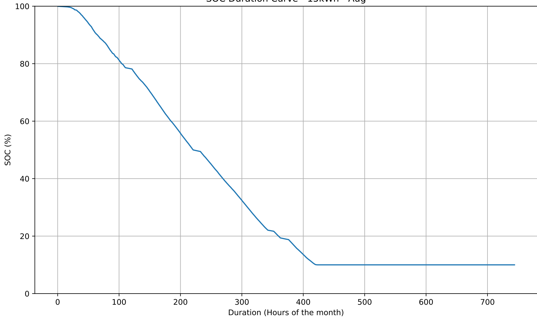
SOC Duration Curve - 15kWh - Aug
