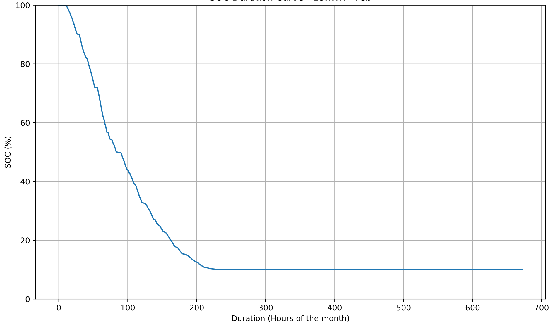
SOC Duration Curve - 15kWh - Feb
