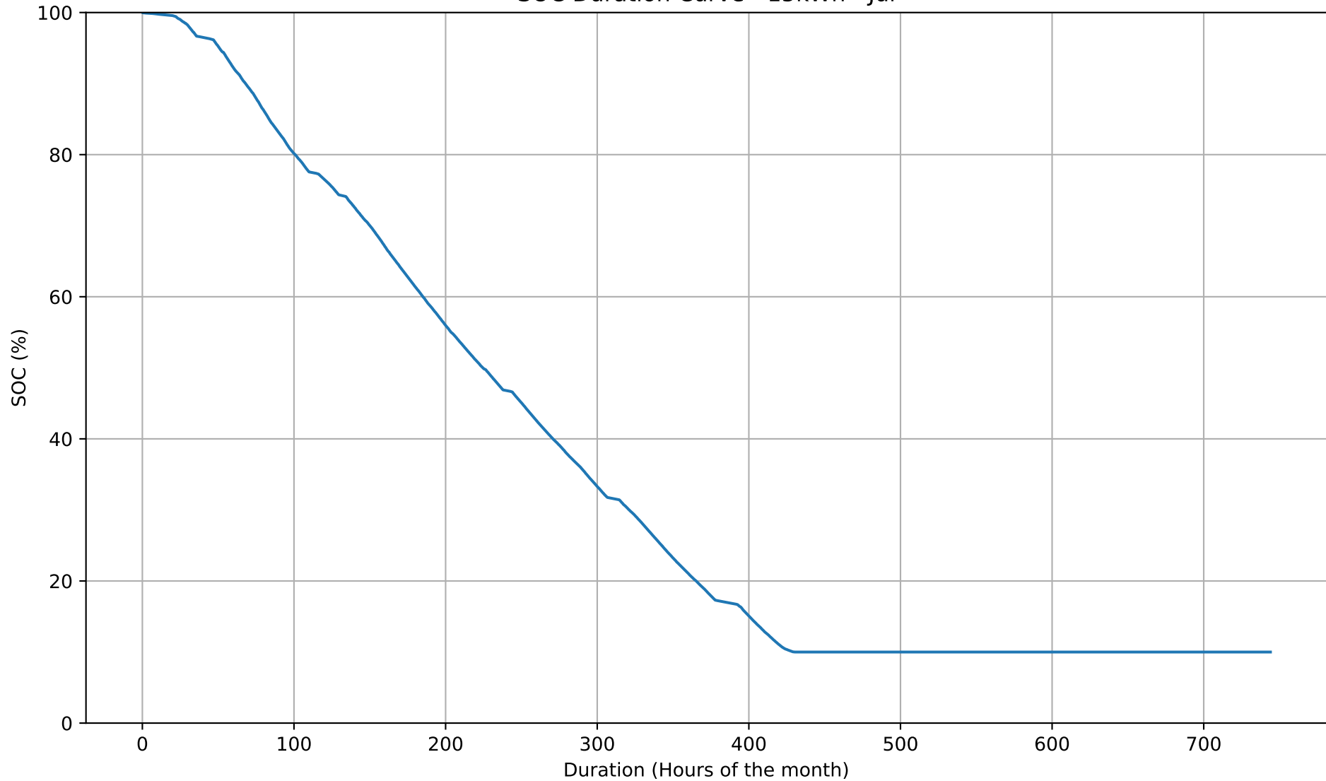
SOC Duration Curve - 15kWh - Jul
