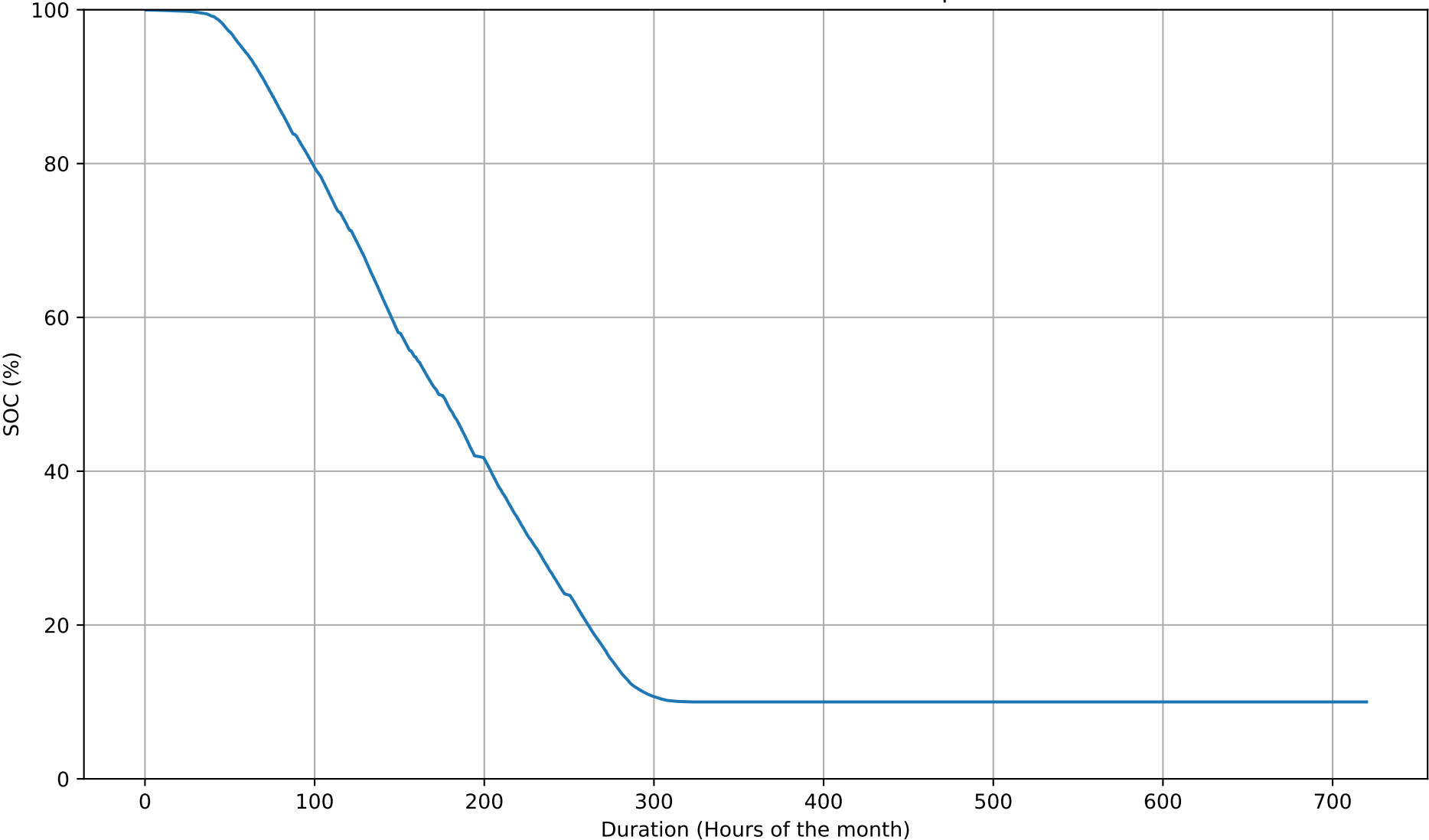
SOC Duration Curve - 15kWh - Apr
