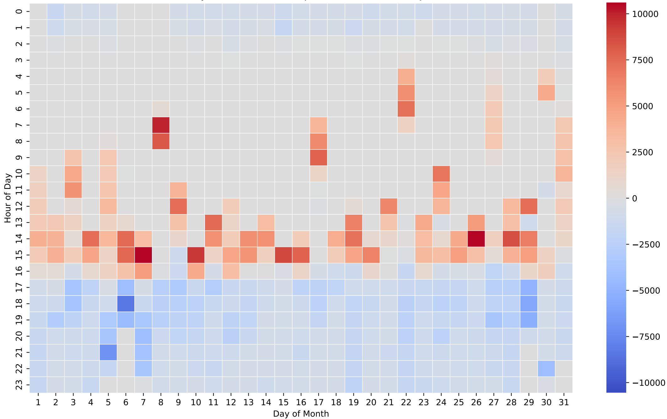
Battery Net Power Heatmap (Wh/Hour) - 20kWh - Jul
