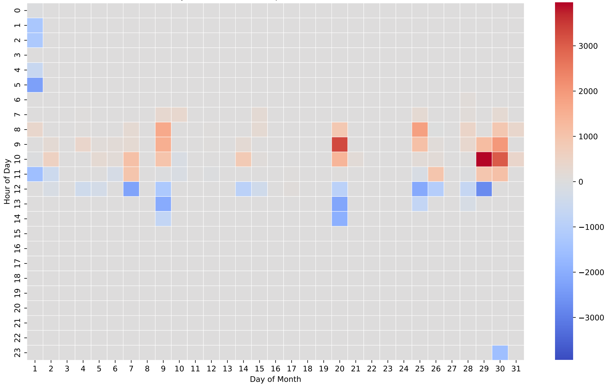
Battery Net Power Heatmap (Wh/Hour) - 26kWh - Dec
