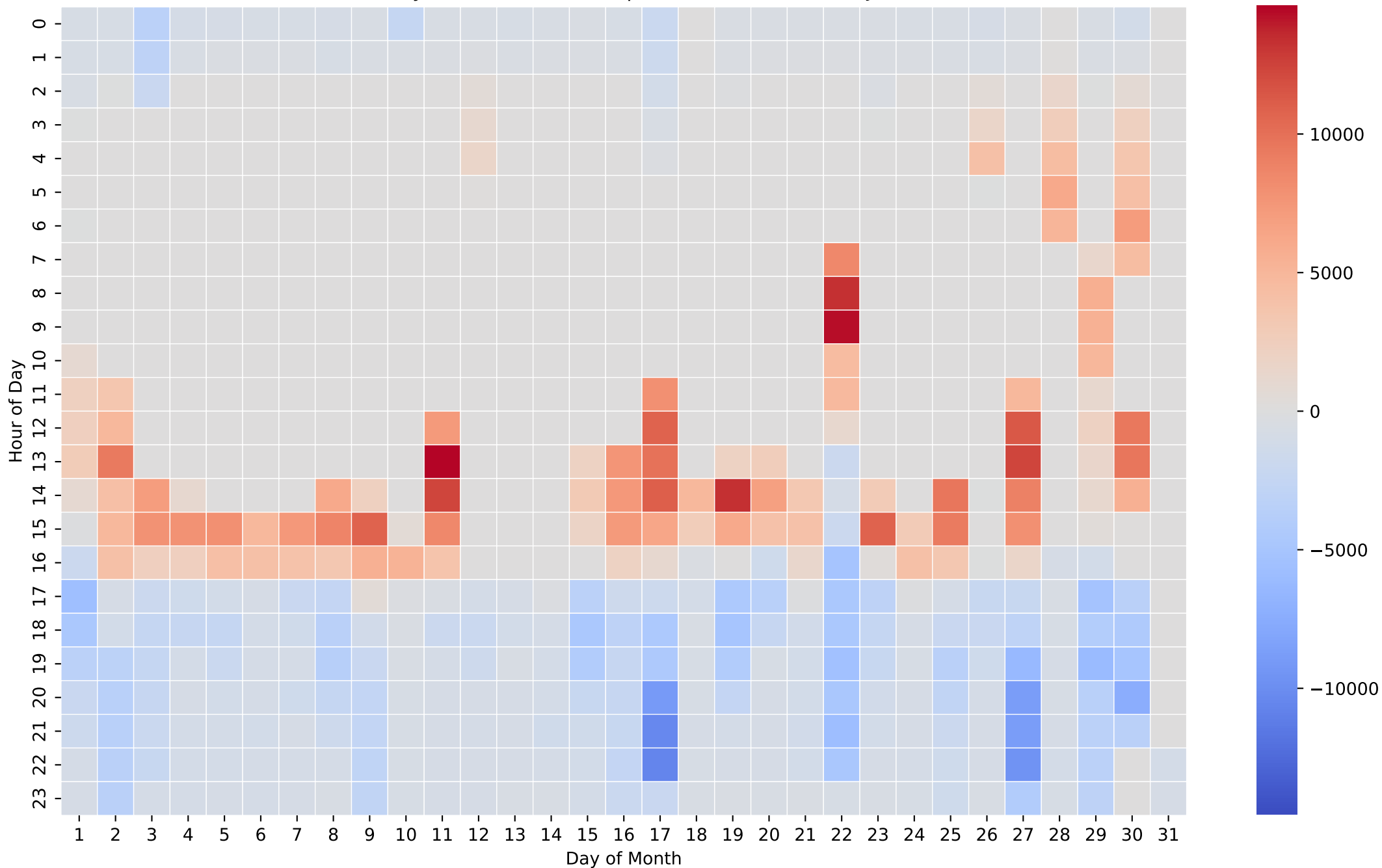
Battery Net Power Heatmap (Wh/Hour) - 50kWh - Jun
