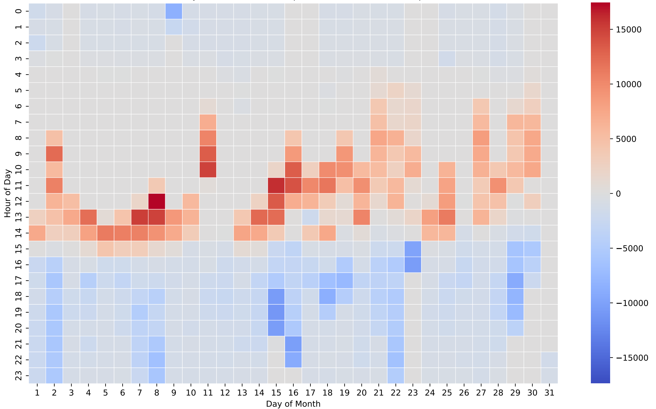
Battery Net Power Heatmap (Wh/Hour) - 50kWh - Sep
