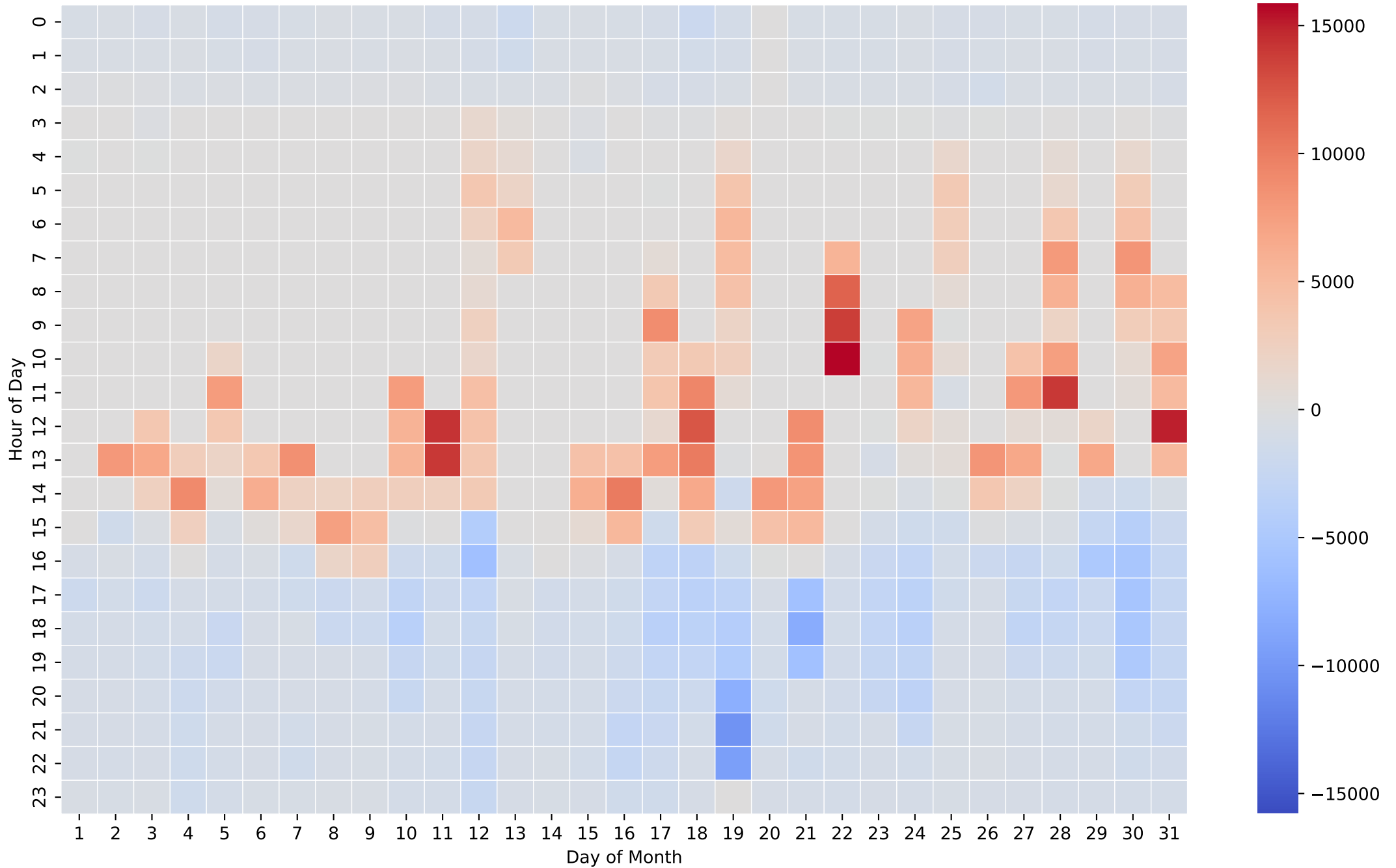
Battery Net Power Heatmap (Wh/Hour) - 50kWh - Aug
