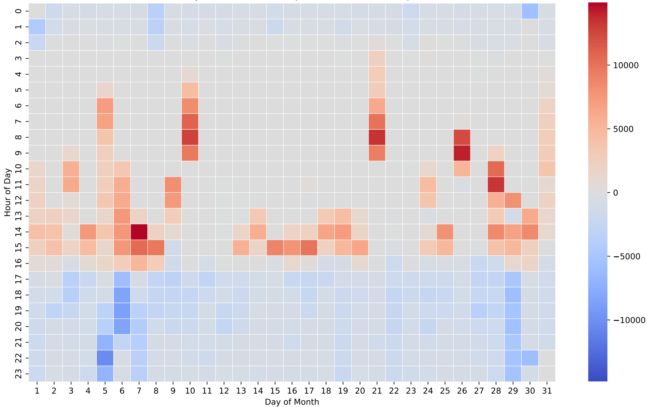
Battery Net Power Heatmap (Wh/Hour) - 50kWh - Jul
