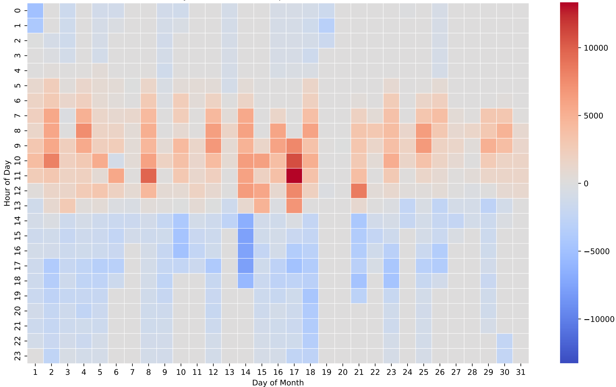
Battery Net Power Heatmap (Wh/Hour) - 50kWh - Oct
