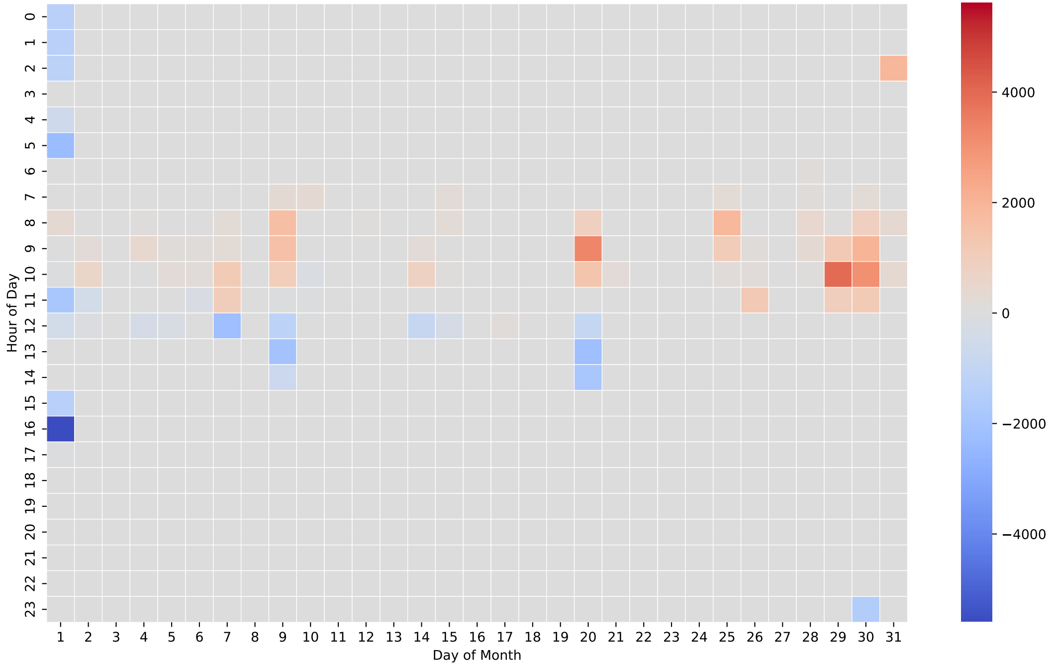
Battery Net Power Heatmap (Wh/Hour) - 50kWh - Dec
