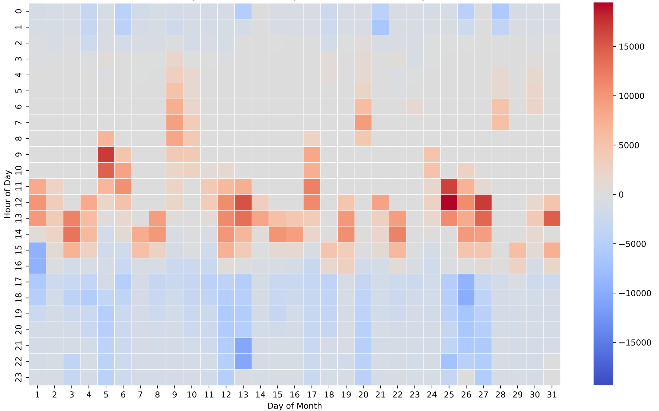
Battery Net Power Heatmap (Wh/Hour) - 50kWh - May
