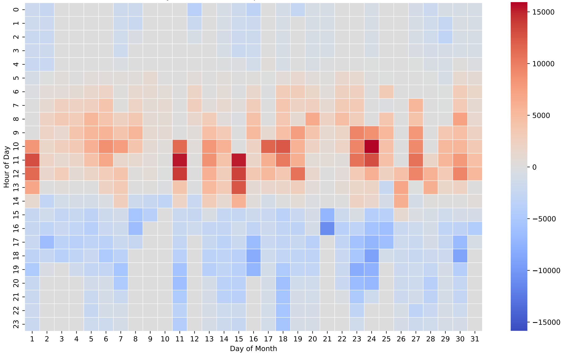
Battery Net Power Heatmap (Wh/Hour) - 50kWh - Mar
