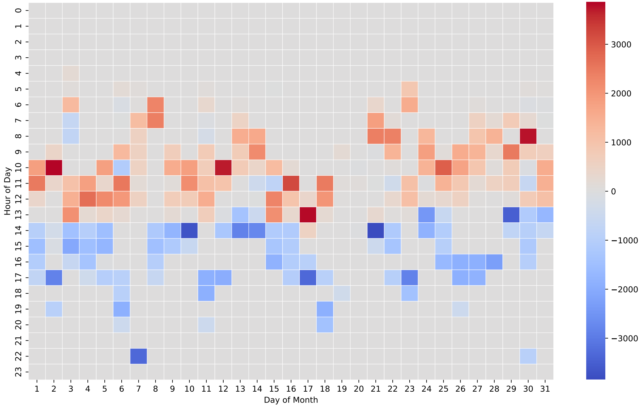
Battery Net Power Heatmap (Wh/Hour) - 5kWh - Oct
