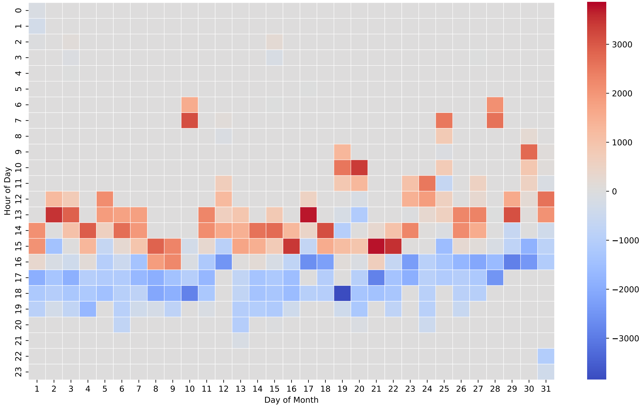
Battery Net Power Heatmap (Wh/Hour) - 5kWh - Aug
