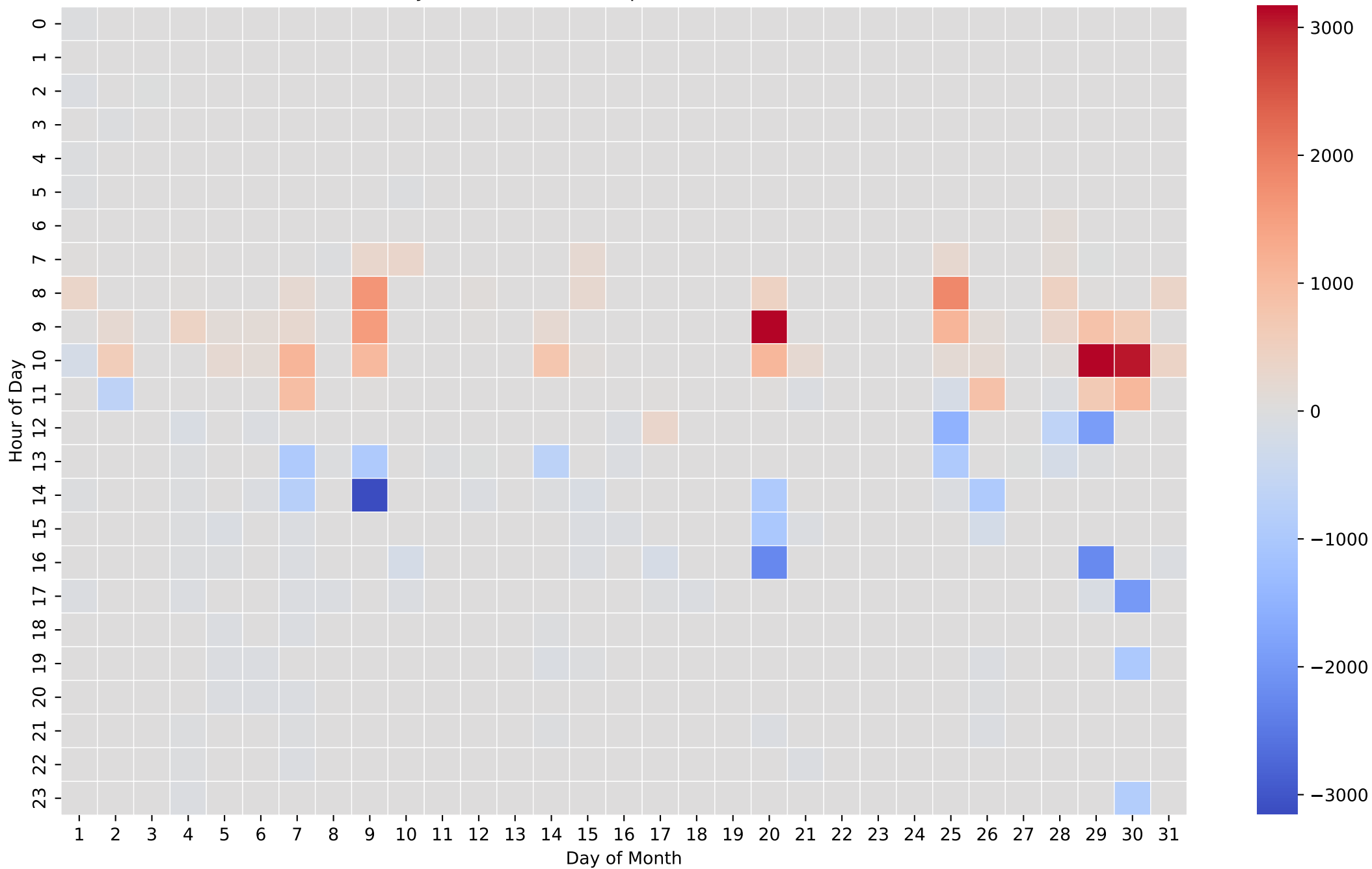
Battery Net Power Heatmap (Wh/Hour) - 5kWh - Dec
