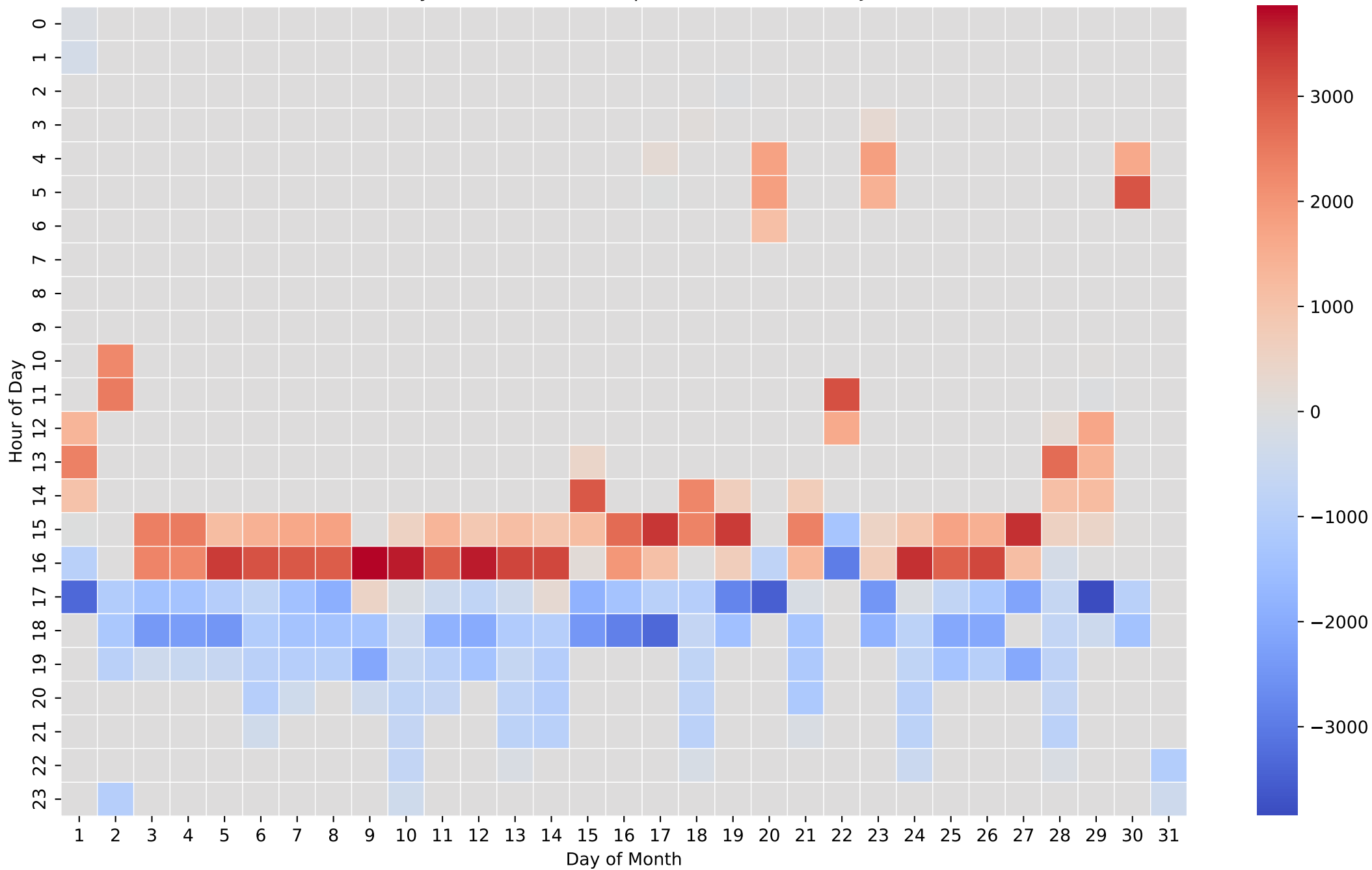
Battery Net Power Heatmap (Wh/Hour) - 5kWh - Jun
