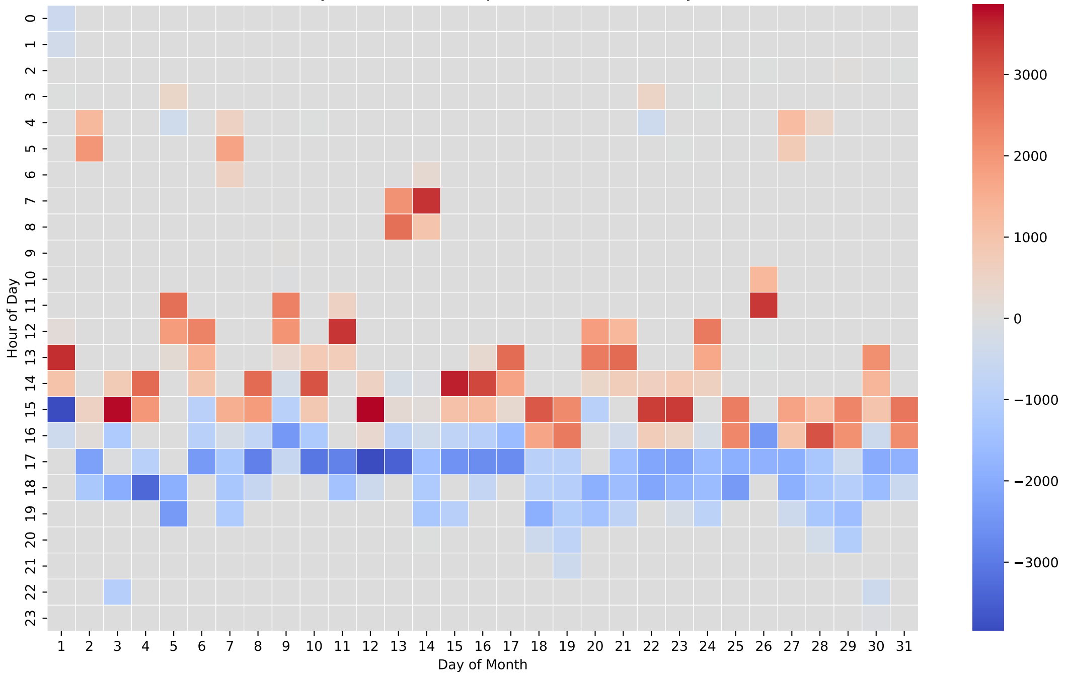
Battery Net Power Heatmap (Wh/Hour) - 5kWh - May
