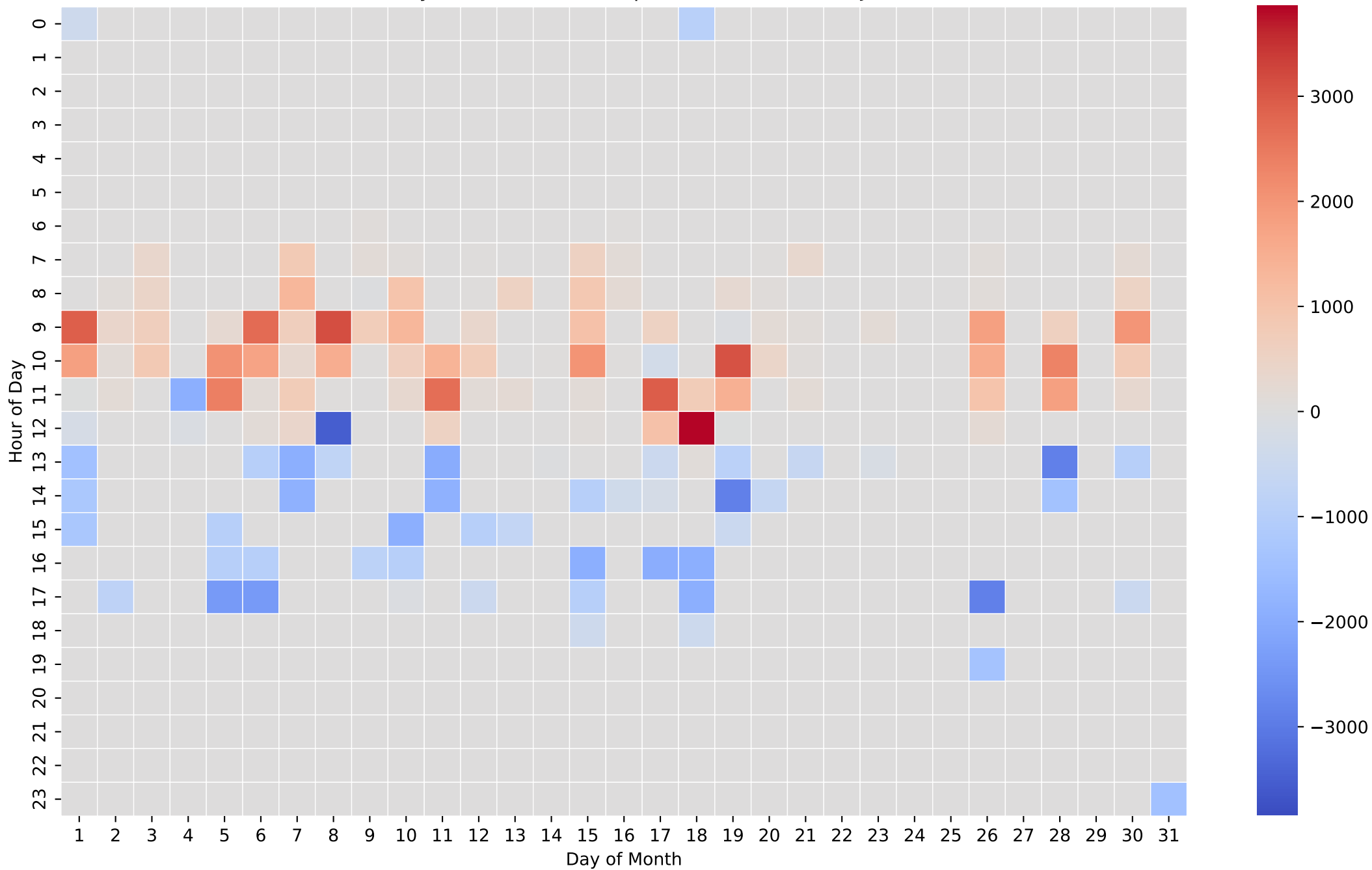
Battery Net Power Heatmap (Wh/Hour) - 5kWh - Jan
