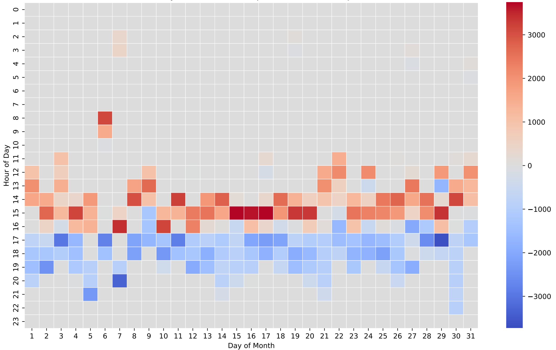
Battery Net Power Heatmap (Wh/Hour) - 5kWh - Jul
