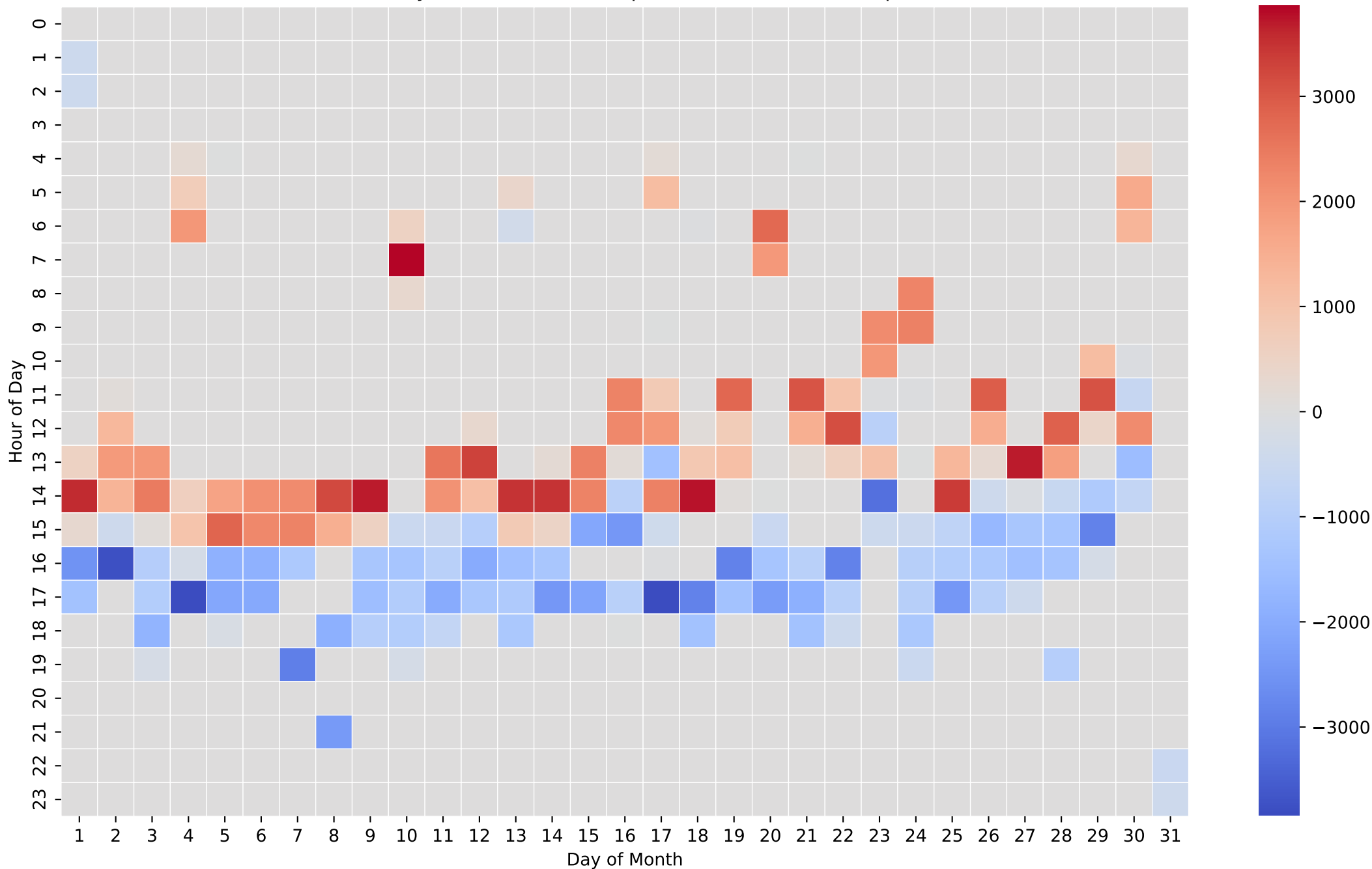
Battery Net Power Heatmap (Wh/Hour) - 5kWh - Sep
