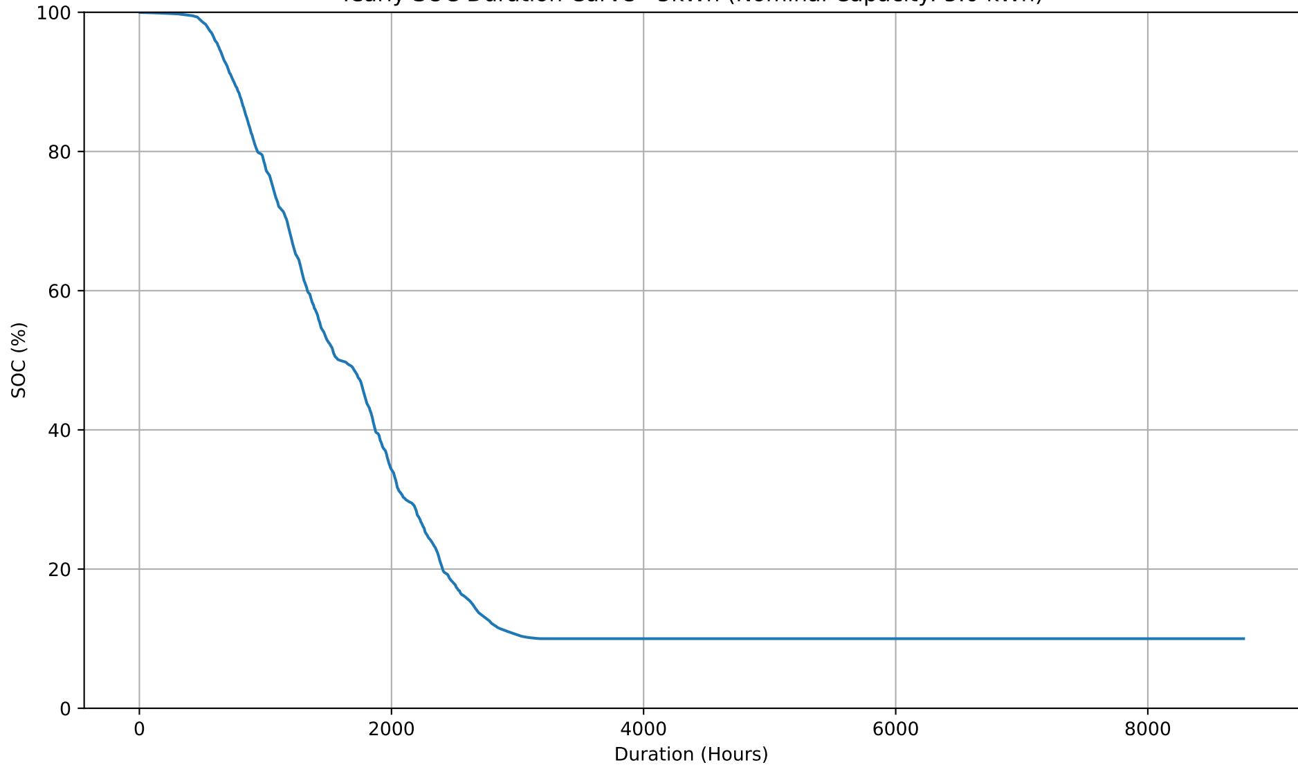
Yearly SOC Duration Curve - 5kWh (Nominal Capacity: 5.0 kWh)
