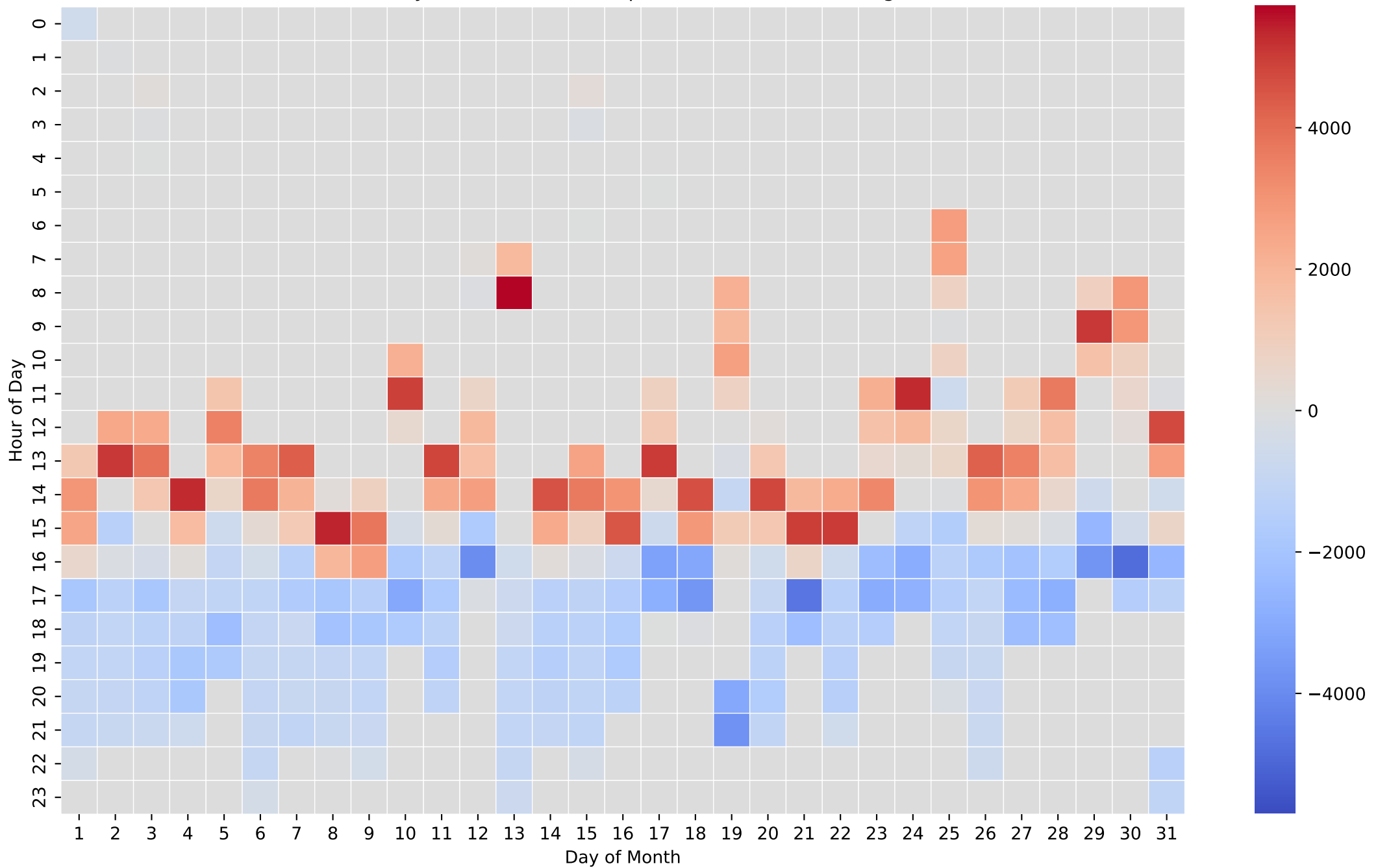
Battery Net Power Heatmap (Wh/Hour) - 8kWh - Aug
