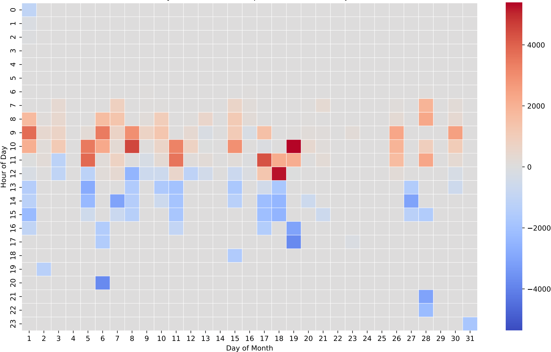
Battery Net Power Heatmap (Wh/Hour) - 8kWh - Jan
