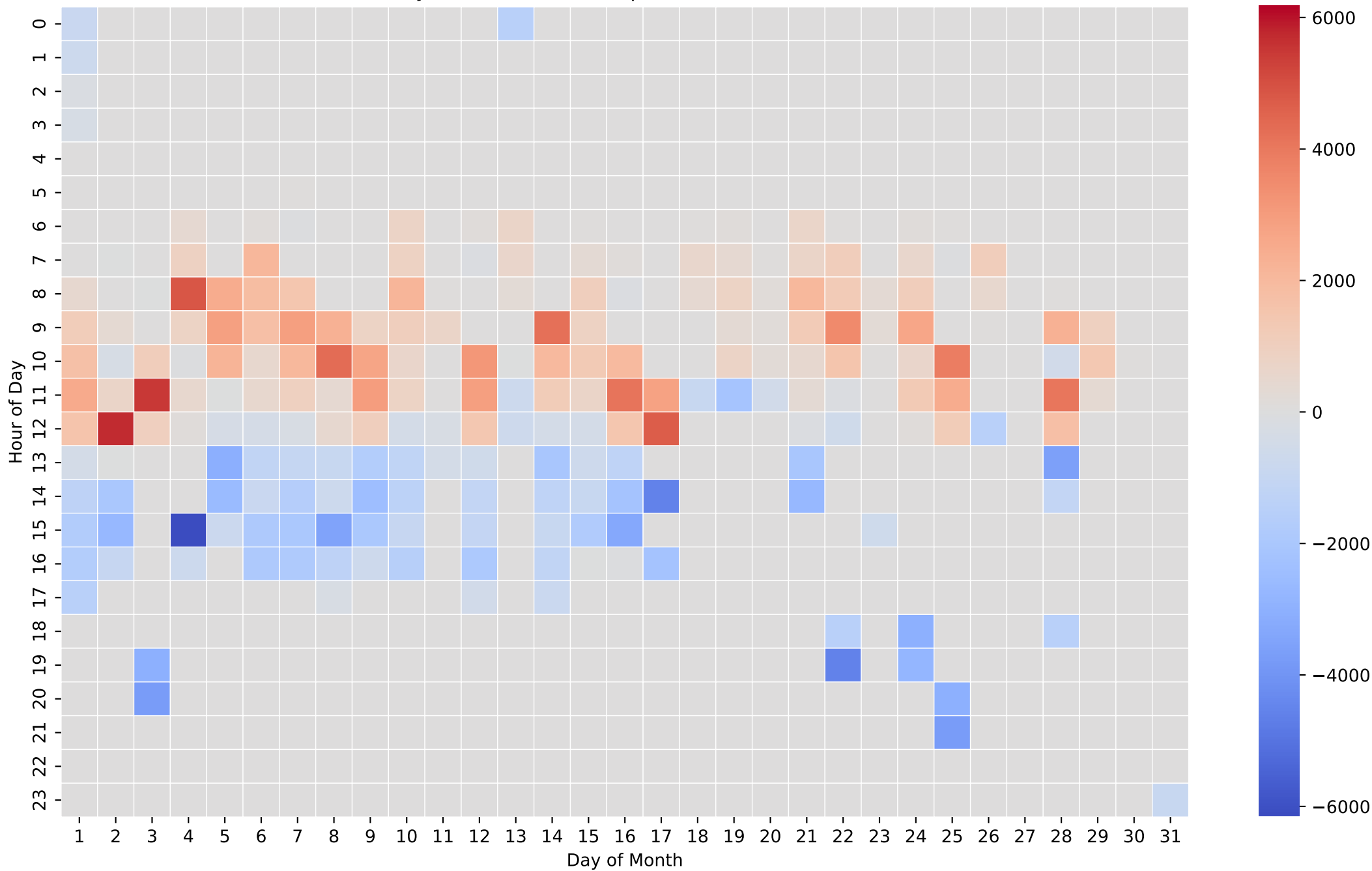
Battery Net Power Heatmap (Wh/Hour) - 8kWh - Nov
