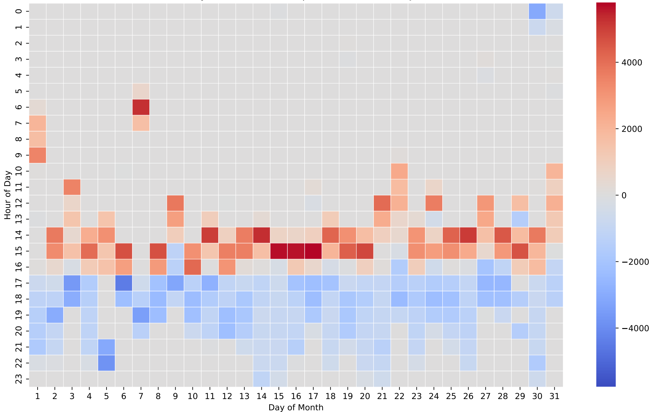
Battery Net Power Heatmap (Wh/Hour) - 8kWh - Jul
