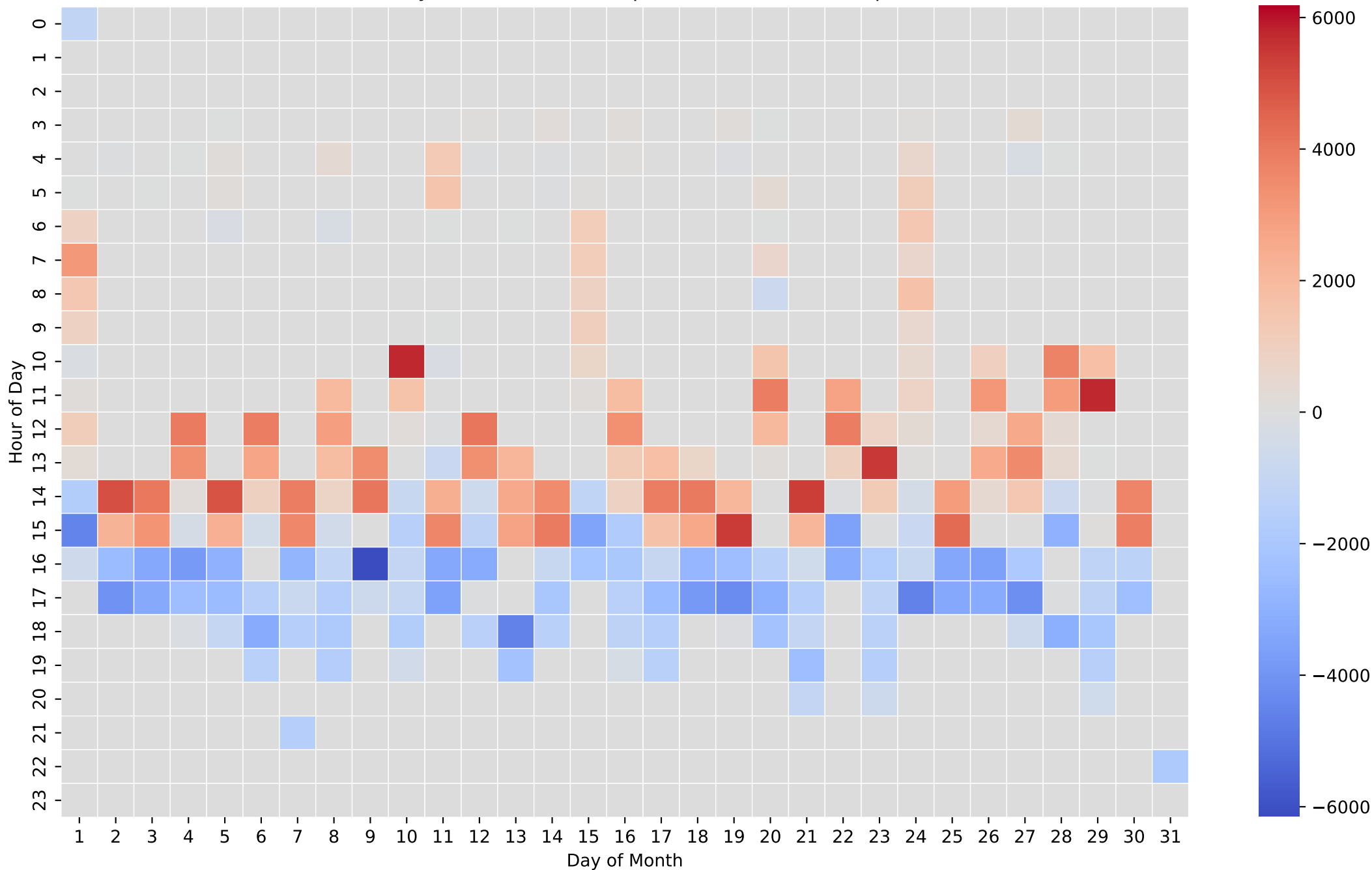
Battery Net Power Heatmap (Wh/Hour) - 8kWh - Apr
