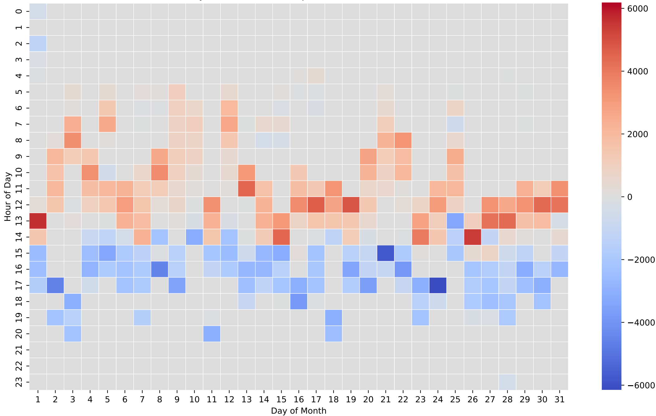
Battery Net Power Heatmap (Wh/Hour) - 8kWh - Mar
