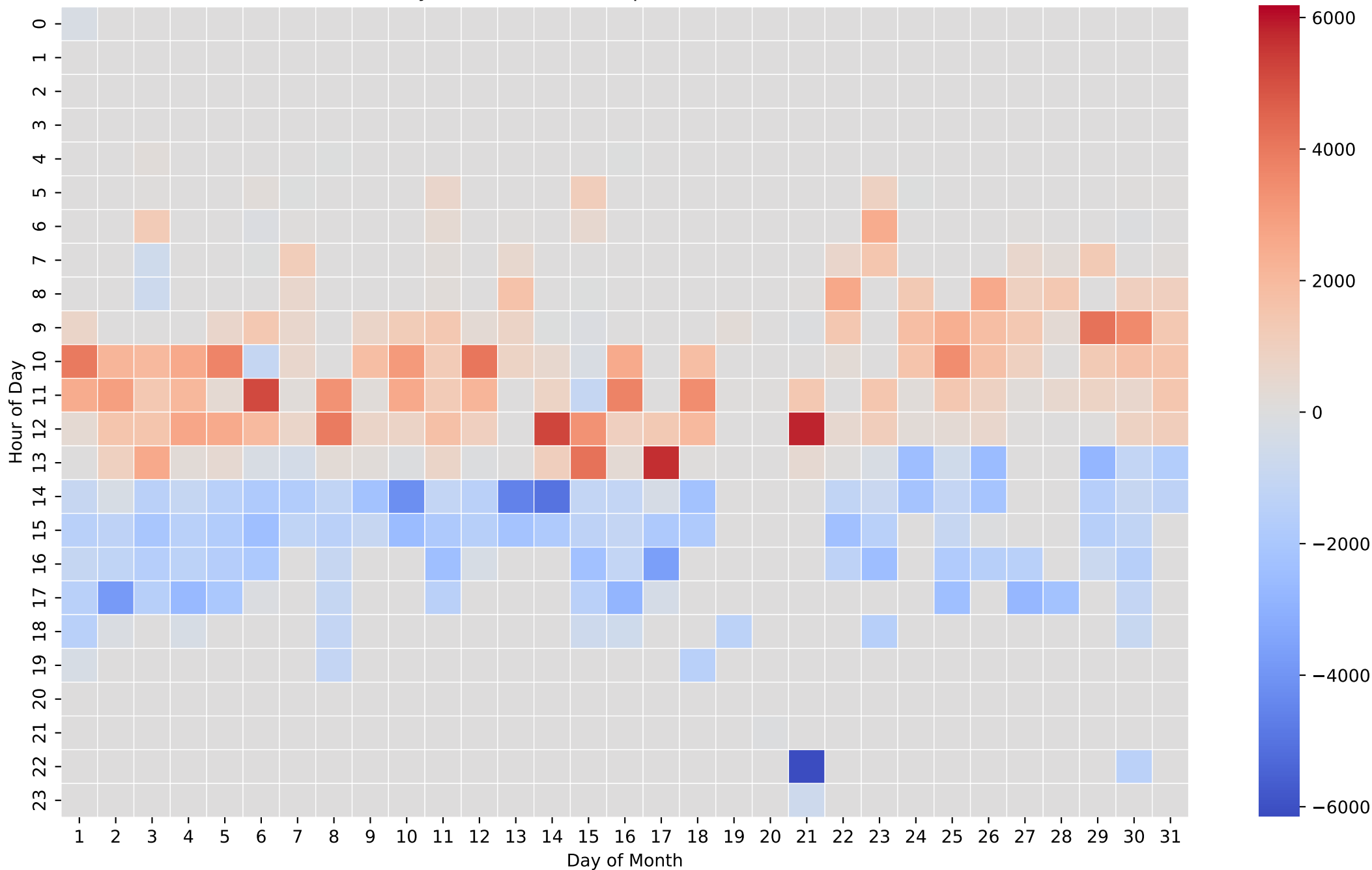
Battery Net Power Heatmap (Wh/Hour) - 8kWh - Oct
