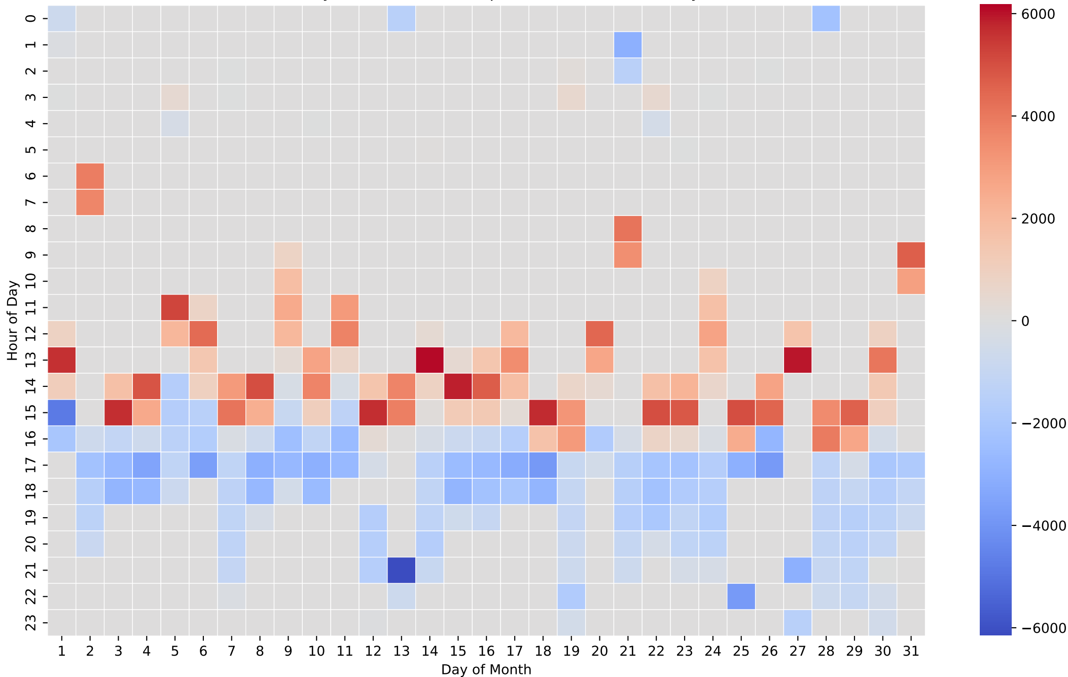
Battery Net Power Heatmap (Wh/Hour) - 8kWh - May
