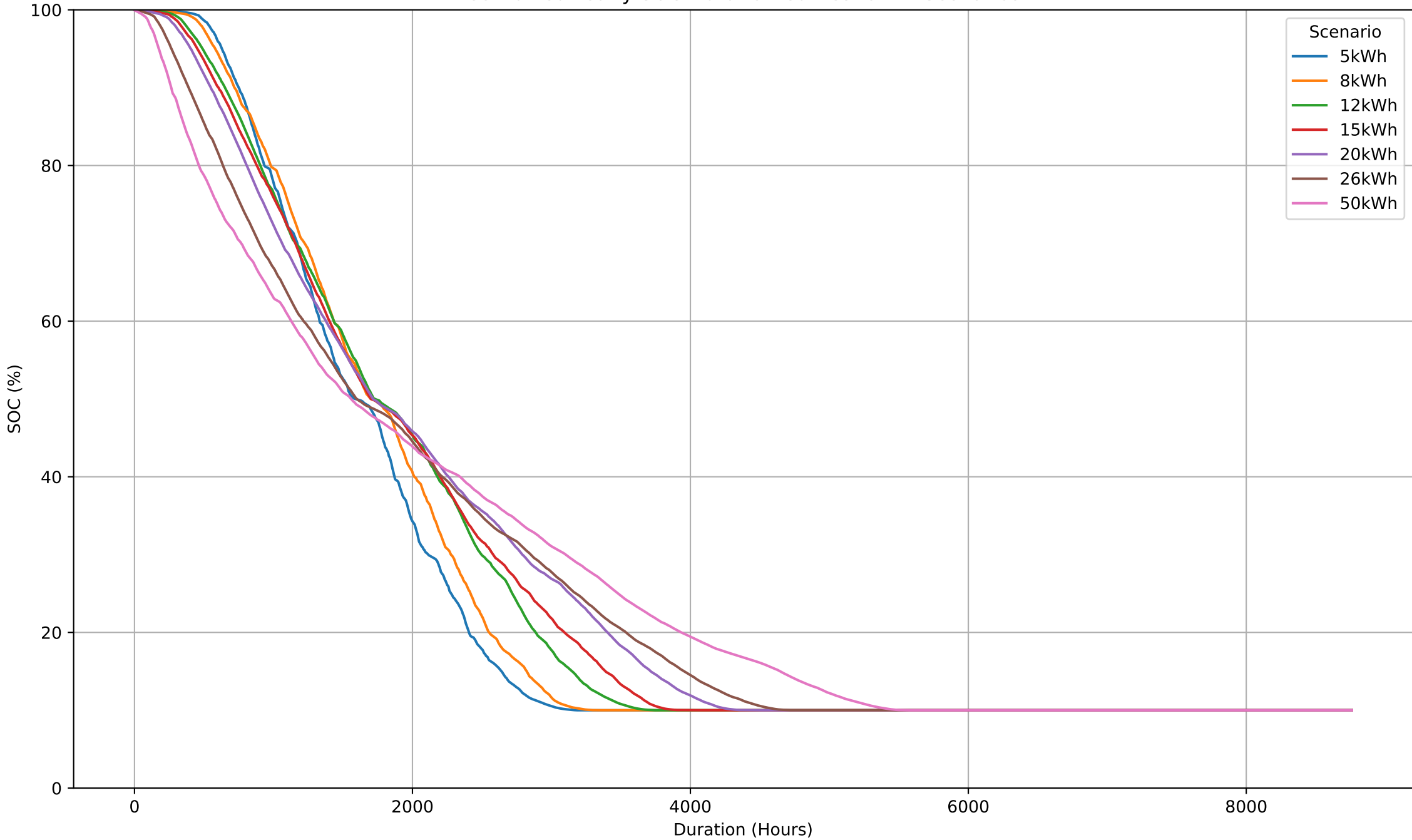
Combined Yearly SOC Duration Curves for All Scenarios
