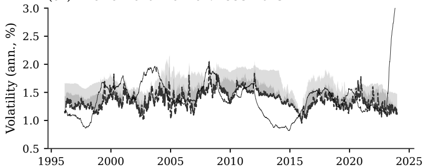
(c1) Twelve-month horizon: 1995-2023
