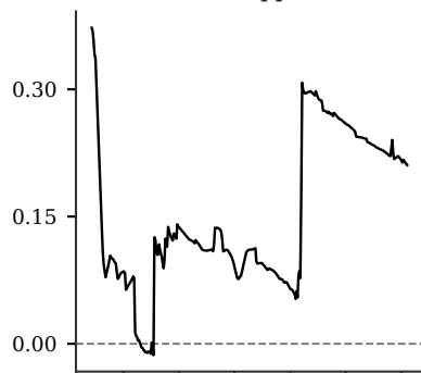
\tau = 0.95 (upper tail)
