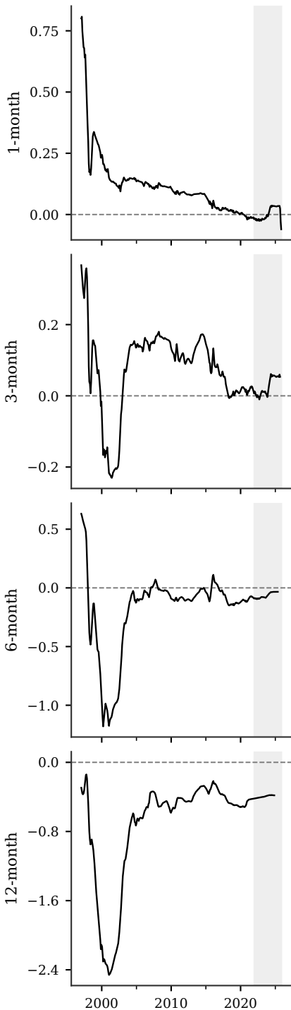
\tau = 0.50 (median)
