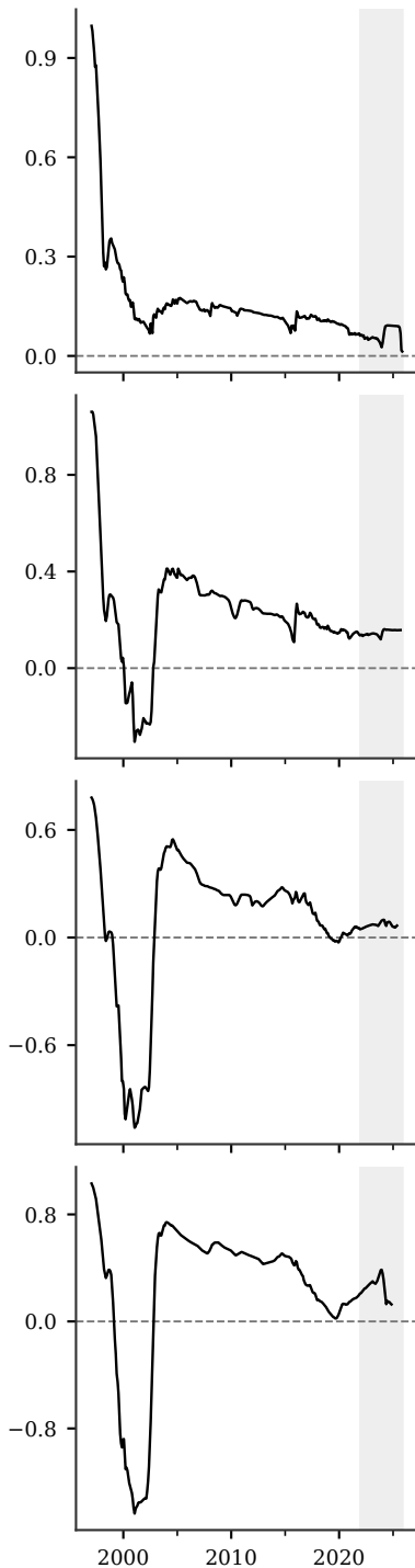
\tau = 0.75
