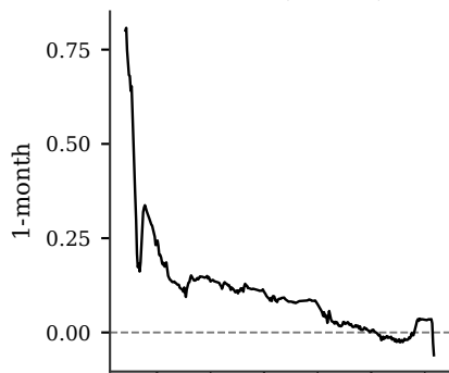
\tau = 0.50 (median)
