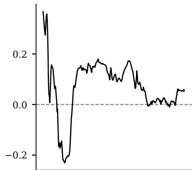
3-month
