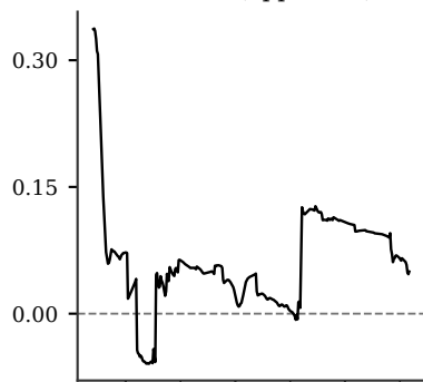
\tau = 0.95 (upper tail)
