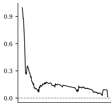
\tau = 0.75
