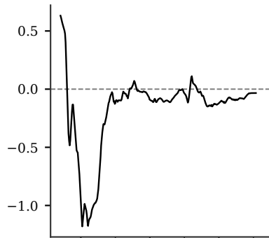
6-month
