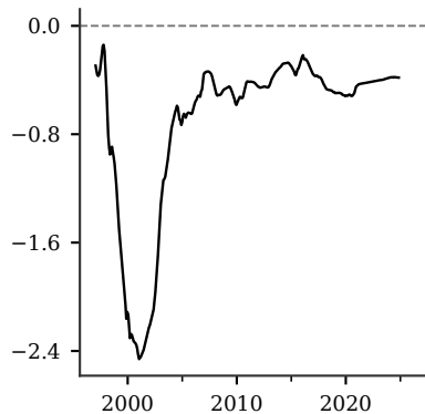
12-month
