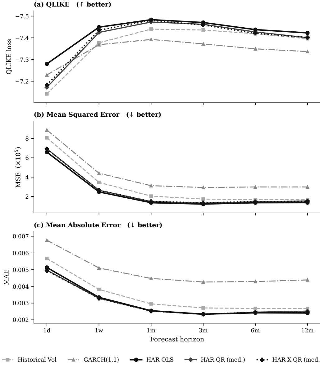
Figure 6: Robustness check: point forecast accuracy under three loss functions. Each panel plots mean (or median) forecast loss across horizons. QLIKE axis is inverted (more negative = better). MSE scaled by 10^5 for readability. The consistent separation between GARCH(1,1) and the HAR family at long horizons holds across all three metrics.
