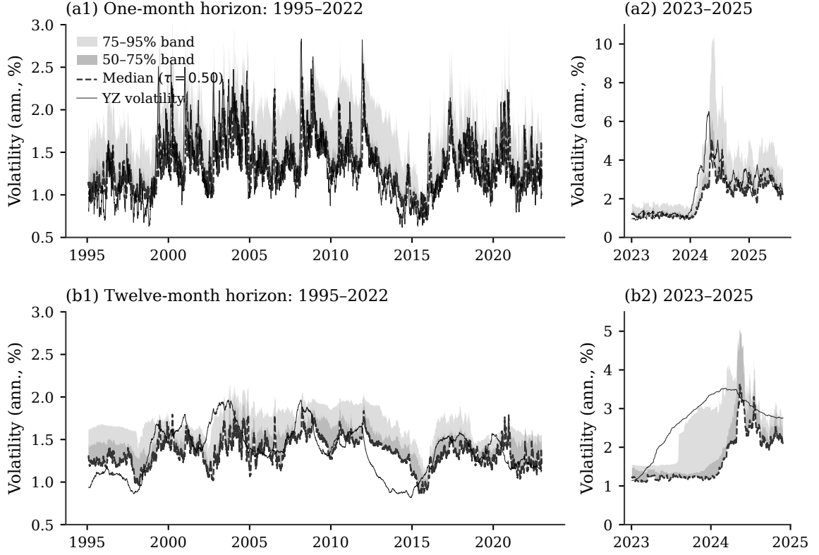
Figure 7: HAR-X-QR distributional forecasts: quantile bands and Yang-Zhang volatility
