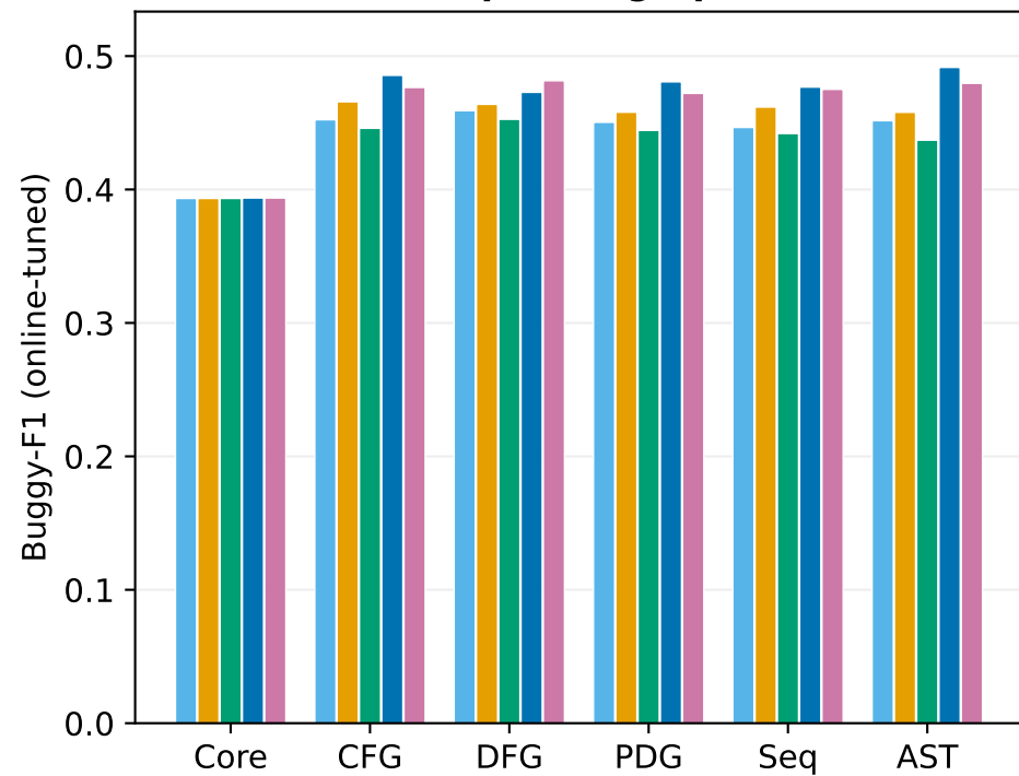
scope: subgraph
