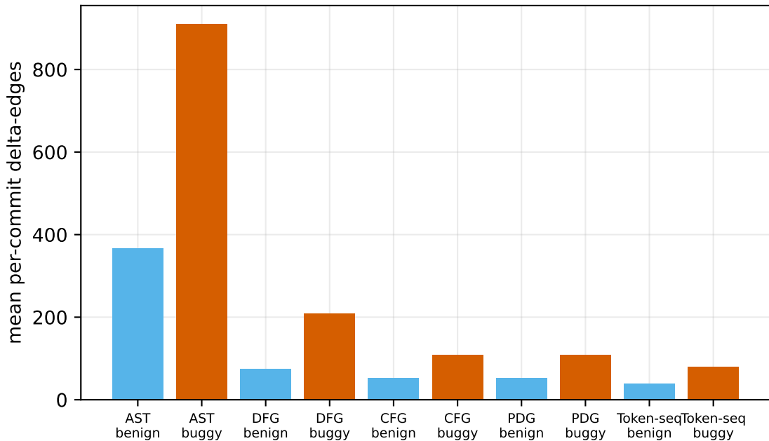
Change size: buggy vs benign (all significant, MW p \ll 0.001 )
