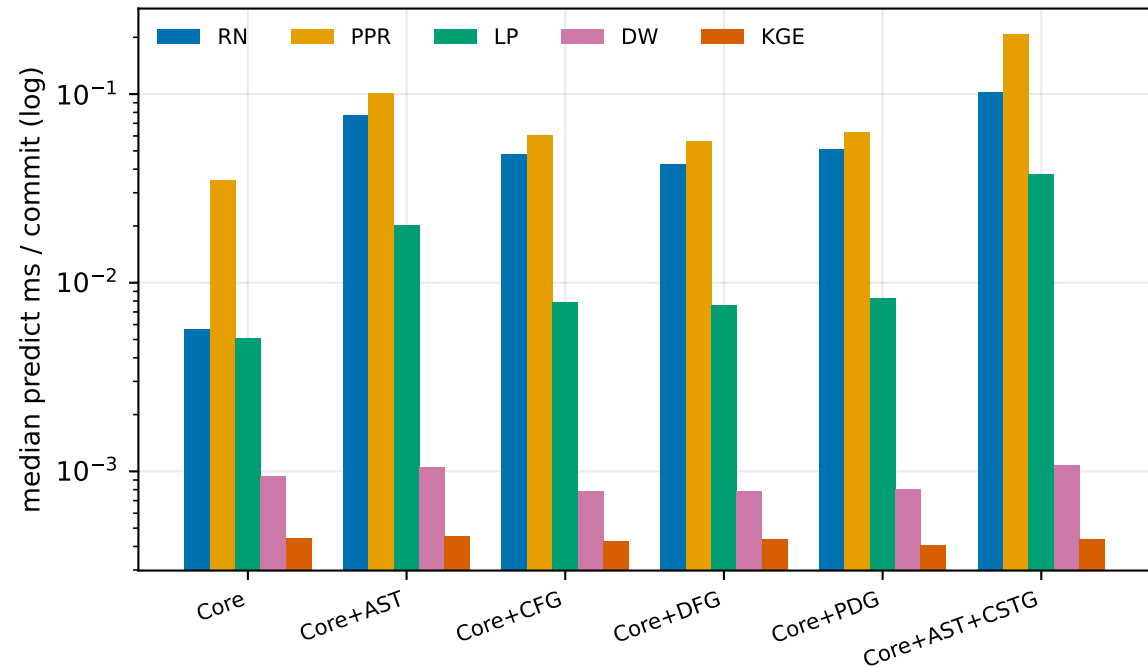
Prediction latency by method and graph richness
