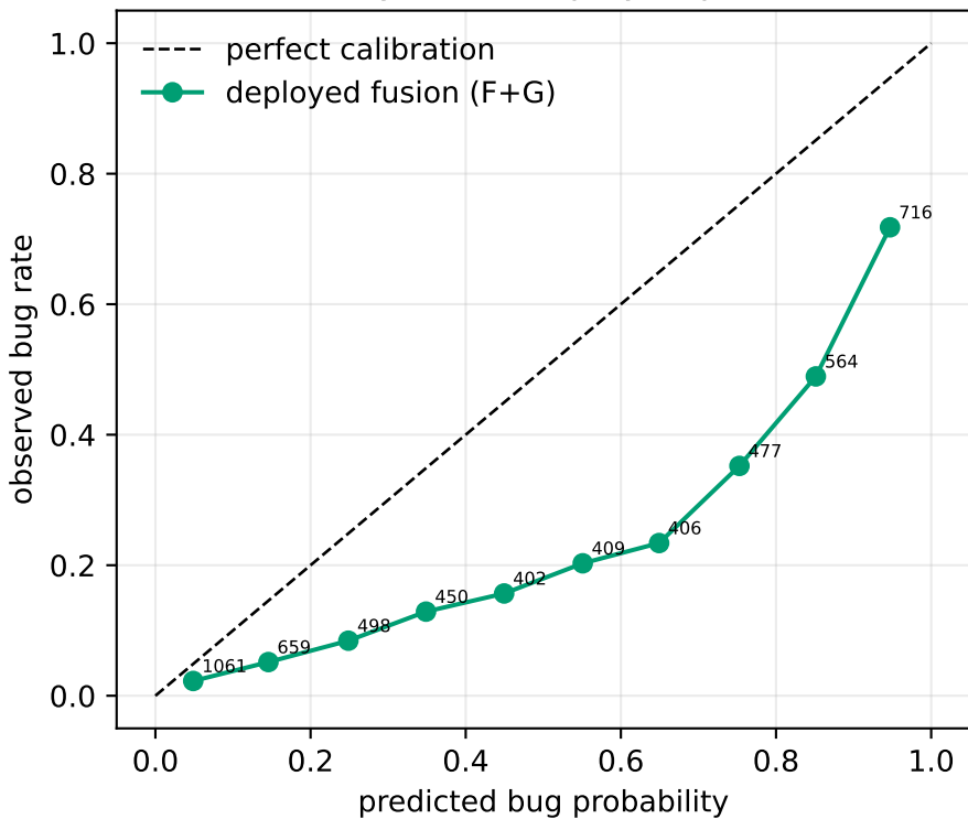
Reliability of the deployed predictor
