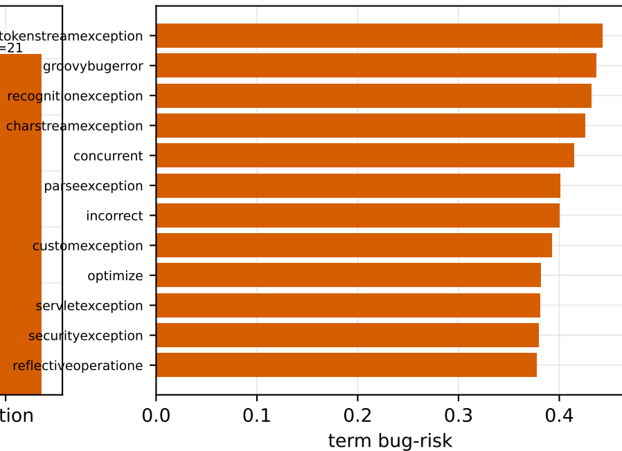
Highest-risk semantic terms
