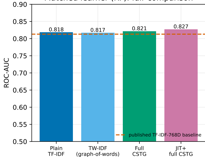
Matched learner (RF): fair comparison
