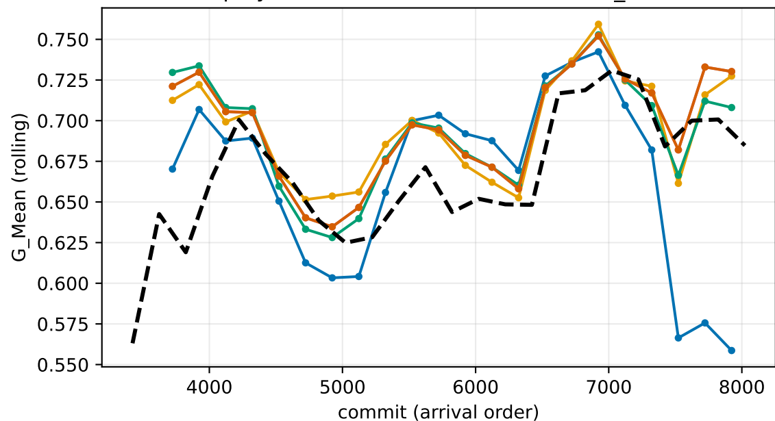
Deployed fusion F+G online stream: G_Mean
