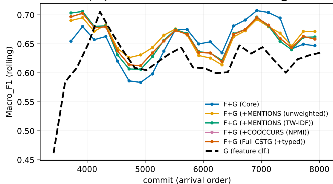
Deployed fusion F+G online stream: Macro_F1
