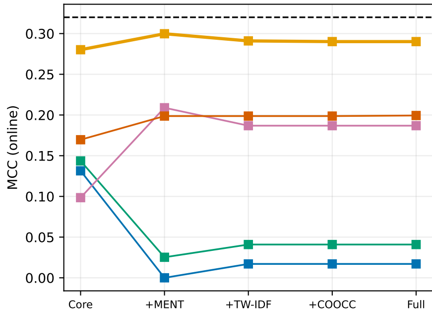
MCC as the CSTG graph is enriched
