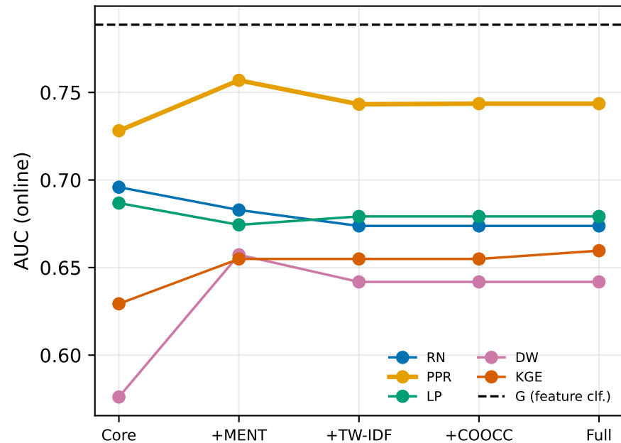
AUC as the CSTG graph is enriched
