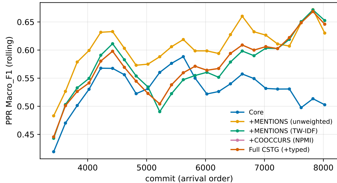
PPR online stream: Macro_F1 across CSTG layers
