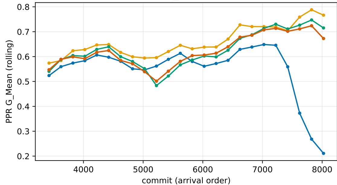
PPR online stream: G_Mean across CSTG layers
