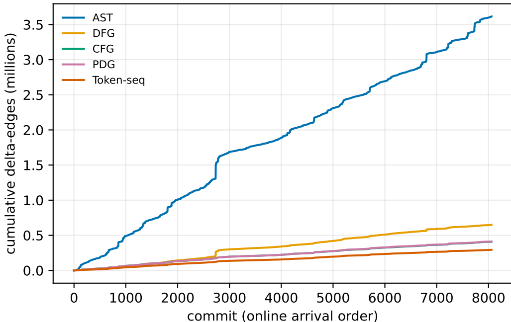
Online KG growth per structural layer
