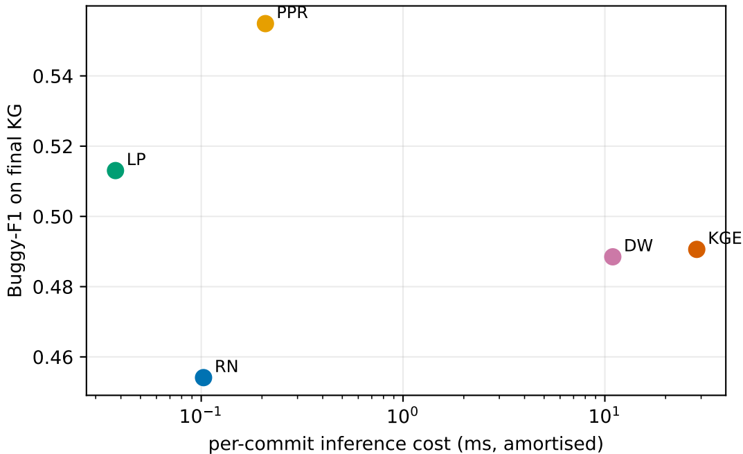
Cost vs accuracy on the deployed graph (Pareto)
