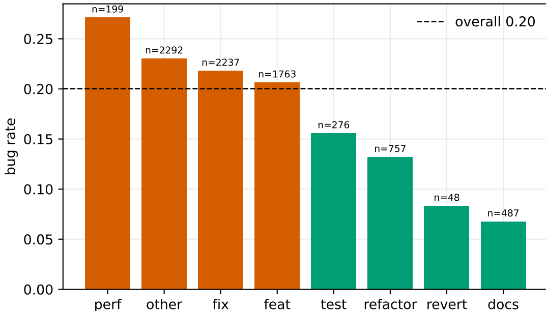
Bug rate by change-intent (CSTG typing)
