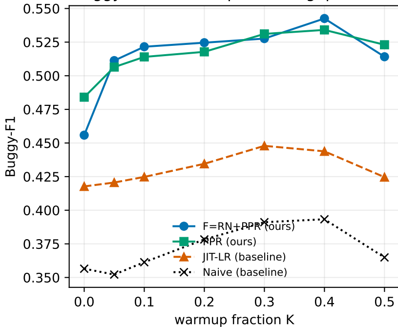
Buggy-F1 vs warmup at fixed gap M=200
