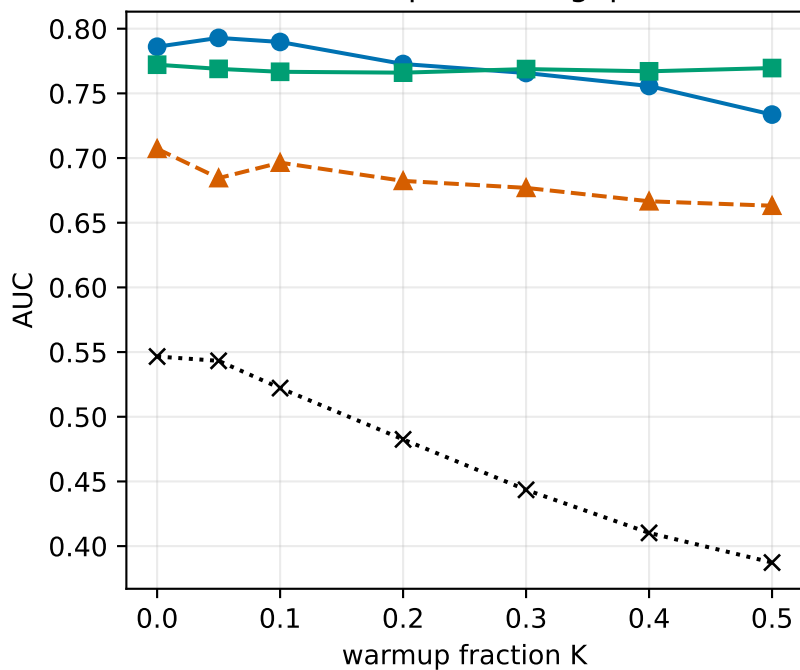
AUC vs warmup at fixed gap M=200
