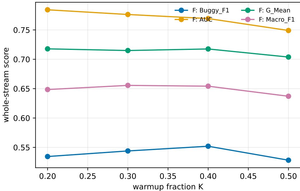
Deployed fusion F vs warmup fraction K
