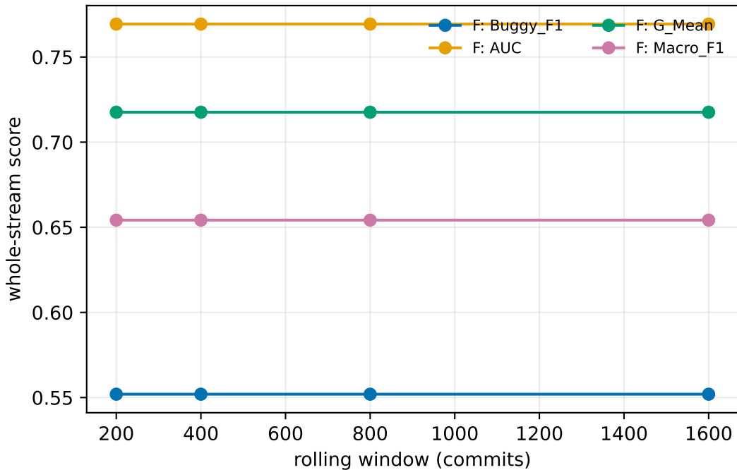
Deployed fusion F vs rolling window (commits)
