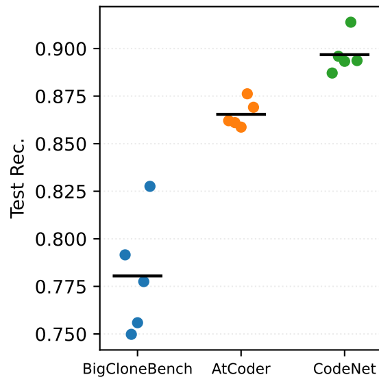
SPECTRA-Siam across independent seeds (5-5 per benchmark; black bar = mean)
