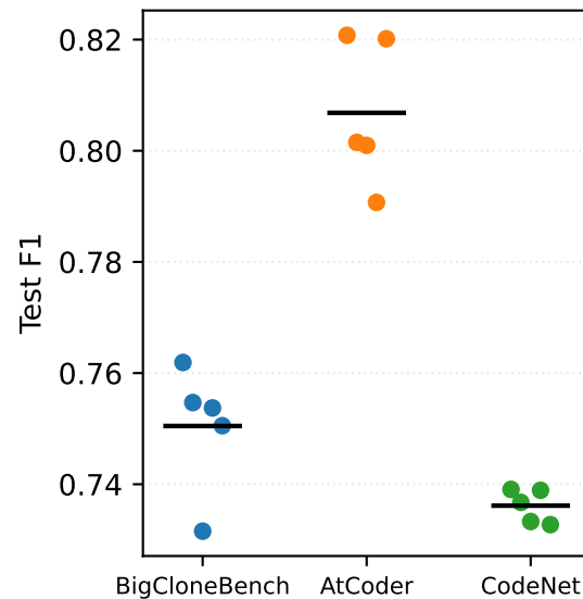
SPECTRA-Siam across independent seeds (5-5 per benchmark; black bar = mean)
