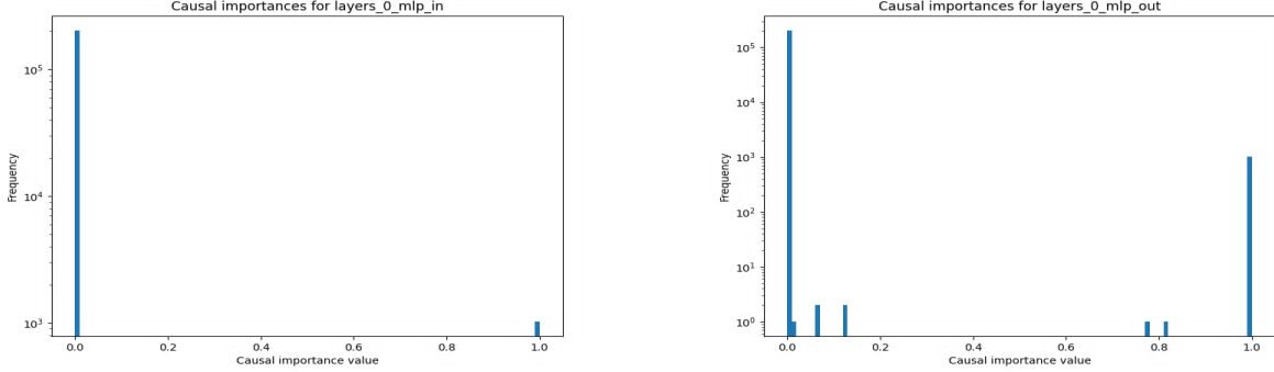
Figure 9: Distributions of causal importance values for the softmax decomposition on both layers.
