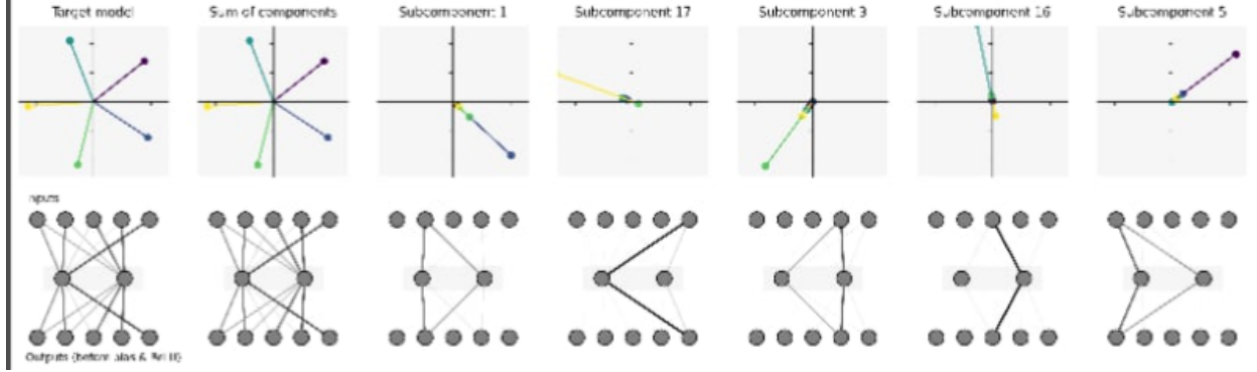
Figure 1: Decomposition of \text{TMS}_{5-2} . The first two panels show the target model’s weight columns and the sum of learned subcomponents. Subsequent panels show the individual subcomponents, ordered by decreasing norm. Although 20 subcomponents are allocated, only the first 5 carry meaningful norm and contribute to reconstruction, while the remaining 15 have negligible weight and are effectively pruned by the method. Each active subcomponent recovers primarily one feature direction, with minor leakage across components.
