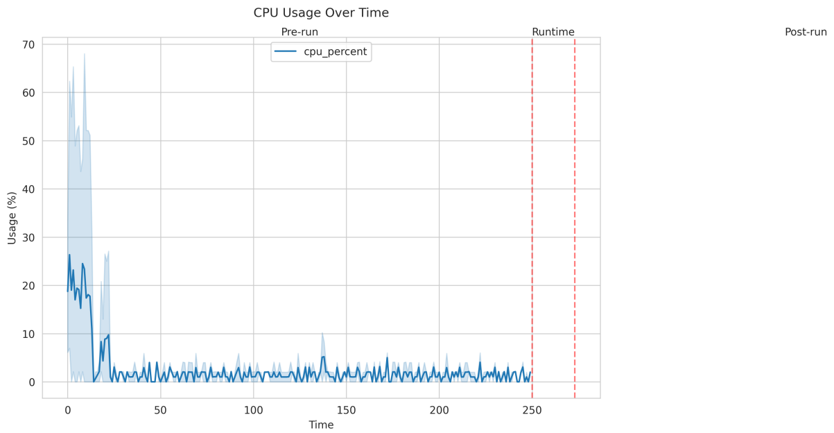
Figure 3: CPU Usage Analysis
