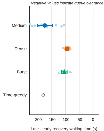
(b) Recovery queue clearance
